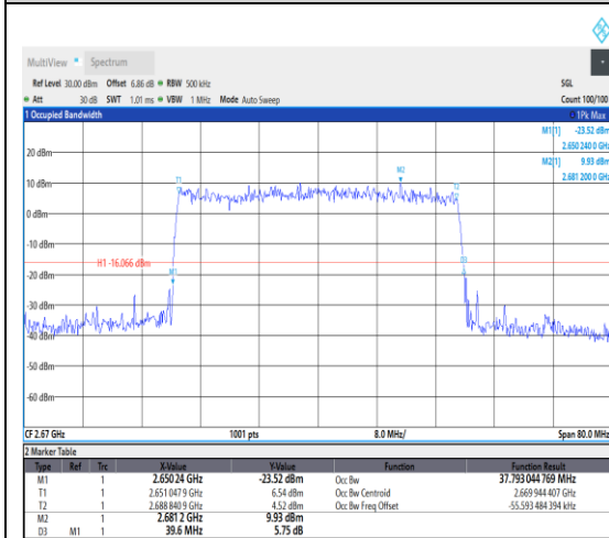
1-N41--30-40-H-9-CP-256QAM-Outer_Full-1 06@0-Ant1-37.793-39.600-≤40-PASS
