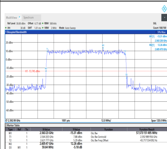
1-N41--30-60-M-3-DFT-16QAM-Outer_Full-1 62@0-Ant1-57.573-59.640-≤60-PASS
