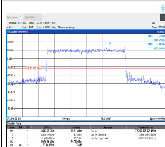
1-N41--30-80-H-8-CP-64QAM-Outer_Full-21 7@0-Ant1-77.294-80.640-≤80-PASS
