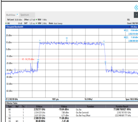
1-N41--30-80-M-5-DFT-256QAM-Outer_Full- 216@0-Ant1-77.069-80.480-≤80-PASS
