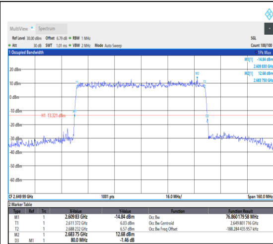
1-N41--30-80-H-5-DFT-256QAM-Outer_Full- 216@0-Ant1-76.86-80.000-≤80-PASS
