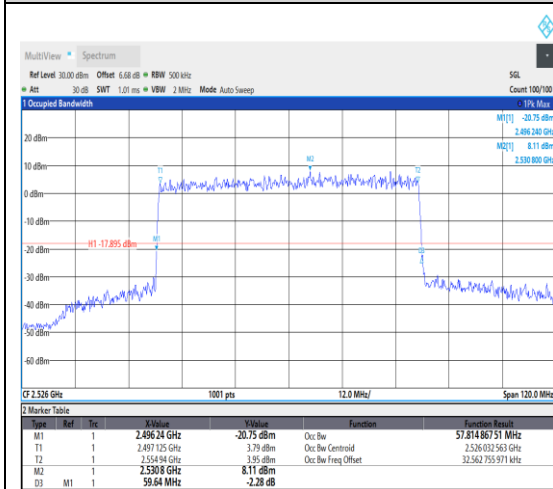
1-N41--30-60-L-9-CP-256QAM-Outer_Full-16 2@0-Ant1-57.815-59.640-≤60-PASS
