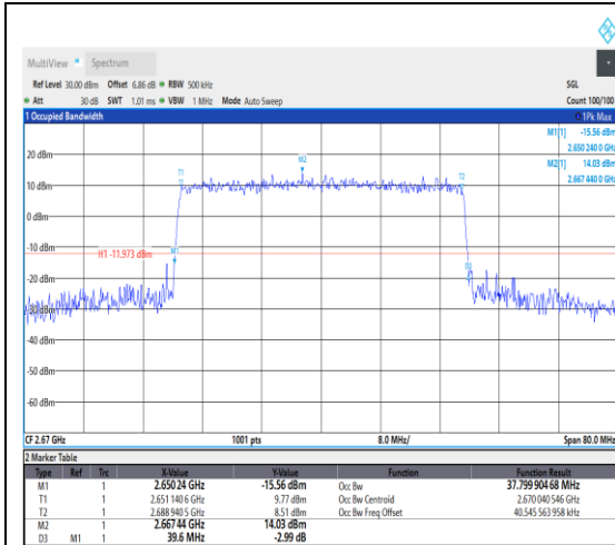
1-N41--30-40-H-7-CP-16QAM-Outer_Full-10 6@0-Ant1-37.8-39.600-≤40-PASS
