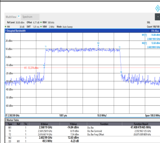
1-N41--30-50-M-6-CP-QPSK-Outer_Full-133 @0-Ant1-47.408-49.500-≤50-PASS
