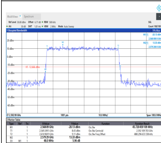
1-N41--30-50-M-3-DFT-16QAM-Outer_Full-1 28@0-Ant1-45.72-48.000-≤50-PASS
