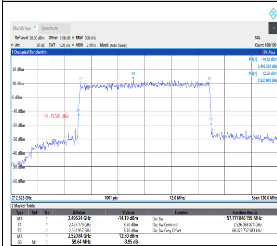
1-N41--30-60-L-3-DFT-16QAM-Outter_Full-16 2@0-Ant1-57.778-59.640-≤60-PASS
