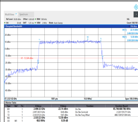
1-N41--30-50-L-3-DFT-16QAM-Outer_Full-12 8@0-Ant1-45.747-48.000-≤50-PASS
