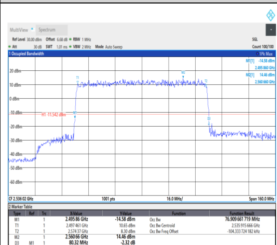
1-N41--30-80-L-3-DFT-16QAM-Outer_Full-21 6@0-Ant1-76.91-80.320-≤80-PASS
