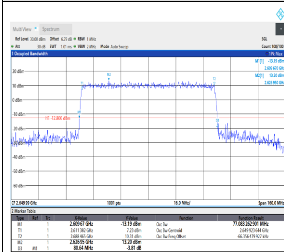
1-N41--30-80-H-6-CP-QPSK-Outer_Full-217 @0-Ant1-77.083-80.640-≤80-PASS
