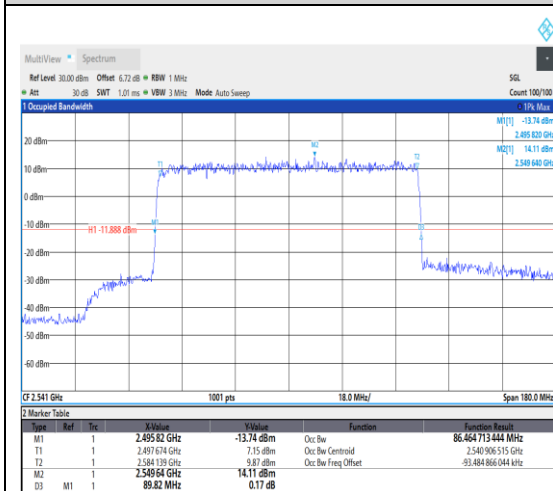
1-N41--30-90-L-3-DFT-16QAM-Outer_Full-243@0-Ant1-86.465-89.820-≤90-PASS
