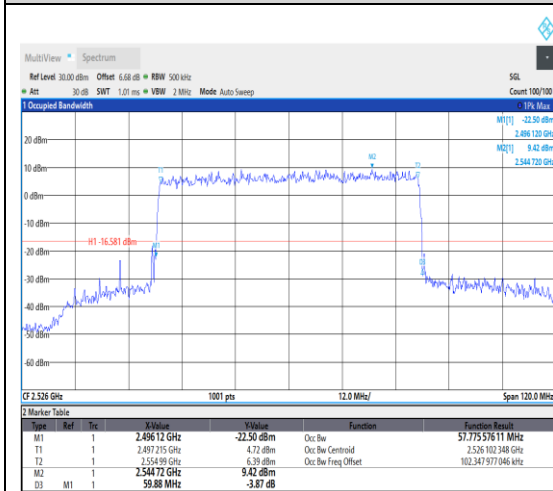
1-N41--30-60-L-5-DFT-256QAM-Outter_Full-1 62@0-Ant1-57.776-59.880-≤60-PASS
