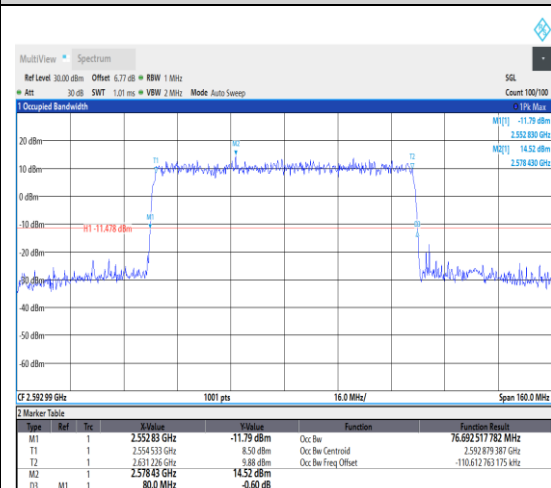
1-N41--30-80-M-4-DFT-64QAM-Outer_Full-2 16@0-Ant1-76.693-80.000-≤80-PASS
