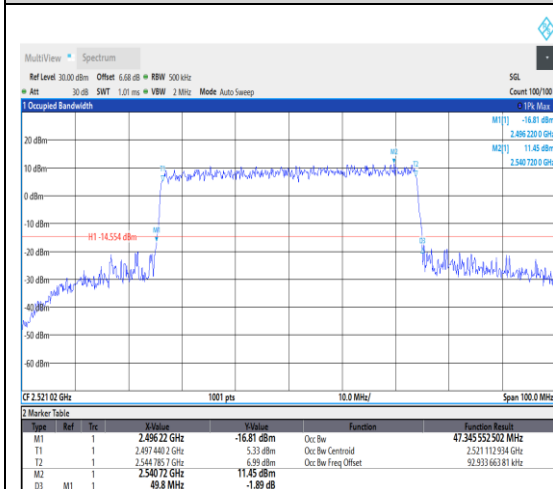
1-N41--30-50-L-8-CP-64QAM-Outer_Full-133 @0-Ant1-47.346-49.800-≤50-PASS
