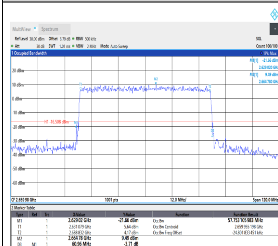
1-N41--30-60-H-5-DFT-256QAM-Outer_Full-162@0-Ant1-57.753-60.960-≤60-PASS
