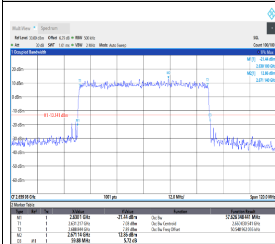
1-N41--30-60-H-3-DFT-16QAM-Outer_Full-1 62@0-Ant1-57.626-59.880-≤60-PASS
