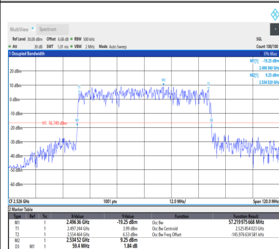
1-N41--30-60-L-6-CP-QPSK-Outter_Full-162 @0-Ant1-57.22-59.400-≤60-PASS
