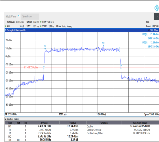
1-N41--30-60-L-4-DFT-64QAM-Outter_Full-16 2@0-Ant1-57.724-59.760-≤60-PASS
