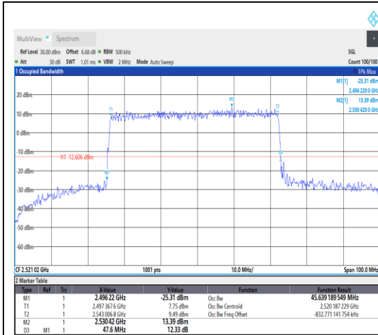
1-N41--30-50-L-4-DFT-64QAM-Outer_Full-12 8@0-Ant1-45.639-47.600-≤50-PASS
