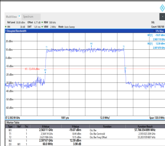
1-N41--30-60-M-1-DFT-QPSK-Outer_Full-16 2@0-Ant1-57.766-60.000-≤60-PASS
