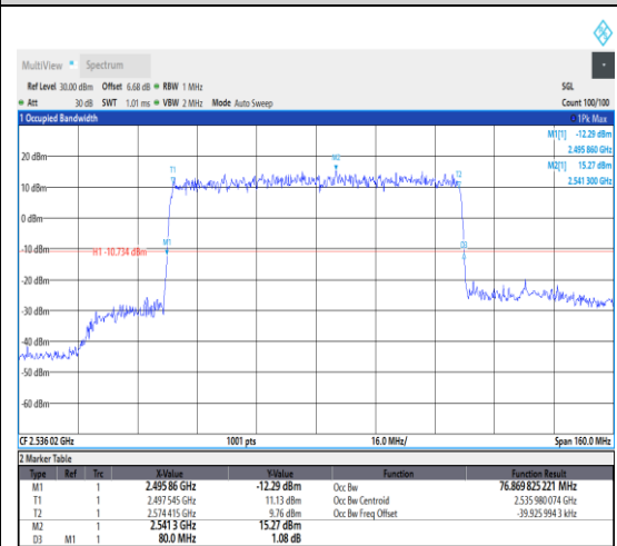
1-N41--30-80-L-1-DFT-QPSK-Outer_Full-216 @0-Ant1-76.87-80.000-≤80-PASS
