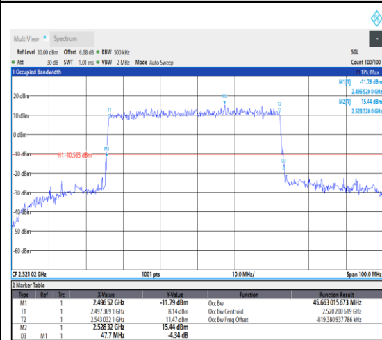
1-N41--30-50-L-1-DFT-QPSK-Outer_Full-128 @0-Ant1-45.663-47.700-≤50-PASS
