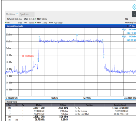
1-N41--30-60-M-2-DFT-PI2BPSK-Outer_Full- 162@0-Ant1-57.91-59.760-≤60-PASS
