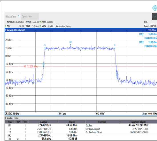
1-N41--30-50-M-4-DFT-64QAM-Outer_Full-1 28@0-Ant1-45.672-47.900-≤50-PASS
