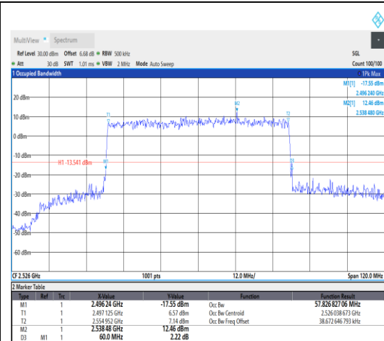
1-N41--30-60-L-8-CP-64QAM-Outer_Full-162 @0-Ant1-57.827-60.000-≤60-PASS
