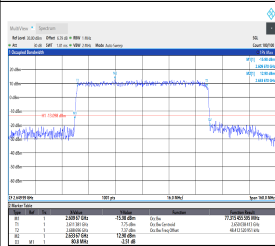
1-N41--30-80-H-7-CP-16QAM-Outer_Full-21 7@0-Ant1-77.315-80.800-≤80-PASS
