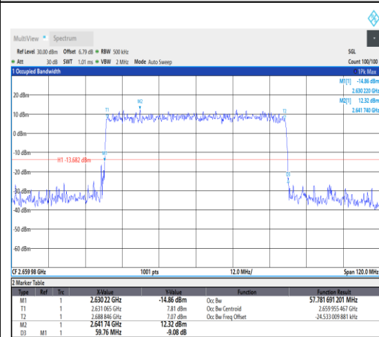
1-N41--30-60-H-4-DFT-64QAM-Outer_Full-1 62@0-Ant1-57.782-59.760-≤60-PASS
