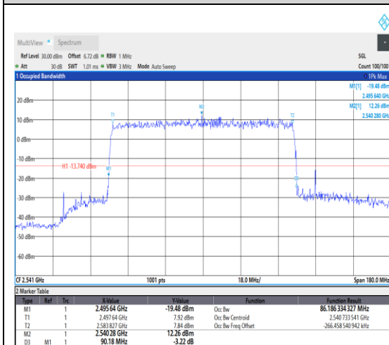
1-N41--30-90-L-5-DFT-256QAM-Outer_Full-243@0-Ant1-86.186-90.180-≤90-PASS
