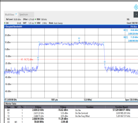
1-N41--30-60-H-6-CP-QPSK-Outer_Full-162 @0-Ant1-57.53-59.640-≤60-PASS
