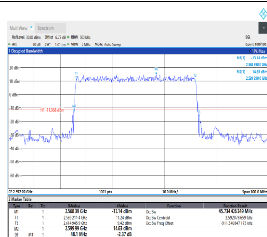
1-N41--30-50-M-2-DFT-PI2BPSK-Outer_Full-128@0-Ant1-45.734-48.100-≤50-PASS
