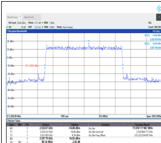
1-N41--30-80-M-1-DFT-QPSK-Outer_Full-21 6@0-Ant1-77.076-80.160-≤80-PASS
