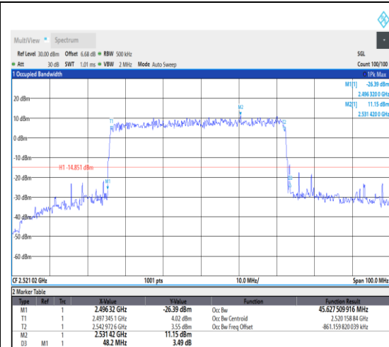
1-N41--30-50-L-5-DFT-256QAM-Outer_Full-1 28@0-Ant1-45.628-48.200-≤50-PASS
