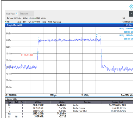
1-N41--30-60-H-1-DFT-QPSK-Outer_Full-16 2@0-Ant1-57.722-59.640-≤60-PASS
