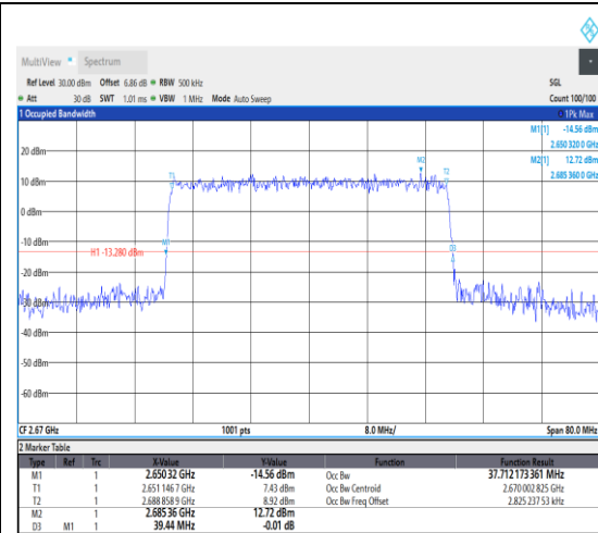
1-N41--30-40-H-8-CP-64QAM-Outer_Full-10 6@0-Ant1-37.712-39.440-≤40-PASS
