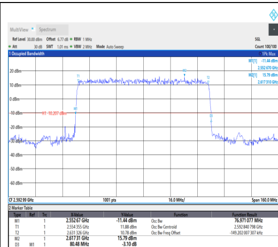
1-N41--30-80-M-2-DFT-PI2BPSK-Outer_Full- 216@0-Ant1-76.971-80.480-≤80-PASS
