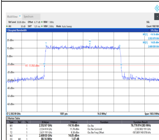
1-N41--30-80-M-3-DFT-16QAM-Outer_Full-2 16@0-Ant1-76.777-80.160-≤80-PASS
