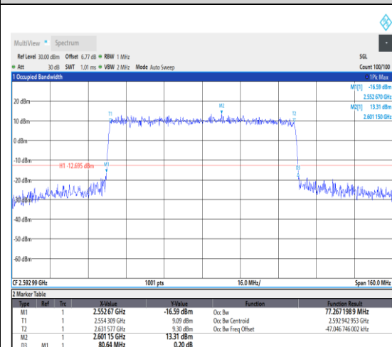
1-N41--30-80-M-6-CP-QPSK-Outer_Full-217 @0-Ant1-77.267-80.640-≤80-PASS
