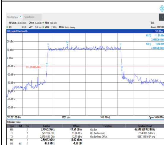
1-N41--30-50-L-2-DFT-PI2BPSK-Outer_Full-128@0-Ant1-45.649-47.300-≤50-PASS
