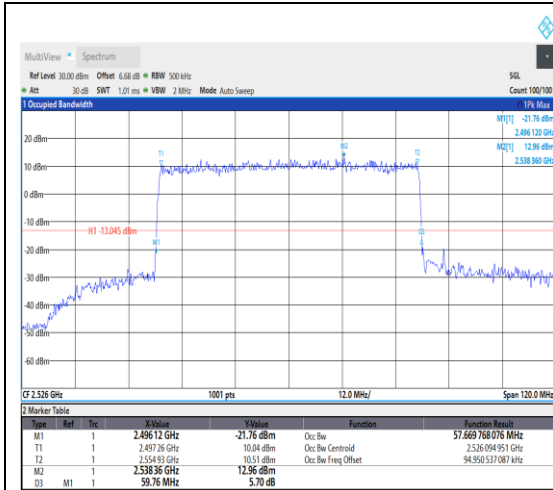
1-N41--30-60-L-1-DFT-QPSK-Outter_Full-162 @0-Ant1-57.67-59.760-≤60-PASS
