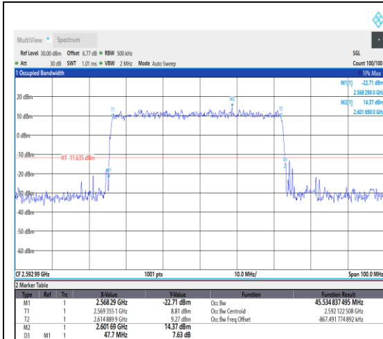
1-N41--30-50-M-1-DFT-QPSK-Outer_Full-12 8@0-Ant1-45.535-47.700-≤50-PASS
