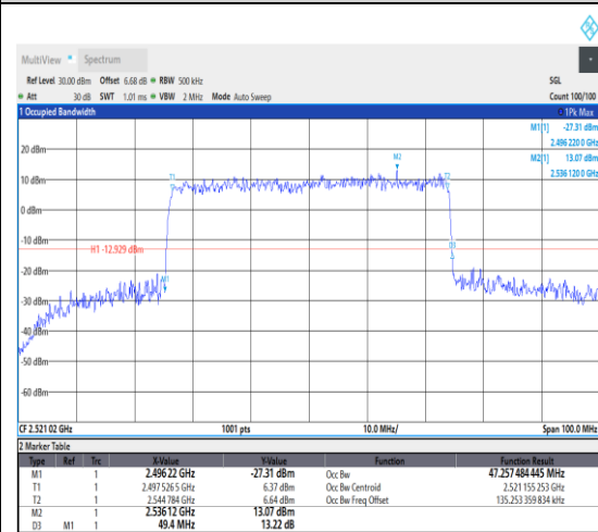
1-N41--30-50-L-7-CP-16QAM-Outer_Full-133 @0-Ant1-47.257-49.400-≤50-PASS
