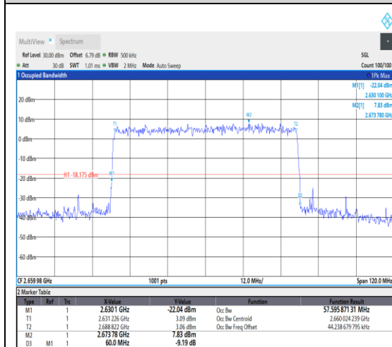
1-N41--30-60-H-9-CP-256QAM-Outer_Full-1 62@0-Ant1-57.596-60.000-≤60-PASS
