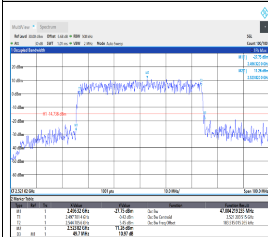
1-N41--30-50-L-6-CP-QPSK-Outer_Full-133 @0-Ant1-47.004-49.700-≤50-PASS
