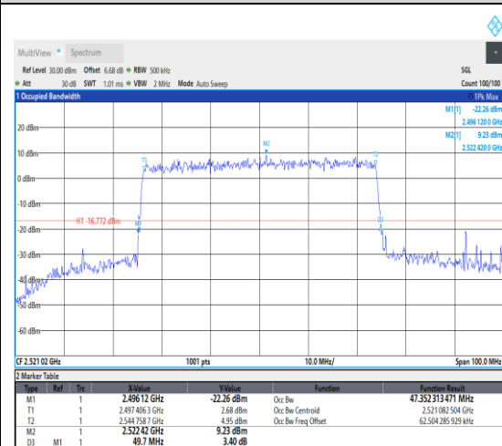
1-N41--30-50-L-9-CP-256QAM-Outer_Full-13 3@0-Ant1-47.352-49.700-≤50-PASS
