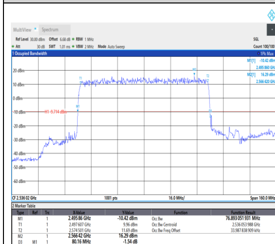
1-N41--30-80-L-2-DFT-PI2BPSK-Outer_Full- 216@0-Ant1-76.893-80.160-≤80-PASS
