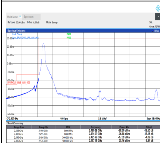
1-N41--30-30-L-1-DFT-PI2BPSK-Edge_1RB_Left-1@0-Ant1-1--PASS-see graph
