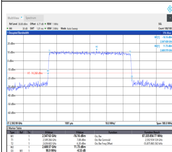
1-N41--30-90-M-8-CP-64QAM-Outer_Full-24 5@0-Ant1-87.336-90.900-≤90-PASS
