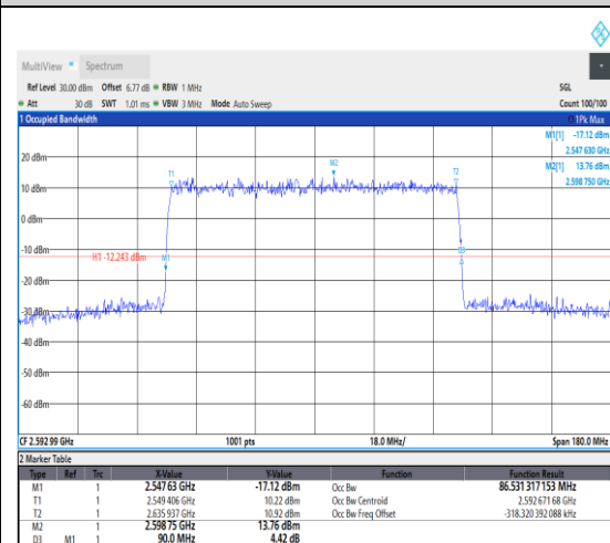
1-N41--30-90-M-3-DFT-16QAM-Outer_Full-2 43@0-Ant1-86.531-90.000-≤90-PASS
