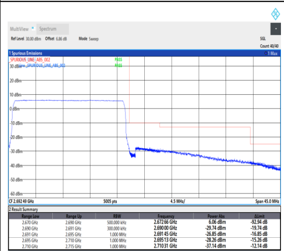
1-N41--30-20-H-6-CP-QPSK-Outer_Full-51@0-Ant1-1--PASS-see graph
