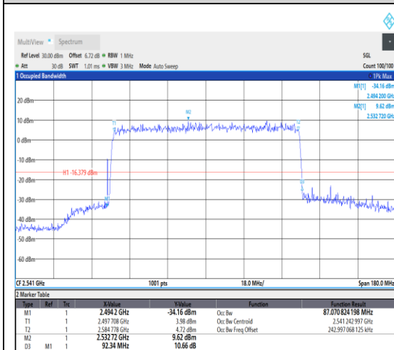
1-N41--30-90-L-9-CP-256QAM-Outer_Full-24 5@0-Ant1-87.071-92.340-≤90-PASS
