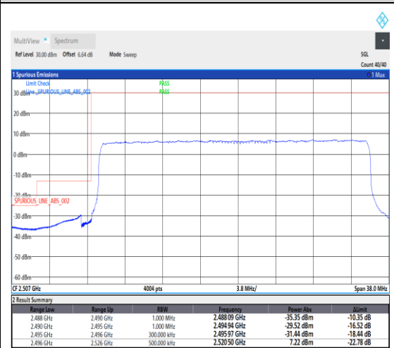
1-N41--30-30-L-3-DFT-PI2BPSK-Outer_Full-75@0-Ant1-1--PASS-see graph
