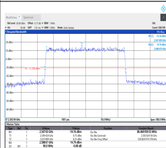
1-N41--30-90-M-1-DFT-QPSK-Outer_Full-24 3@0-Ant1-86.47-90.000-≤90-PASS
