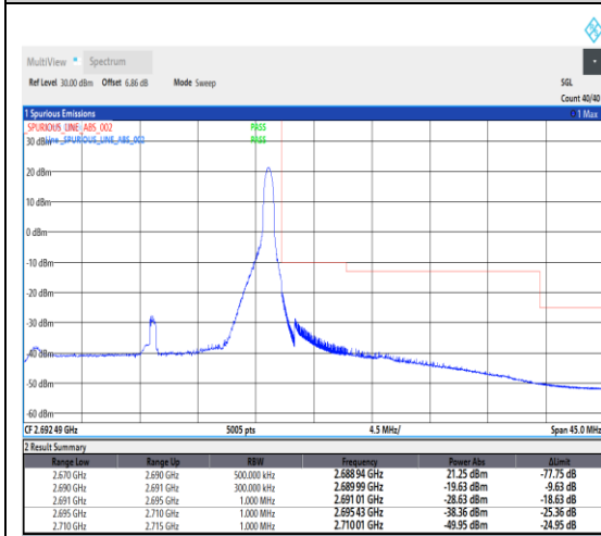
1-N41--30-20-H-5-CP-QPSK-Edge_1RB_Right-1@50-Ant1-1--PASS-see graph
