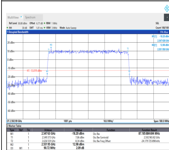
1-N41--30-90-M-6-CP-QPSK-Outer_Full-245 @0-Ant1-87.186-90.720-≤90-PASS
