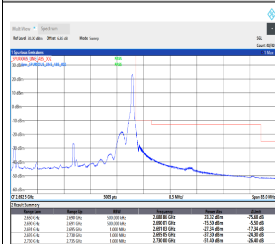
1-N41--30-40-H-2-DFT-PI2BPSK-Edge_1RB_Right-1@105-Ant1-1--PASS-see graph
