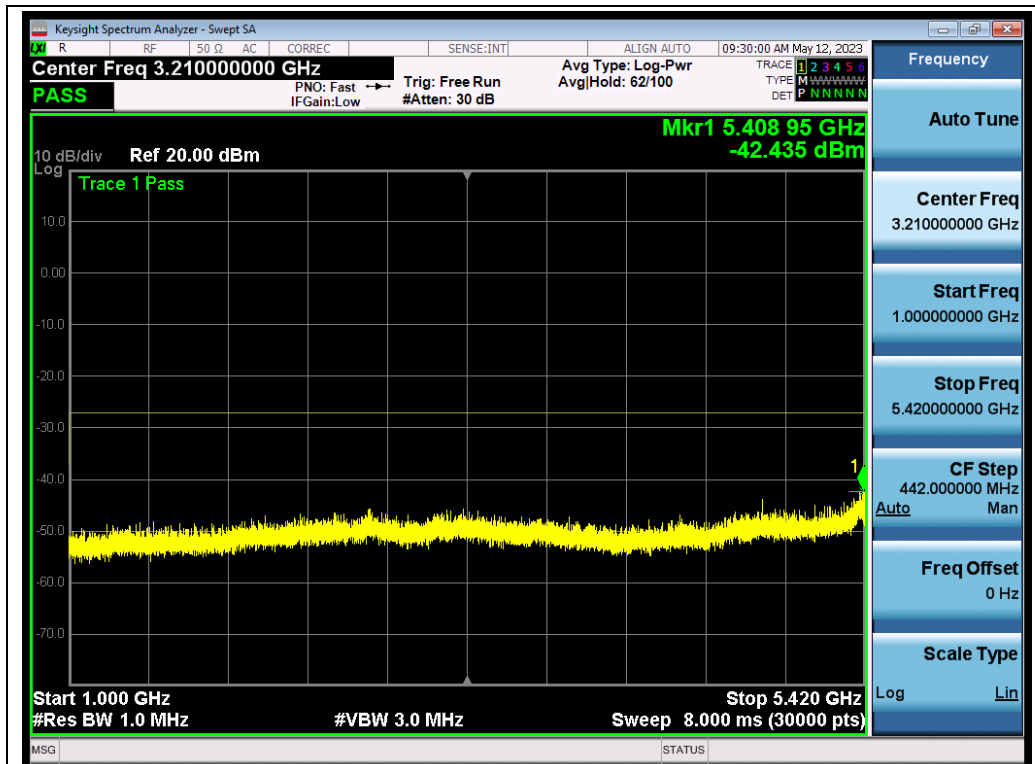
802.11ac80_ANT1_5530_MCS0_Frequency Band 2
