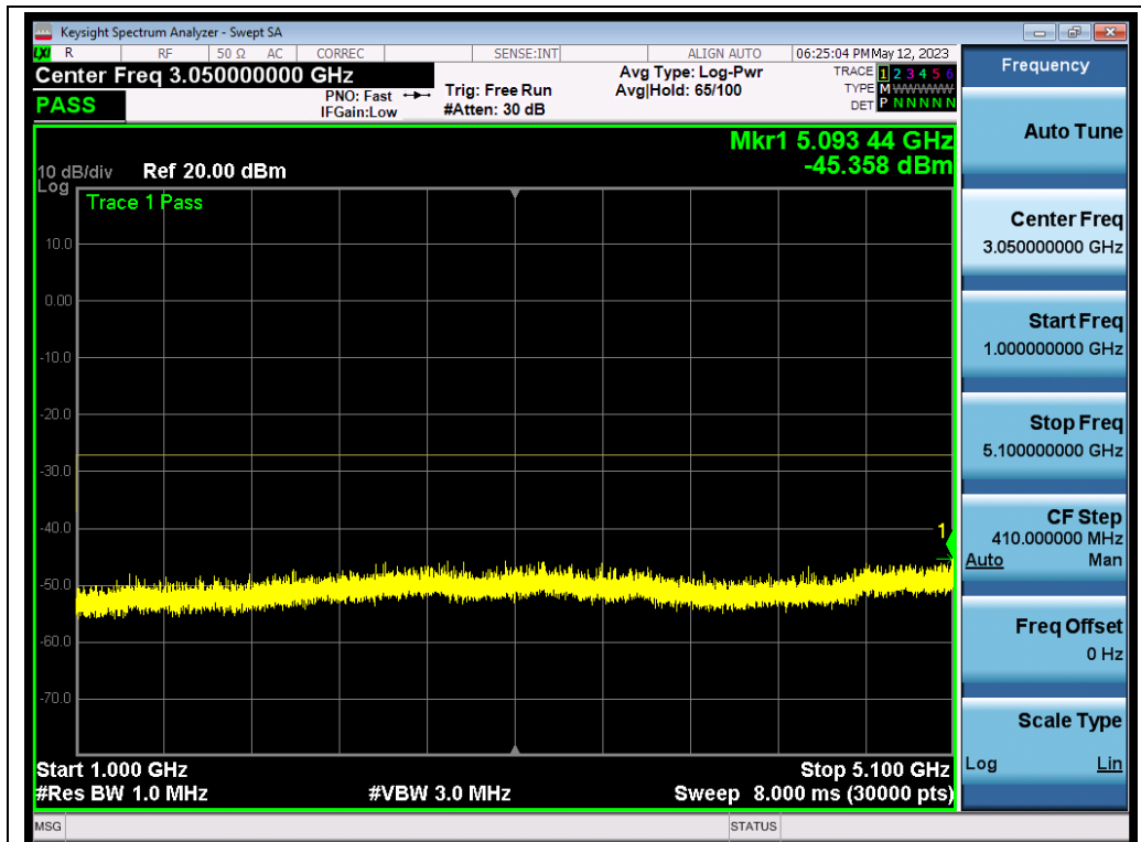
802.11ac80_ANT1_5290_MCS0_Frequency Band 2
