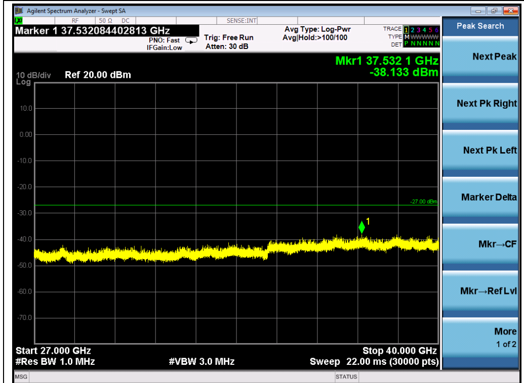
802.11n40_ANT1_5590_MCS0_Frequency Band 5
