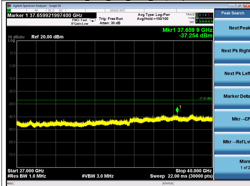
802.11ac80_ANT1_5530_MCS0_Frequency Band 5
