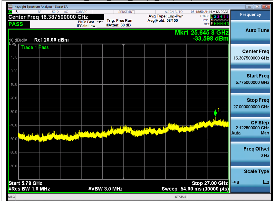
802.11a ANT1 5500 6Mbps Frequency Band 4
