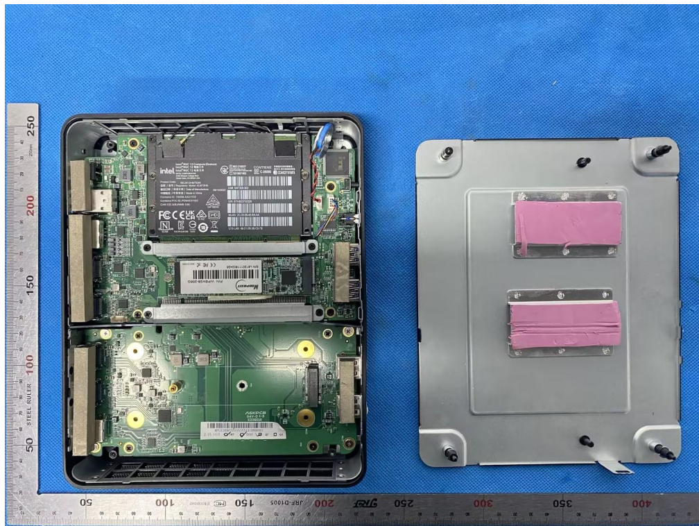
OPEN VIEW OF EUT (FIGURE 1) -DP PORT
