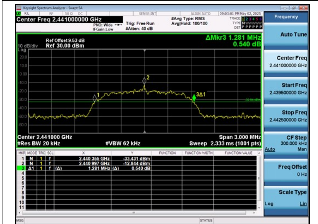
3DH5_Ant1_2441
