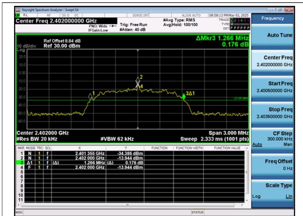
3DH5_Ant1_2402
