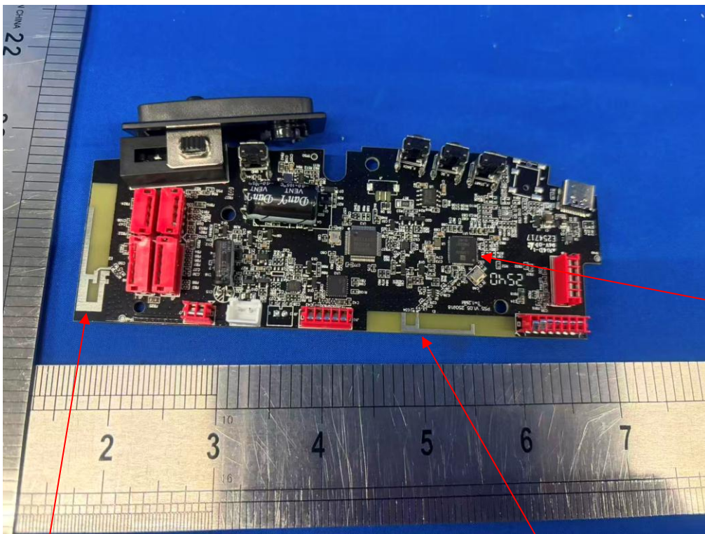
Antenna 2: BL-EC1950331-902 (2.4GHz SRD & Bluetooth)
