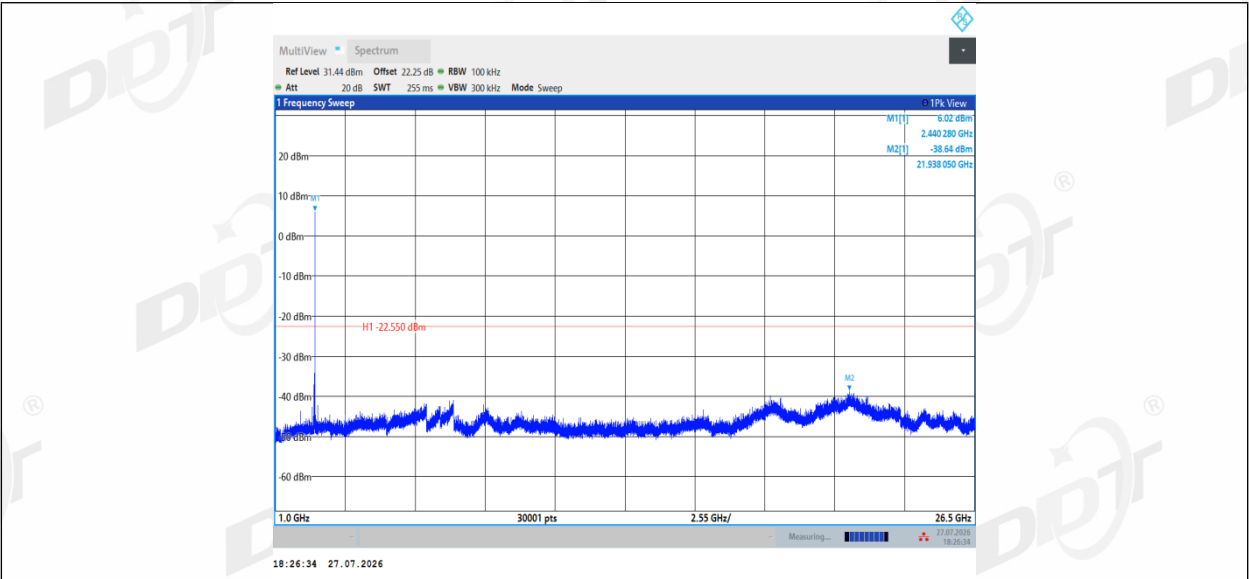
BLE_1M_Ant1_2480_0~Reference
