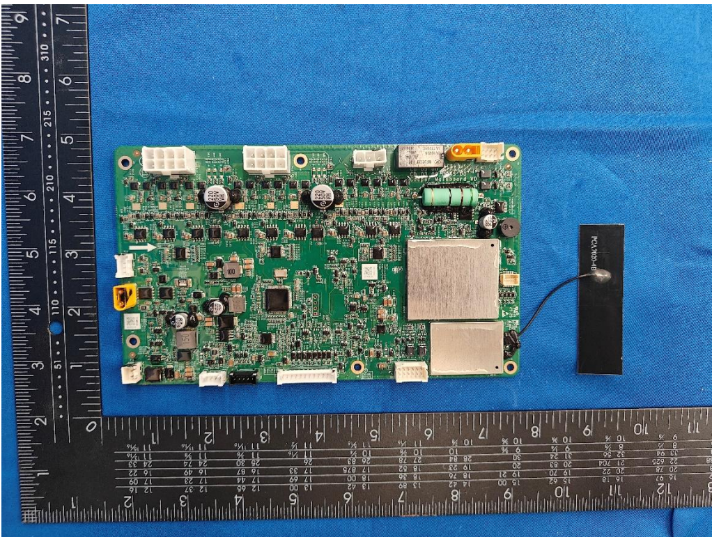
(42) EUT Photo
