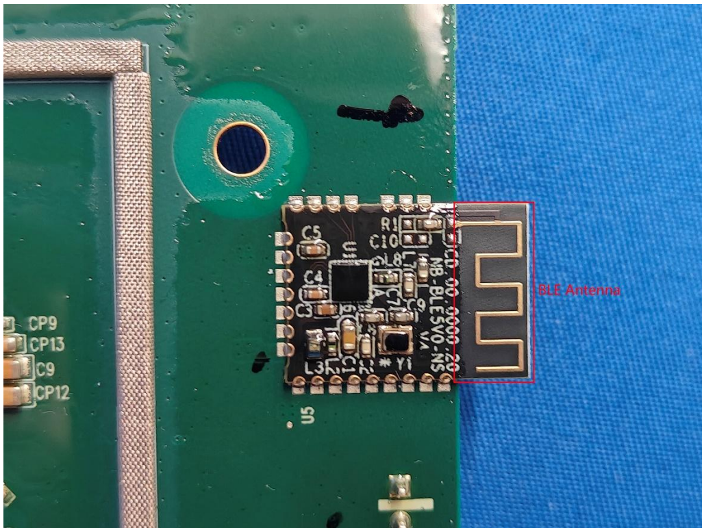
(38) EUT Photo
