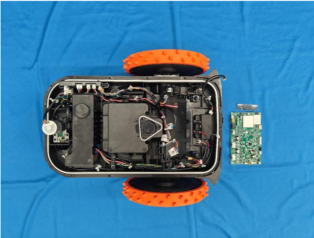
(42) EUT Photo
