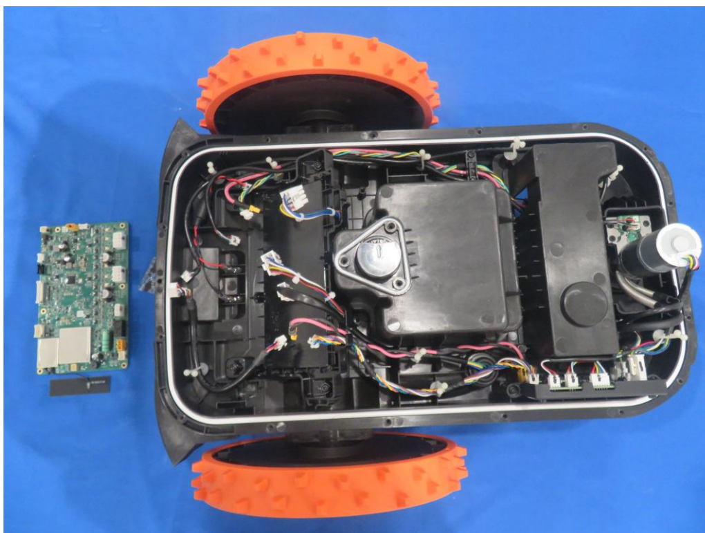
(38) EUT Photo
