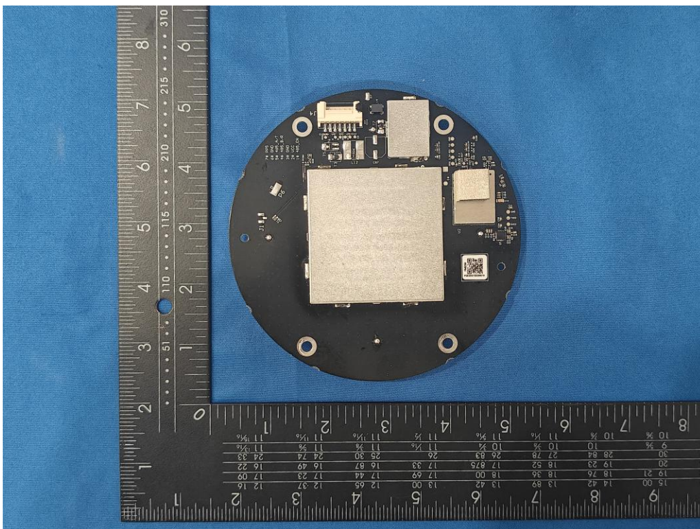
(22) EUT Photo
