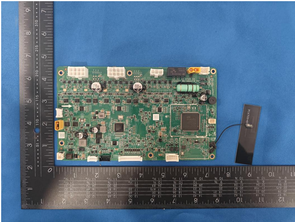
(42) EUT Photo
