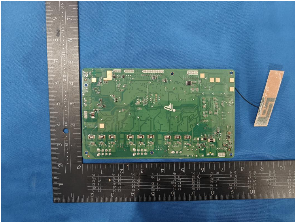
(45) EUT Photo
