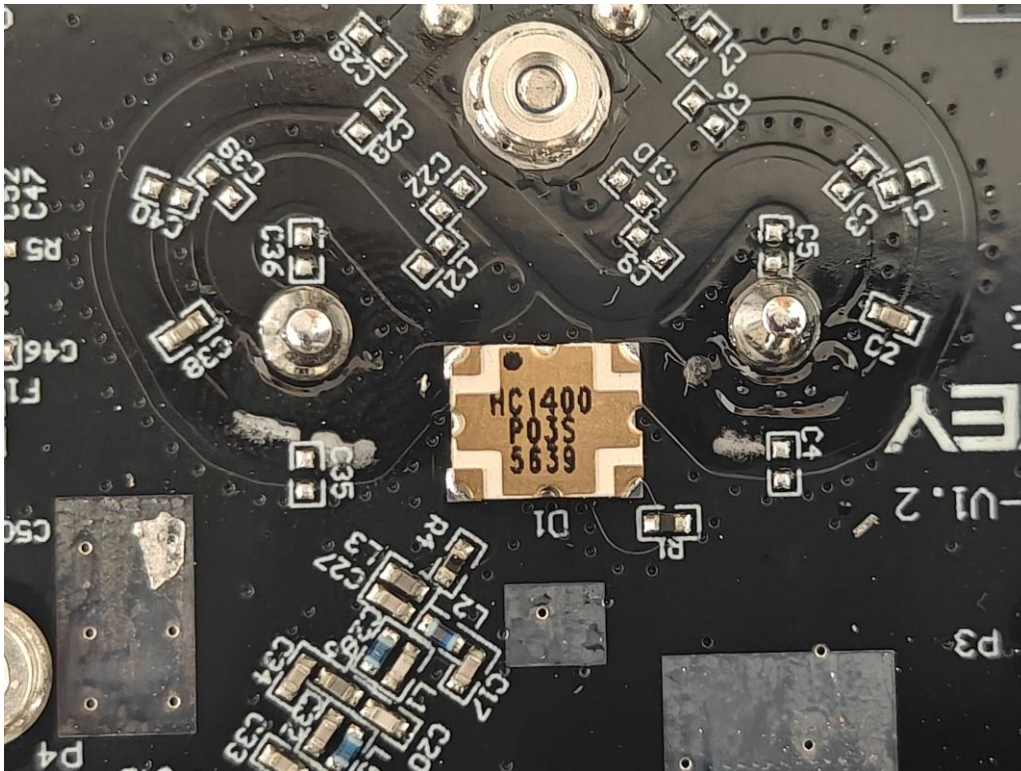
(28) EUT Photo
