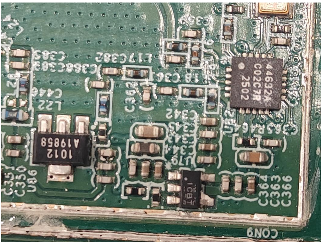
(42) EUT Photo
