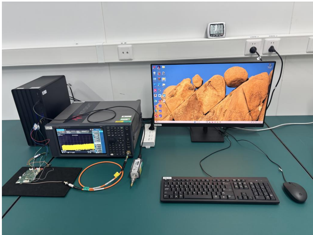
Description: Conducted Test Setup for SRD (WJ-SR3)
