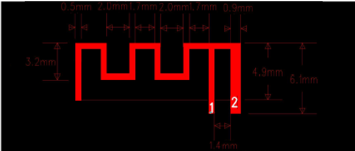
Antenna Photo & Length (mm)
