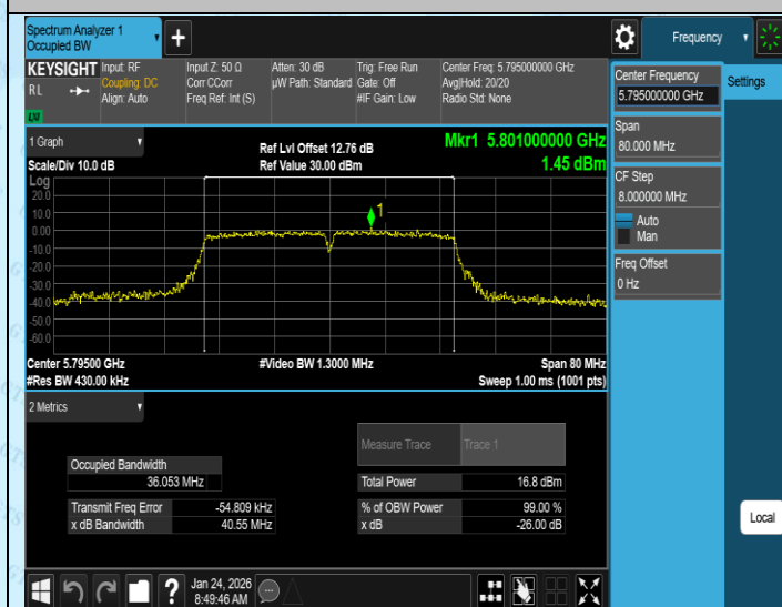
11AC40SISO-Ant1-5795
