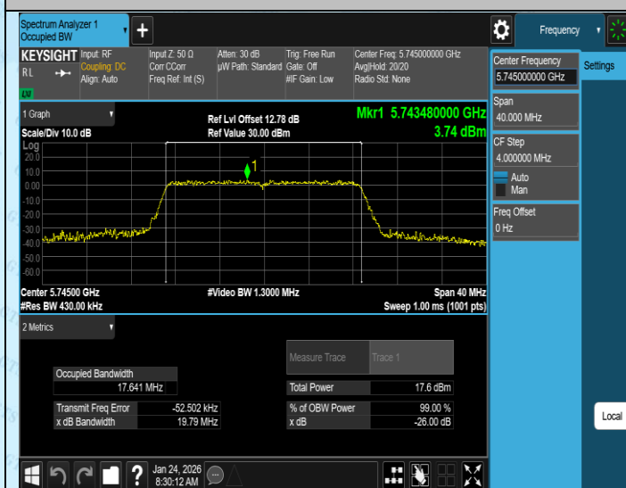
11AC20SISO-Ant1-5745
