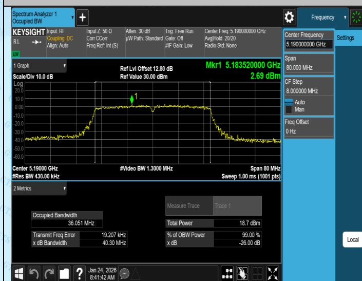
11AC40SISO-Ant1-5190
