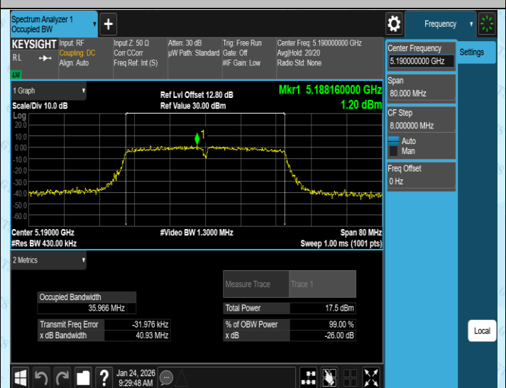
11AC40SISO-Ant2-5190
