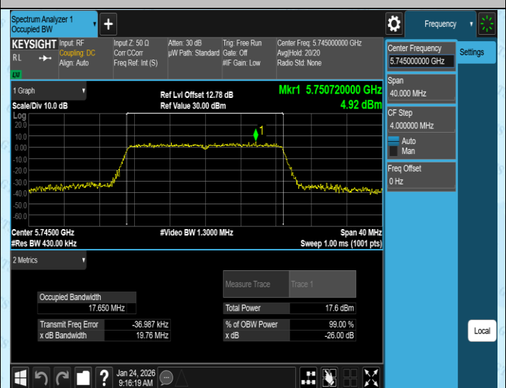
11AC20SISO-Ant2-5745
