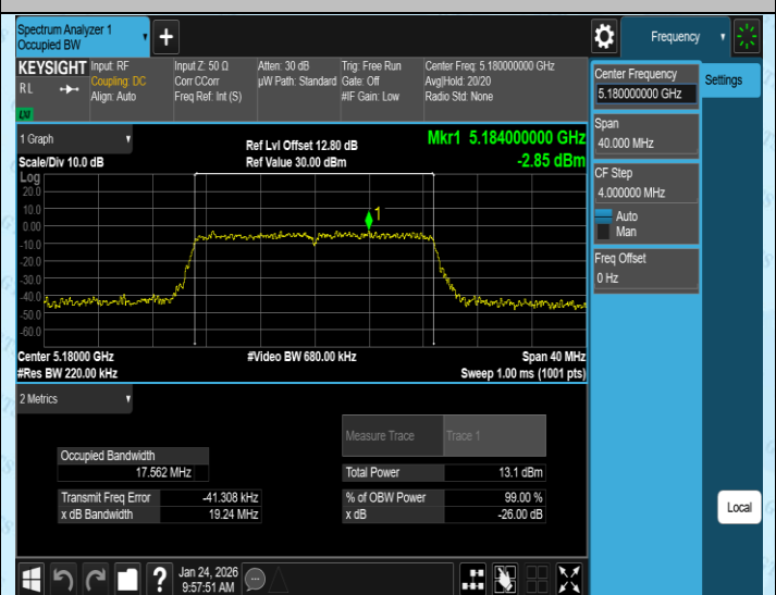
11AC20MIMO-Ant2-5180
