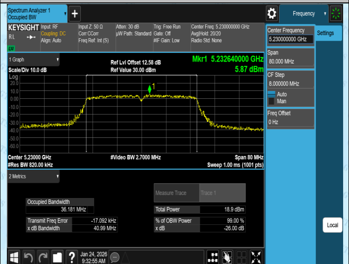
11AC40SISO-Ant2-5230
