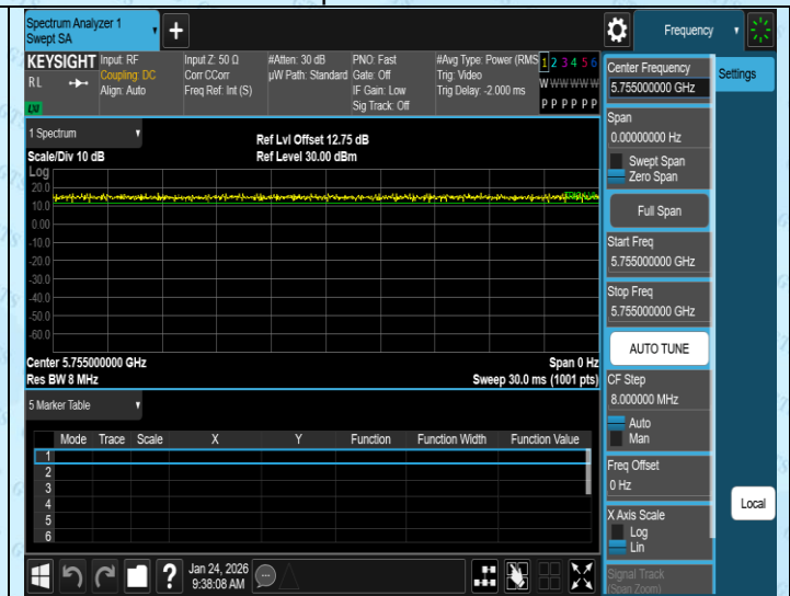
NTNV-11AC40SISO-Ant2-5755
