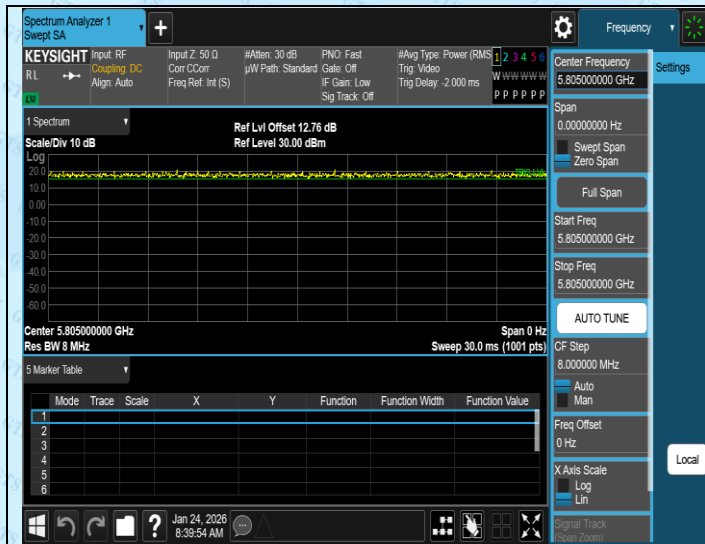
NTNV-11AC20SISO-Ant1-5805
