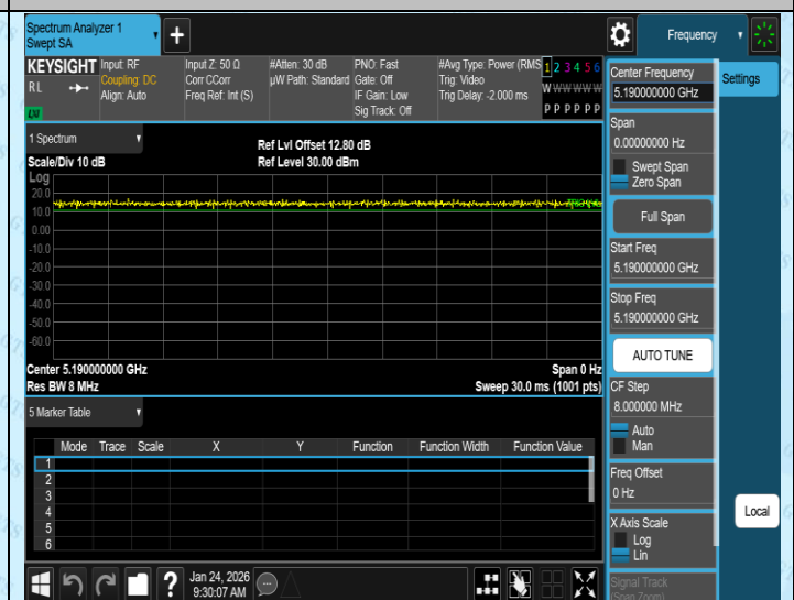
NTNV-11AC40SISO-Ant2-5190
