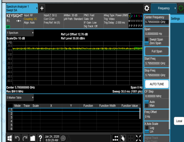
NTNV-11AC40SISO-Ant1-5795
