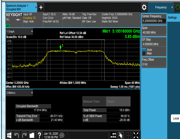
11AC20SISO-Ant3-5200
