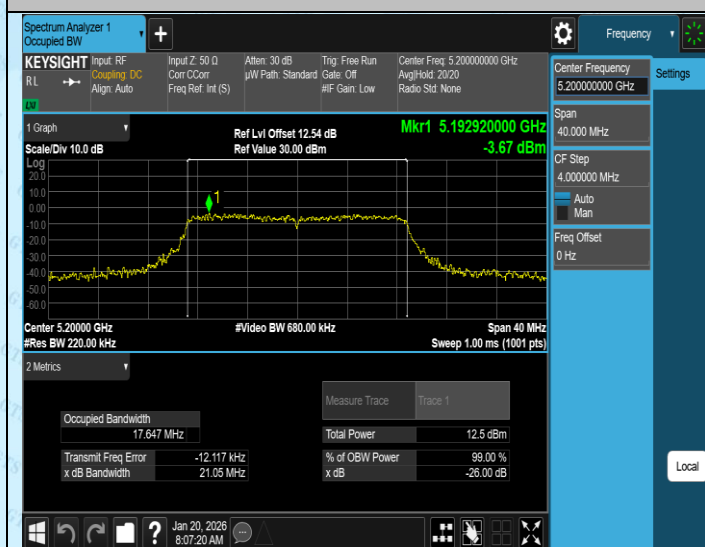
11AC20MIMO-Ant3-5200
