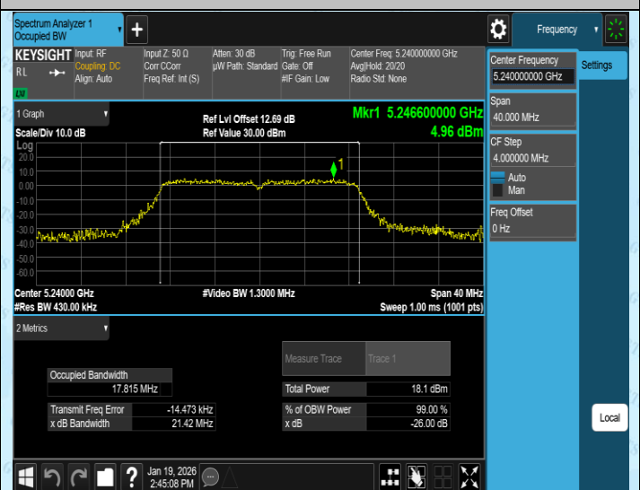
11AC20SISO-Ant4-5240
