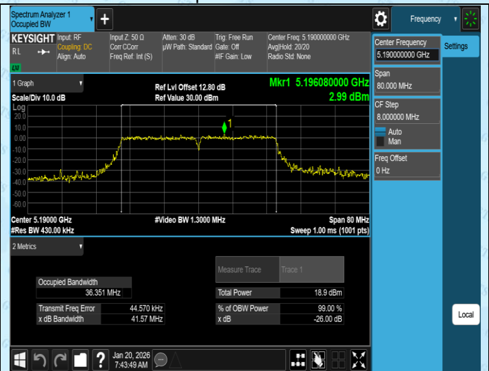
11AC40SISO-Ant4-5190
