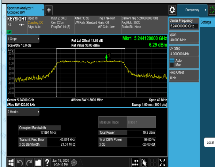
11AC20SISO-Ant3-5240
