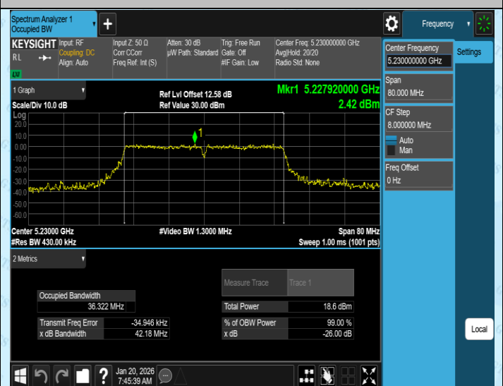
11AC40SISO-Ant4-5230
