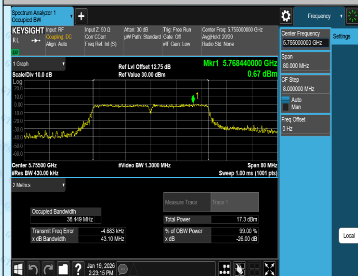
11AC40SISO-Ant3-5755
