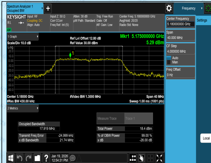
11AC20SISO-Ant3-5180
