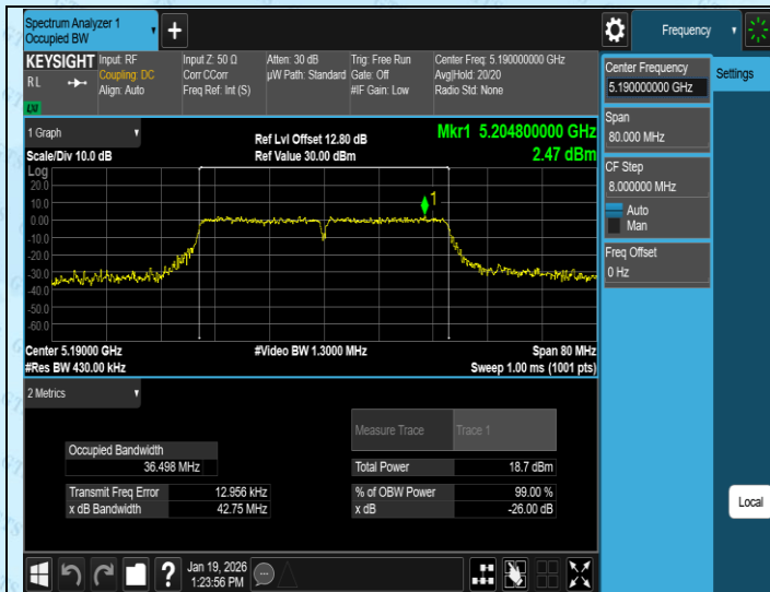
11AC40SISO-Ant3-5190
