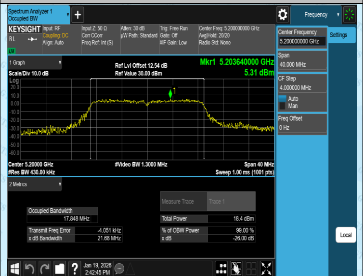
11AC20SISO-Ant4-5200
