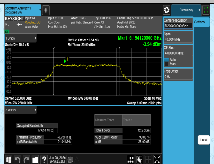
11AC20MIMO-Ant4-5200
