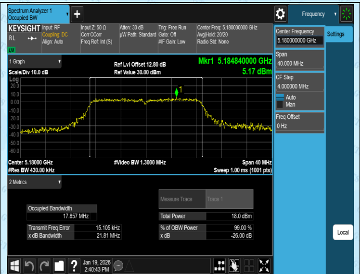
11AC20SISO-Ant4-5180
