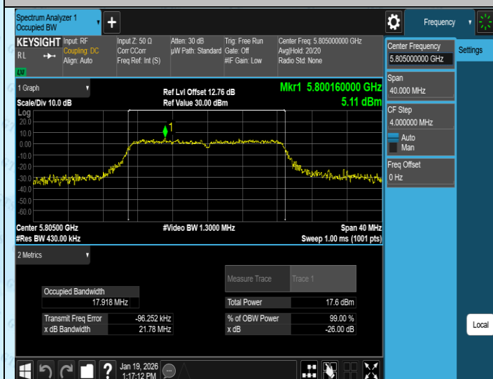
11AC20SISO-Ant3-5805
