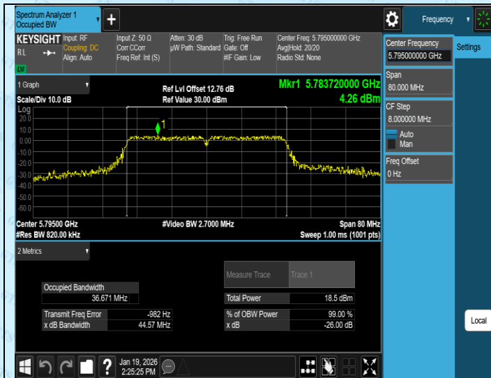
11AC40SISO-Ant3-5795
