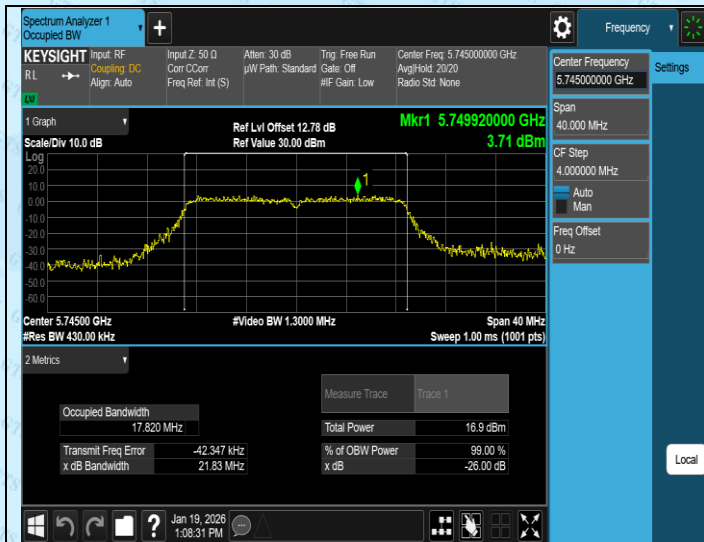
11AC20SISO-Ant3-5745
