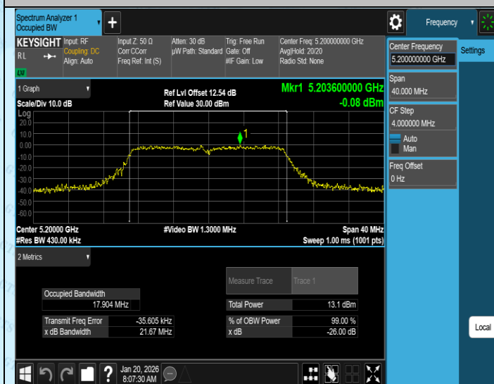
11AC20MIMO-Ant3-5200
