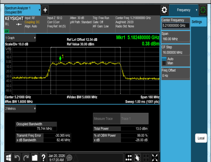
11AC80MIMO-Ant4-5210
