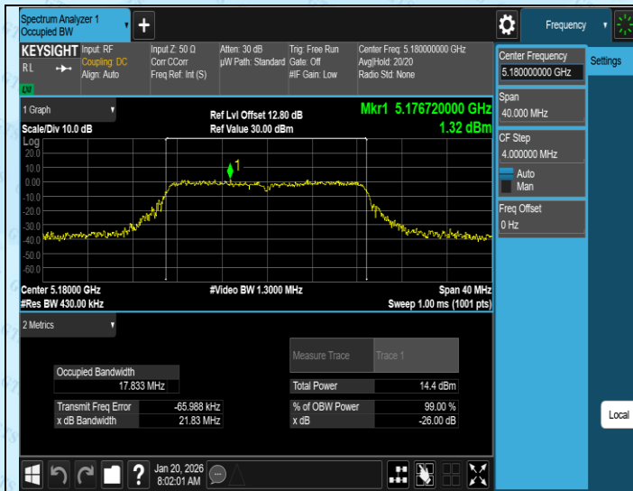
11AC20MIMO-Ant3-5180
