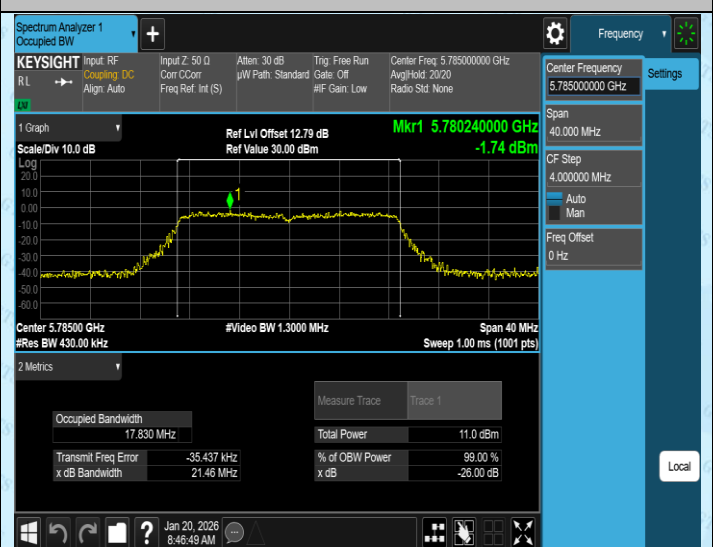
11AC20MIMO-Ant4-5785
