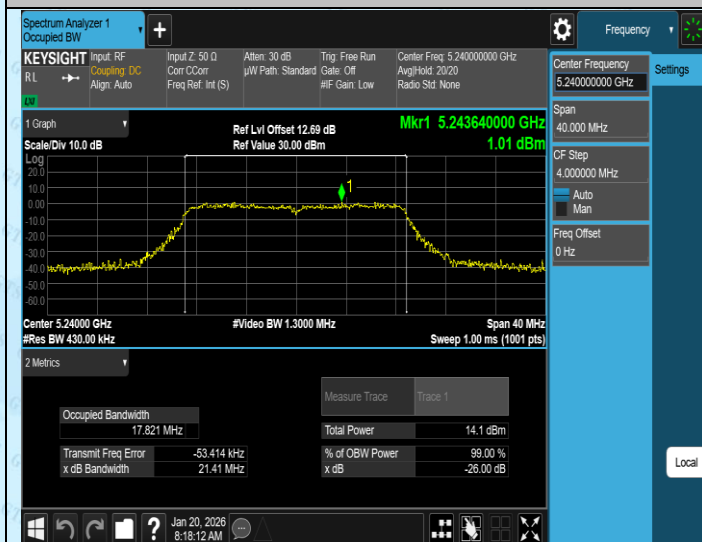
11AC20MIMO-Ant3-5240
