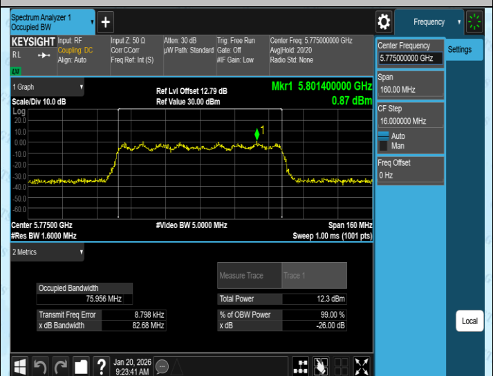
11AC80MIMO-Ant4-5775
