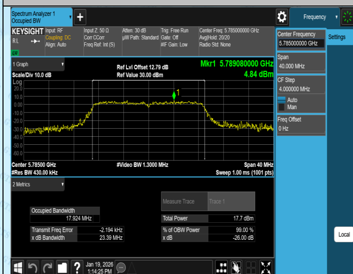
11AC20SISO-Ant3-5785
