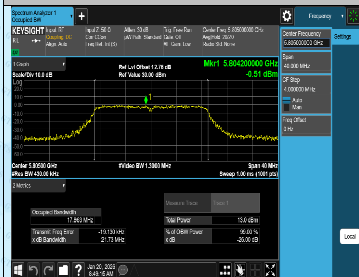
11AC20MIMO-Ant3-5805
