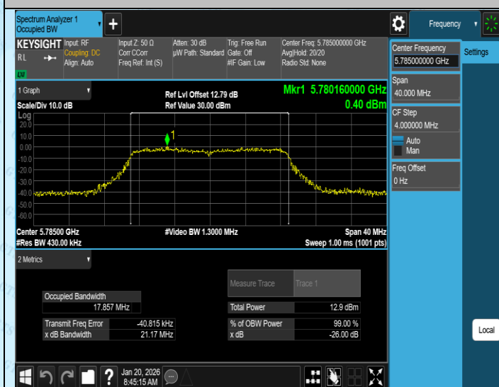
11AC20MIMO-Ant3-5785
