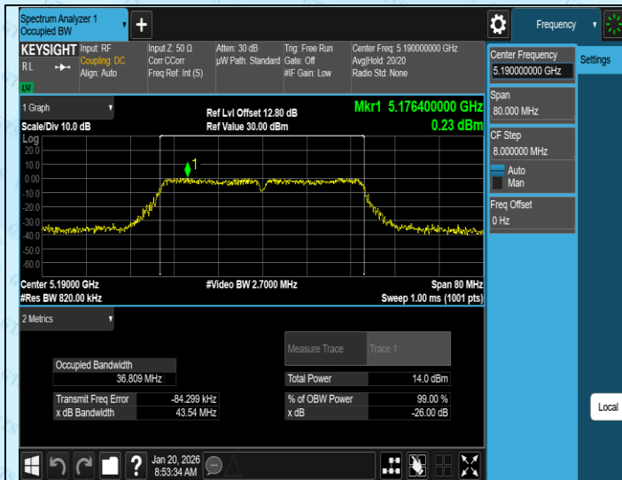
11AC40MIMO-Ant3-5190
