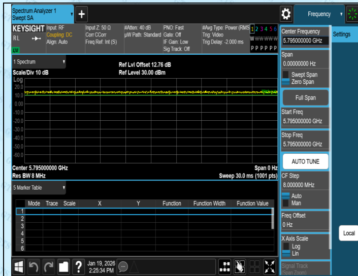
NTNV-11AC40SISO-Ant3-5795
