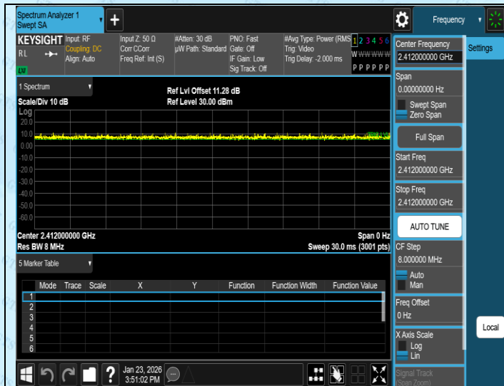
NTNV-11N20MIMO-Ant1-2412
