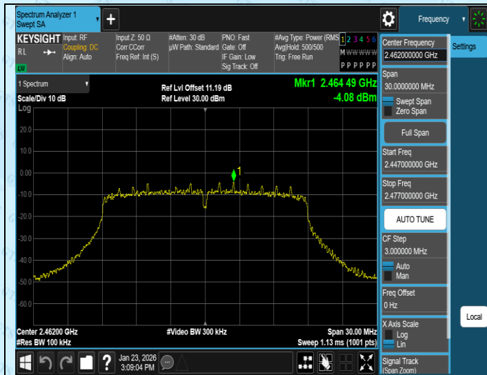
11N20SISO-Ant1-2462-0~Reference-PASS
