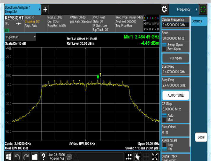
11N20SISO-Ant2-2462-0~Reference-PASS
