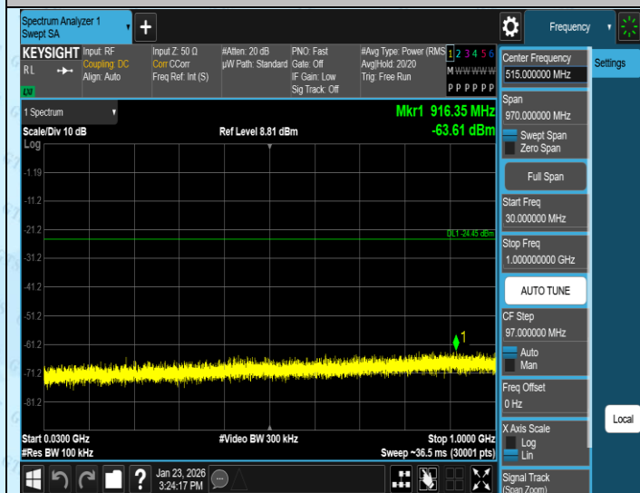
11N20SISO-Ant2-2462-30~1000-PASS
