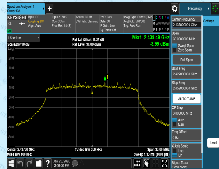
11N20SISO-Ant1-2437-0~Reference-PASS
