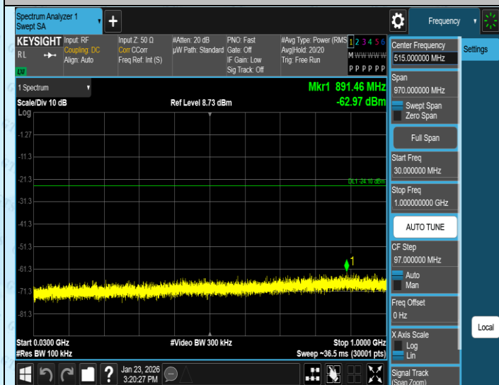
11N20SISO-Ant2-2437-30~1000-PASS
