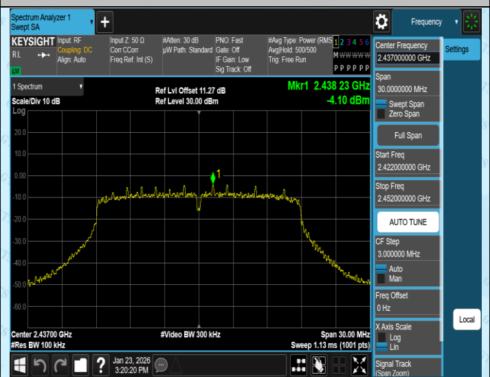
11N20SISO-Ant2-2437-0~Reference-PASS
