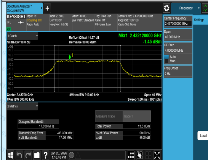
11N20SISO-Ant3-2437-PASS
