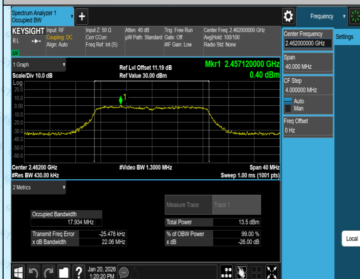
11N20SISO-Ant3-2462
