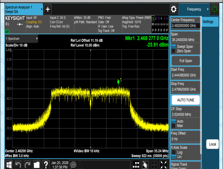
11N20MIMO-Ant4-2462-PASS
