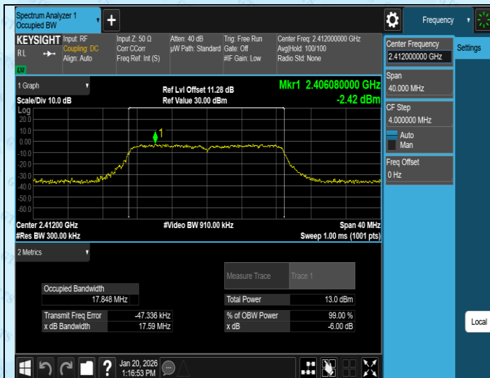
11N20SISO-Ant3-2412-PASS
