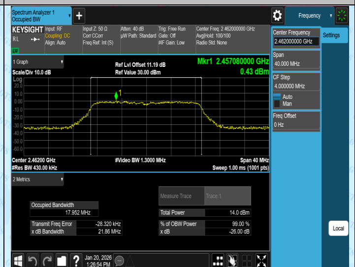
11N20SISO-Ant4-2462
