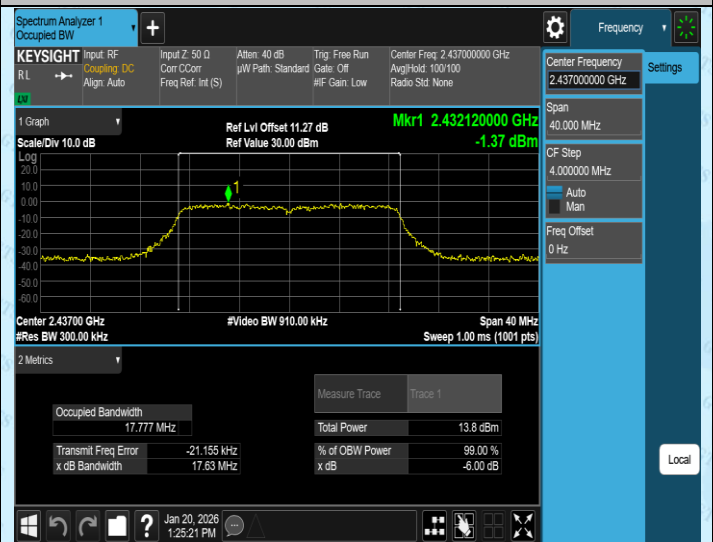
11N20SISO-Ant4-2437-PASS
