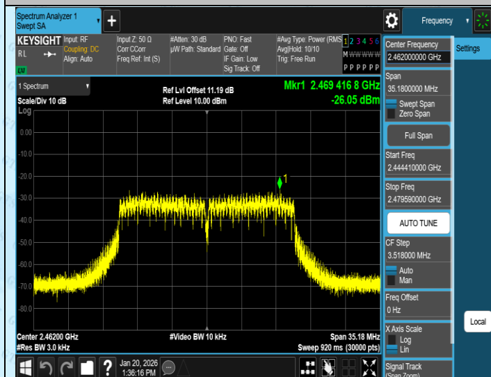
11N20MIMO-Ant3-2462-PASS
