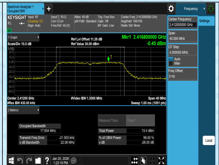
11N20SISO-Ant4-2412
