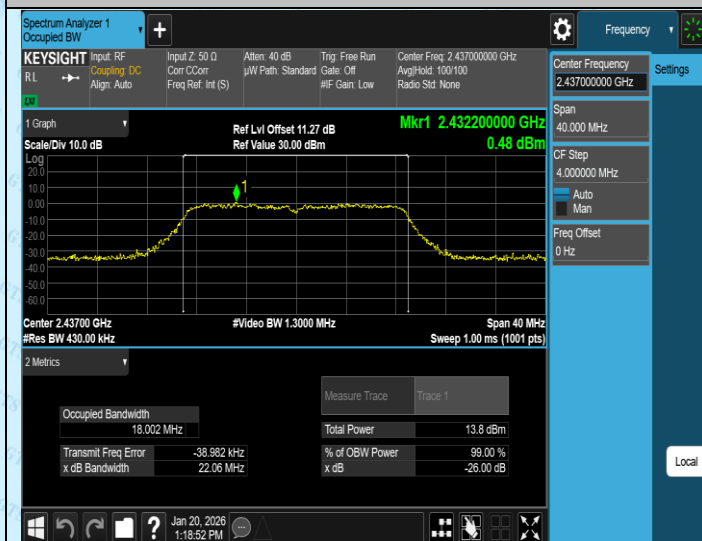
11N20SISO-Ant3-2437
