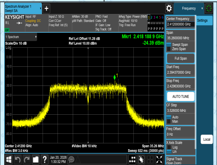
11N20MIMO-Ant4-2412-PASS
