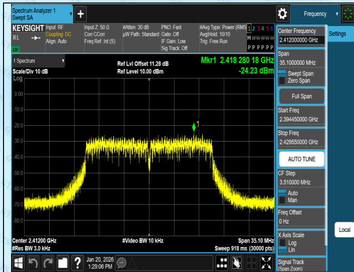
11N20MIMO-Ant3-2412-PASS
