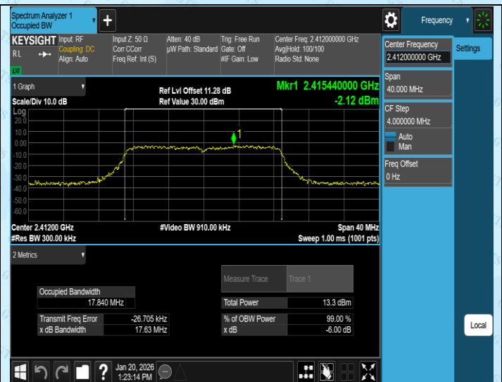
11N20SISO-Ant4-2412-PASS
