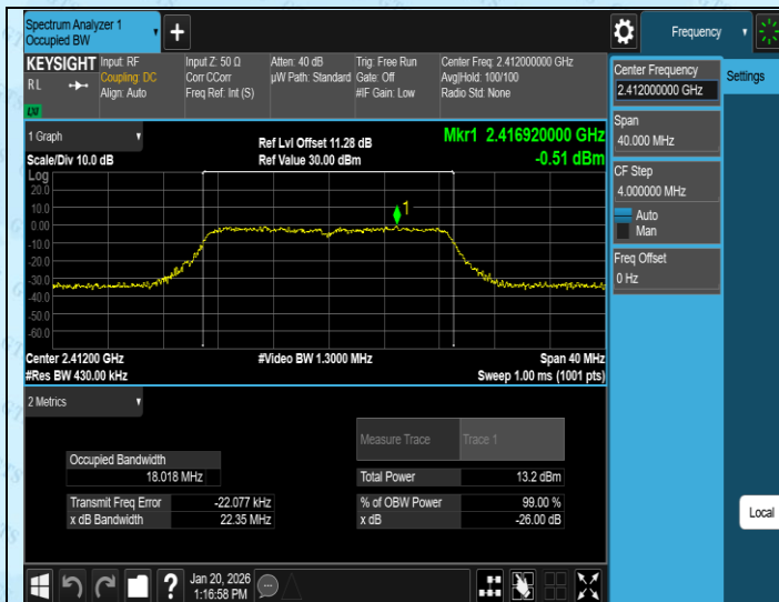
11N20SISO-Ant3-2412
