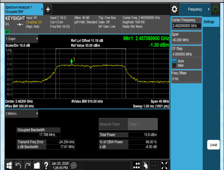
11N20SISO-Ant4-2462-PASS
