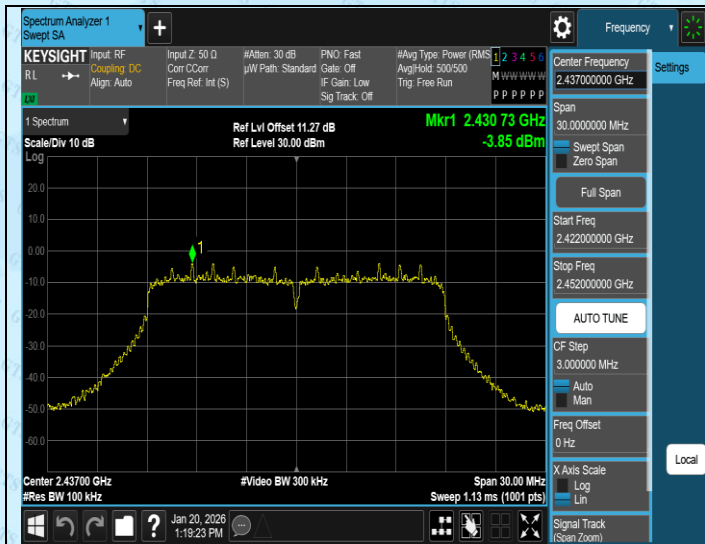
11N20SISO-Ant3-2437-0~Reference-PASS
