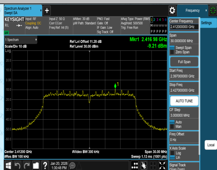
11N20MIMO-Ant4-2412-0~Reference-PASS
