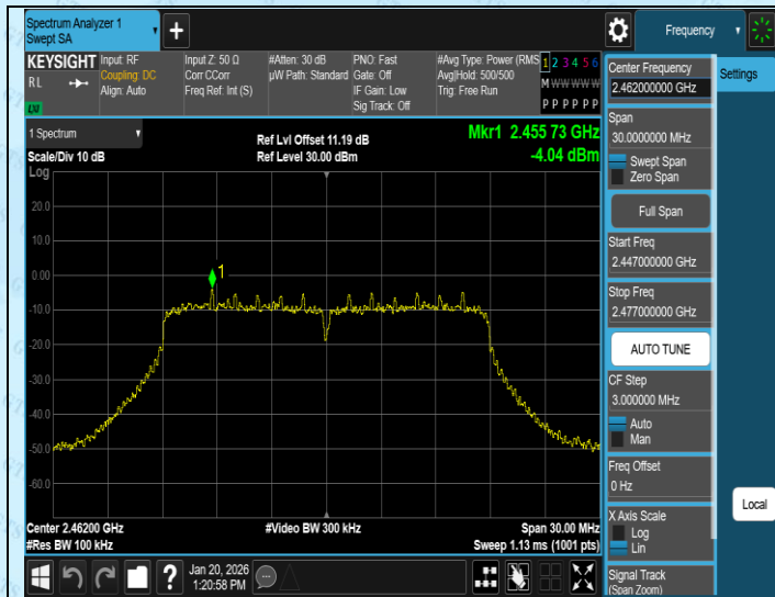
11N20SISO-Ant3-2462-0~Reference-PASS
