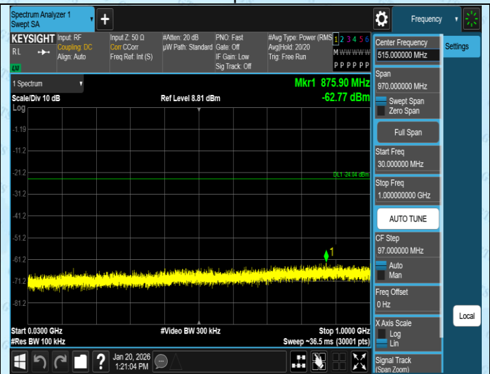
11N20SISO-Ant3-2462-30~1000-PASS
