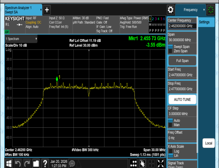
11N20SISO-Ant4-2462-0~Reference-PASS
