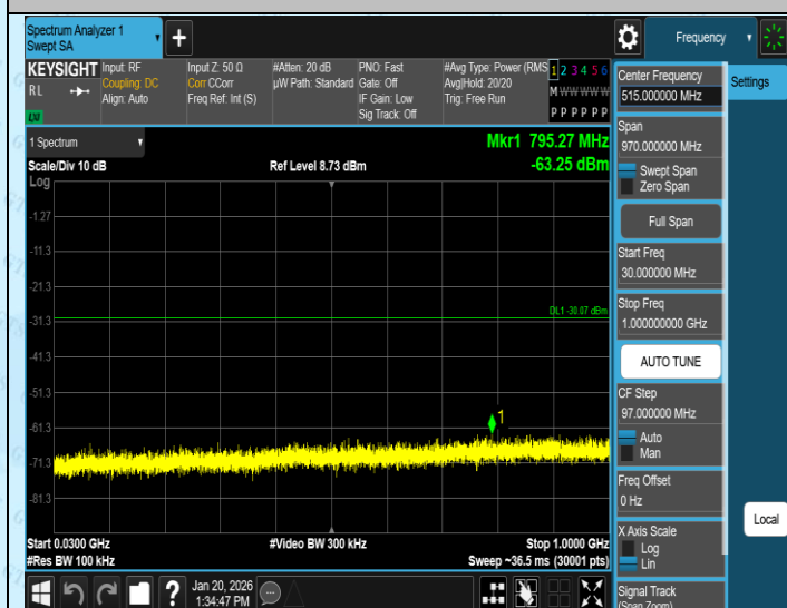
11N20MIMO-Ant4-2437-30~1000-PASS
