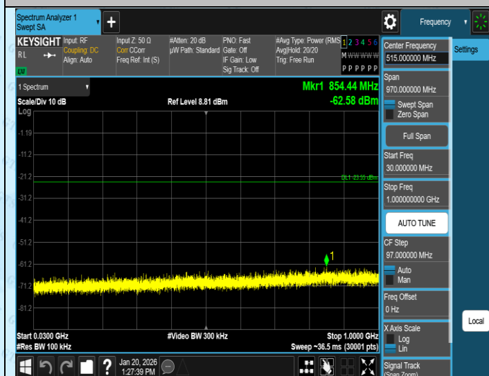
11N20SISO-Ant4-2462-30~1000-PASS
