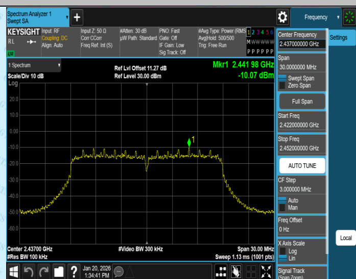
11N20MIMO-Ant4-2437-0~Reference-PASS
