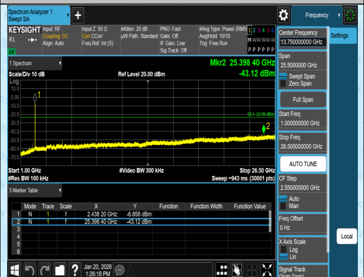
11N20SISO-Ant4-2437-1000~26500-PASS
