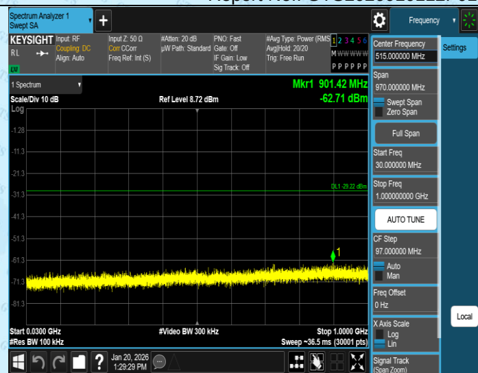
11N20MIMO-Ant3-2412-30~1000-PASS
