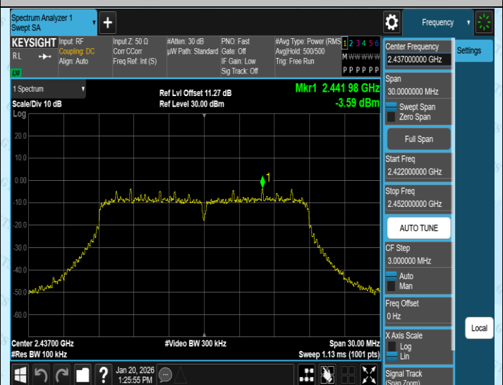
11N20SISO-Ant4-2437-0~Reference-PASS
