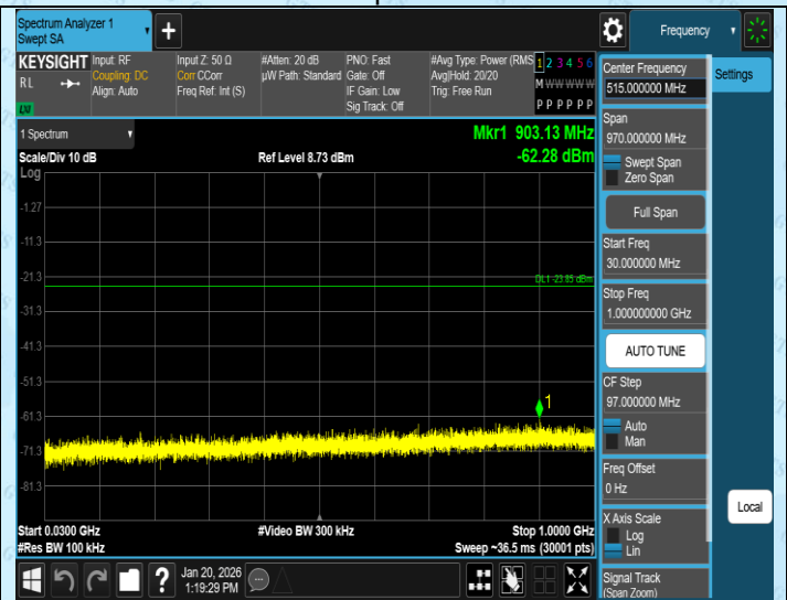
11N20SISO-Ant3-2437-30~1000-PASS
