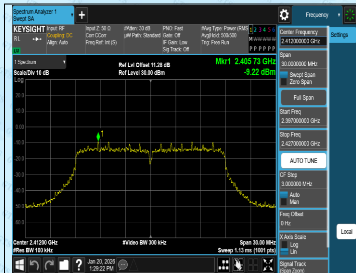
11N20MIMO-Ant3-2412-0~Reference-PASS
