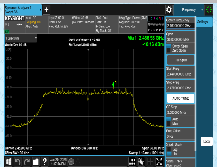
11N20MIMO-Ant4-2462-0~Reference-PASS
