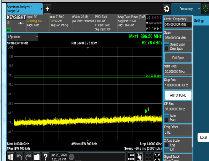
11N20SISO-Ant4-2437-30~1000-PASS
