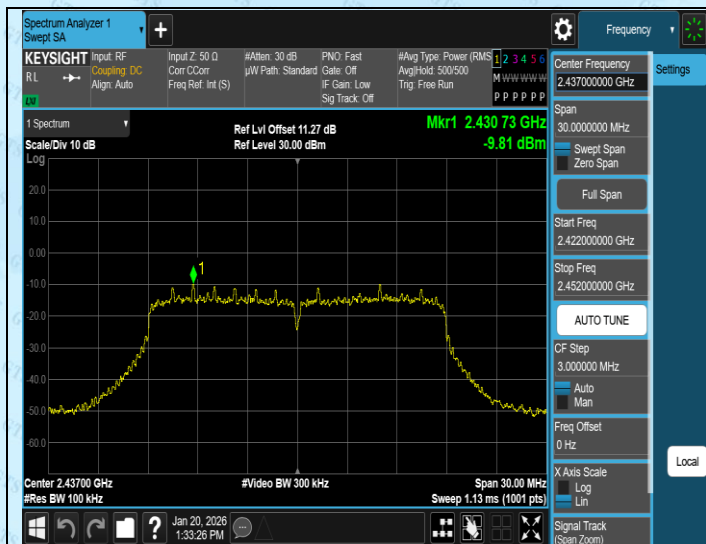
11N20MIMO-Ant3-2437-0~Reference-PASS
