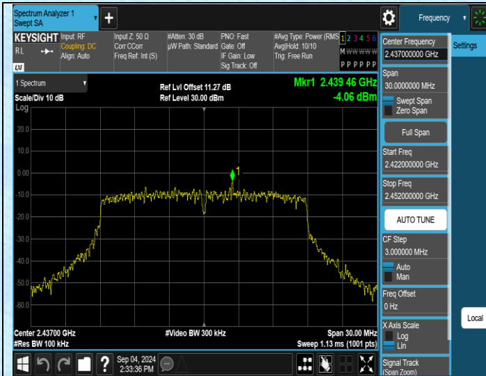
11N20MIMO-Ant1-2437-0~Reference-PASS
