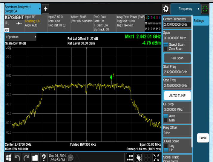
11N20MIMO-Ant2-2437-0~Reference-PASS
