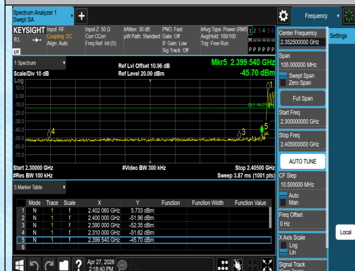
DH5-Ant1-Hop 2402-PASS
