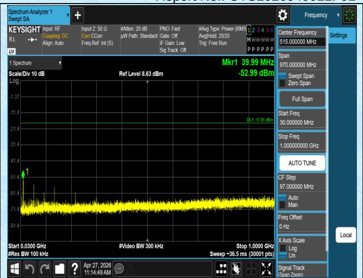
3DH5-Ant1-2480-30~1000-PASS
