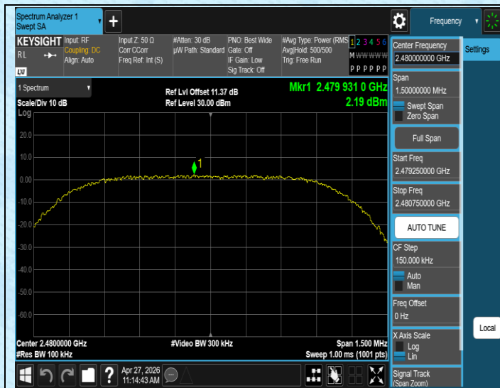
3DH5-Ant1-2480-0~Reference-PASS
