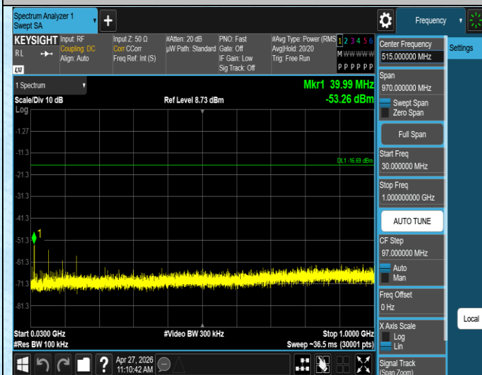
3DH5-Ant1-2441-30~1000-PASS
