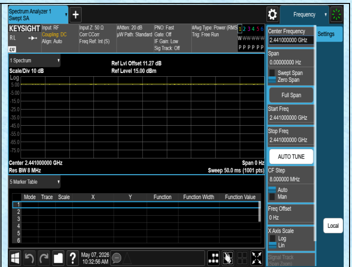
NTNV-DH5-Ant1-2441
