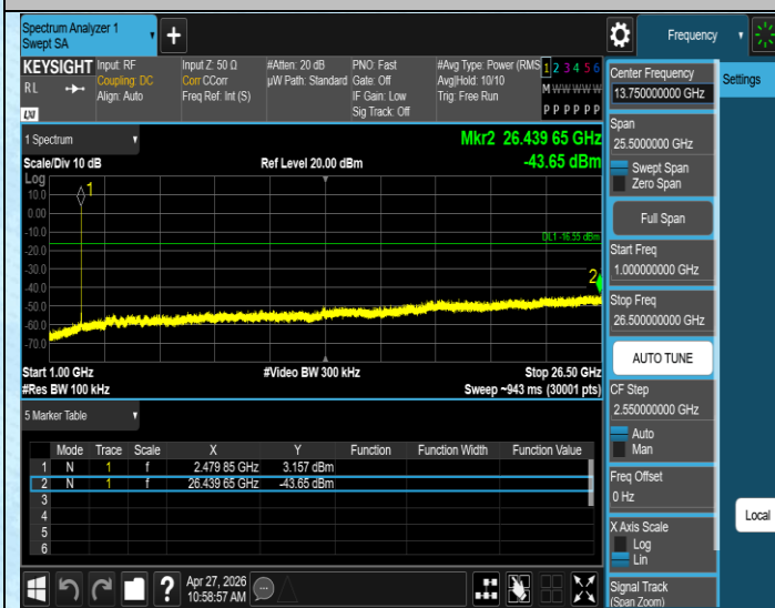
DH5-Ant1-2480-1000~26500-PASS
