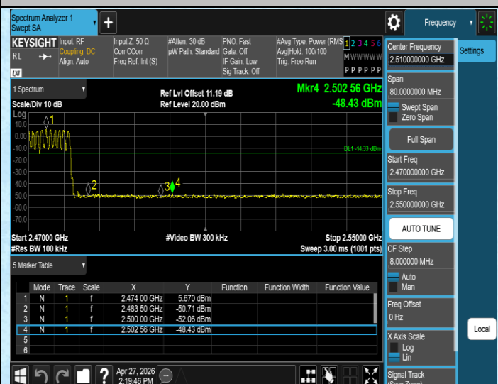
DH5-Ant1-Hop 2480-PASS
