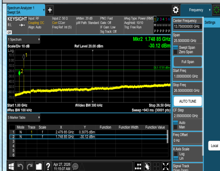
3DH5-Ant1-2480-1000~26500-PASS
