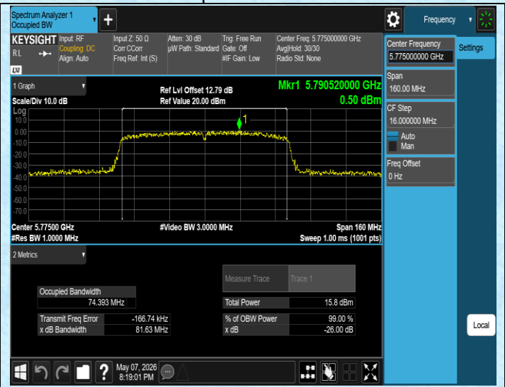
11AC80MIMO-Ant2-5775
