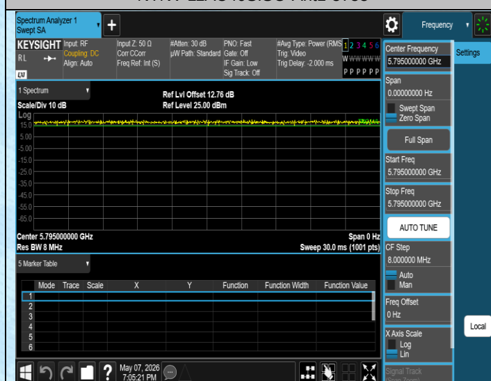
NTNV-11AC40SISO-Ant1-5795
