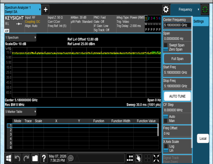
NTNV-11AC20MIMO-Ant2-5180
