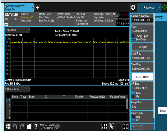
NTNV-11AC20MIMO-Ant1-5180
