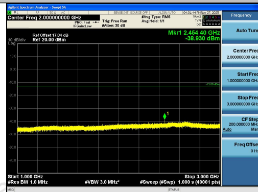
Band26(814-824)-1.4MHz-16QAM-26783-1RB#5- 1000~3000-PASS
