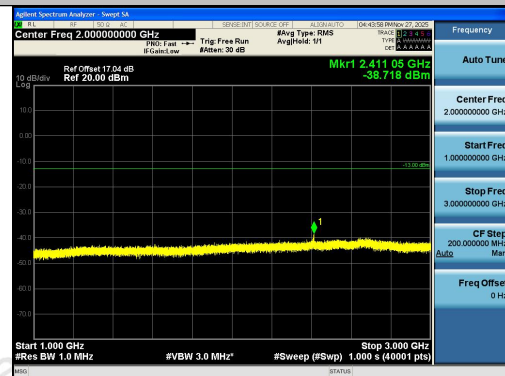
Band26(814-824)-3MHz-16QAM-26705-15RB#0-1 000~3000-PASS
