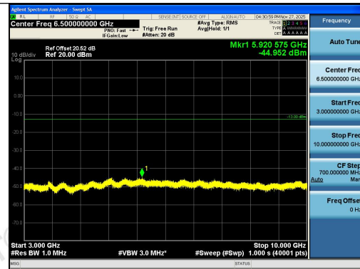
Band26(814-824)-1.4MHz-QPSK-26783-1RB#5-3 000~10000-PASS
