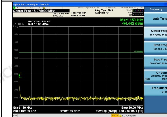
Band26(814-824)-3MHz-QPSK-26705-1RB#0-0.15~30-PASS
