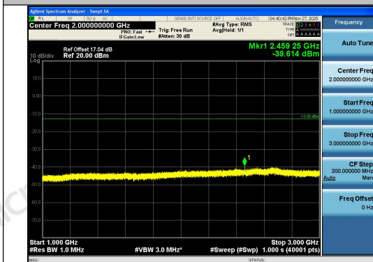
Band26(814-824)-3MHz-QPSK-26705-1RB#14-10 00~3000-PASS
