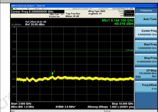
Band26(814-824)-1.4MHz-QPSK-26783-6RB#0-3 000~10000-PASS
