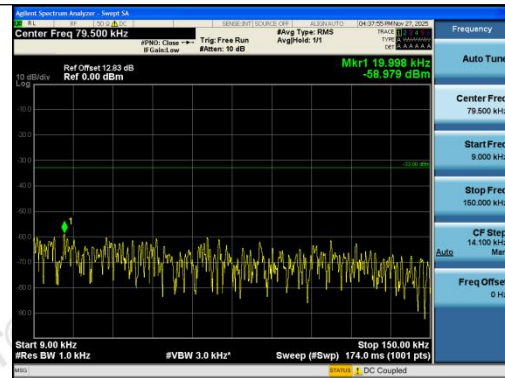
Band26(814-824)-3MHz-QPSK-26705-1RB#0-0.09~0.15-PASS
