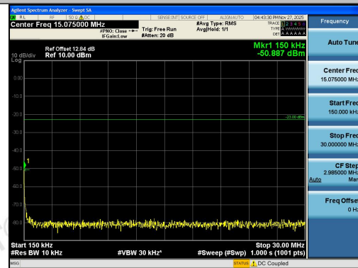
Band26(814-824)-3MHz-16QAM-26705-15RB#0-0 .15~30-PASS
