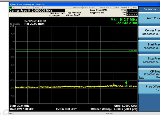
Band26(814-824)-3MHz-QPSK-26705-1RB#14-30 ~1000-PASS
