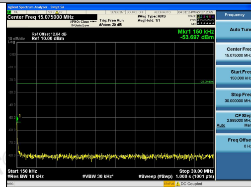
Band26(814-824)-1.4MHz-16QAM-26783-1RB#5- 0.15~30-PASS
