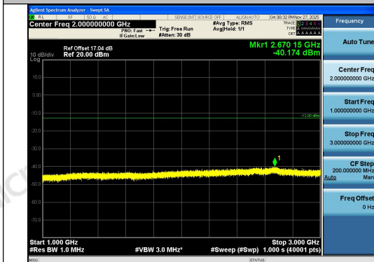
Band26(814-824)-3MHz-QPSK-26705-1RB#0-100~3000-PASS
