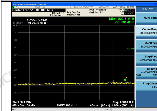
Band26(814-824)-1.4MHz-16QAM-26783-1RB#5- 30~1000-PASS
