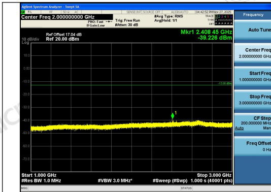
Band26(814-824)-3MHz-QPSK-26705-15RB#0-10 00~3000-PASS
