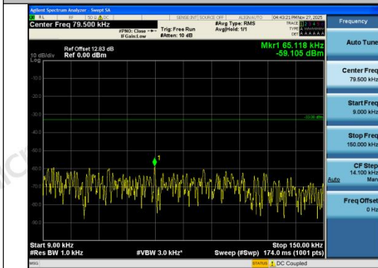
Band26(814-824)-3MHz-16QAM-26705-15RB#0-0 .009~0.15-PASS
