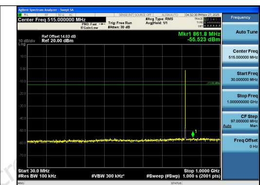
Band26(814-824)-1.4MHz-QPSK-26783-6RB#0-3 0~1000-PASS
