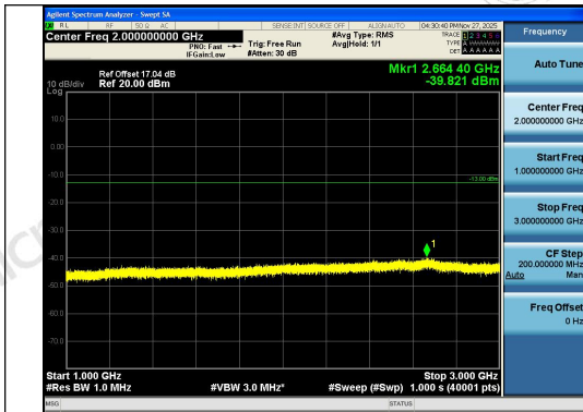
Band26(814-824)-1.4MHz-QPSK-26783-1RB#5-1 000~3000-PASS
