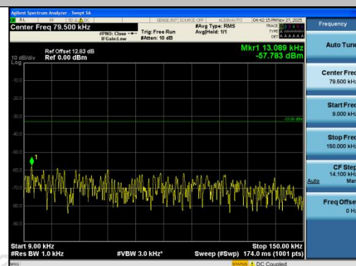
Band26(814-824)-3MHz-QPSK-26705-15RB#0-0. 009~0.15-PASS
