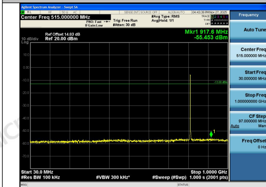
Band26(814-824)-3MHz-16QAM-26705-15RB#0-3 0~1000-PASS
