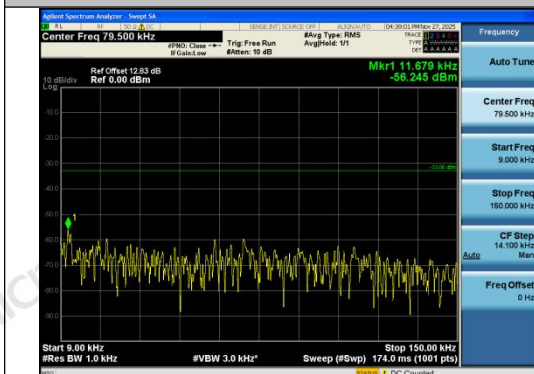
Band26(814-824)-3MHz-16QAM-26705-1RB#0-0.009~0.15-PASS
