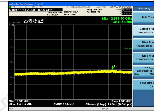
Band26(814-824)-3MHz-16QAM-26705-1RB#0-10 00~3000-PASS
