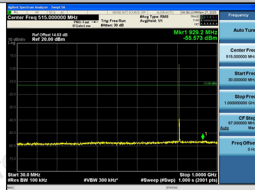
Band26(814-824)-3MHz-QPSK-26705-1RB#0-30~1000-PASS
