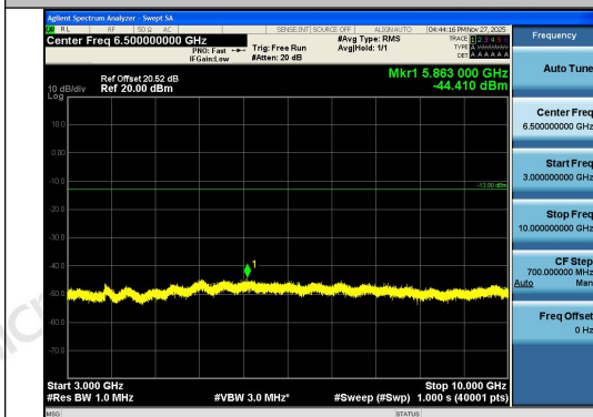
Band26(814-824)-3MHz-16QAM-26705-15RB#0-3 000~10000-PASS
