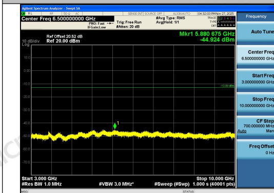
Band26(814-824)-1.4MHz-16QAM-26783-1RB#5- 3000~10000-PASS
