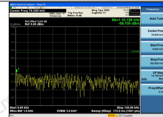
Band26(814-824)-3MHz-QPSK-26705-1RB#14-0. 009~0.15-PASS
