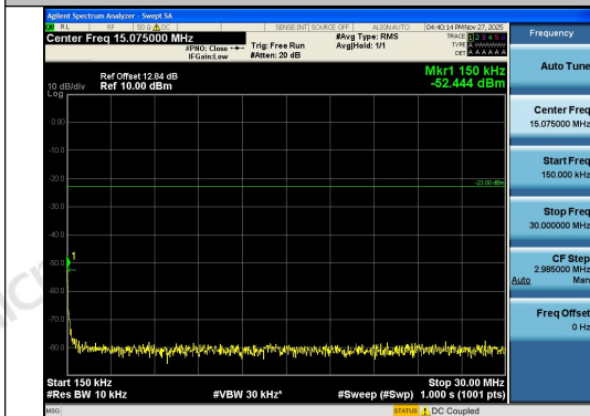
Band26(814-824)-3MHz-QPSK-26705-1RB#14-0. 15~30-PASS
