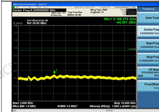
Band26(814-824)-3MHz-16QAM-26705-1RB#0-30 00~10000-PASS
