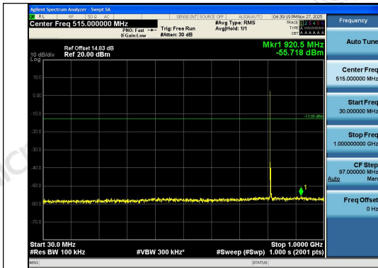
Band26(814-824)-3MHz-16QAM-26705-1RB#0-30 ~1000-PASS
