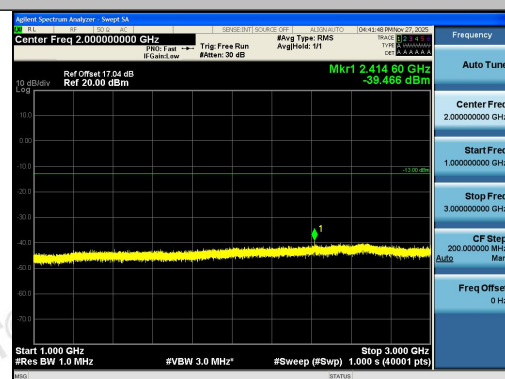
Band26(814-824)-3MHz-16QAM-26705-1RB#14-1 000~3000-PASS
