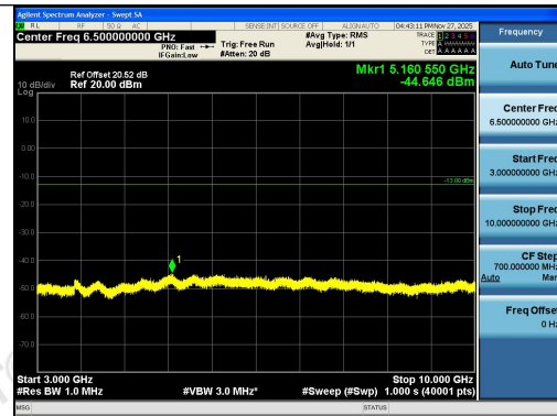
Band26(814-824)-3MHz-QPSK-26705-15RB#0-30 00~10000-PASS
