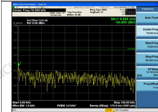
Band26(814-824)-1.4MHz-16QAM-26783-1RB#5- 0.009~0.15-PASS
