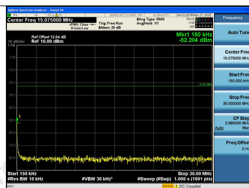
Band26(814-824)-3MHz-16QAM-26705-1RB#14-0 .15~30-PASS
