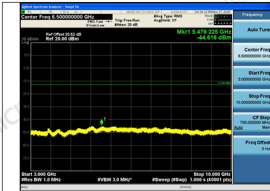
Band26(814-824)-1.4MHz-16QAM-26783-6RB#0-3000~10000-PASS
