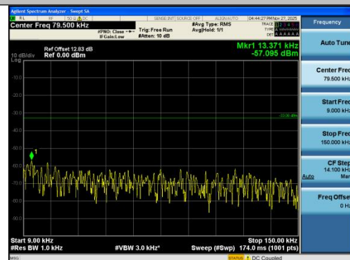
Band26(814-824)-3MHz-QPSK-26740-1RB#0-0.0 09~0.15-PASS
