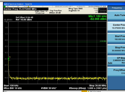
Band26(814-824)-3MHz-16QAM-26705-1RB#0-0.15~30-PASS
