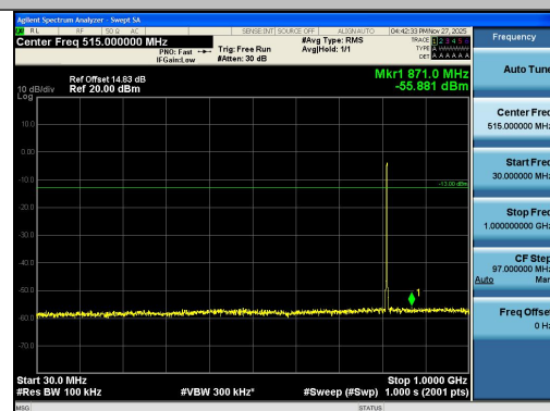
Band26(814-824)-3MHz-QPSK-26705-15RB#0-30 ~1000-PASS
