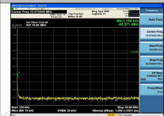
Band26(814-824)-1.4MHz-16QAM-26783-6RB#0- 0.15~30-PASS
