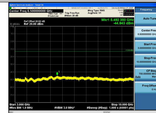
Band26(814-824)-3MHz-QPSK-26705-1RB#14-30 00~10000-PASS
