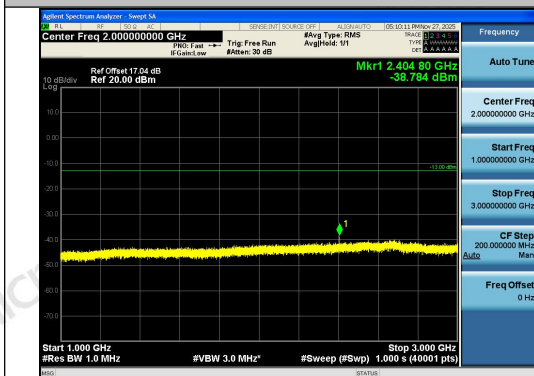
Band26(814-824)-5MHz-QPSK-26740-1RB#24-10 00~3000-PASS
