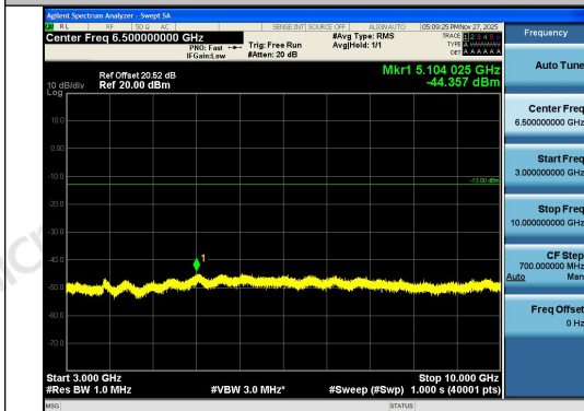
Band26(814-824)-5MHz-16QAM-26740-1RB#0-30 00~10000-PASS
