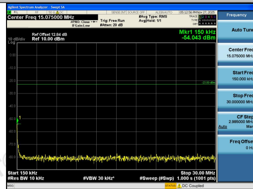
Band26(814-824)-5MHz-16QAM-26740-25RB#0-0 .15~30-PASS
