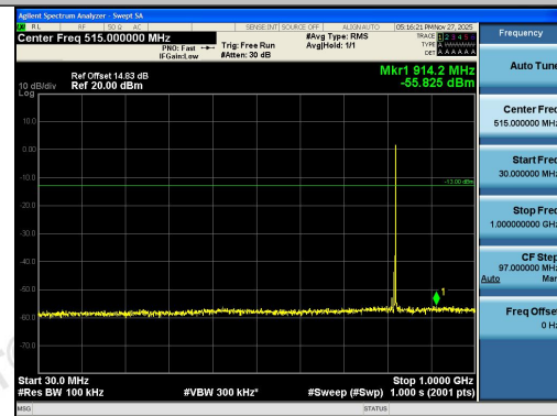
Band26(814-824)-5MHz-QPSK-26765-1RB#24-30 ~1000-PASS
