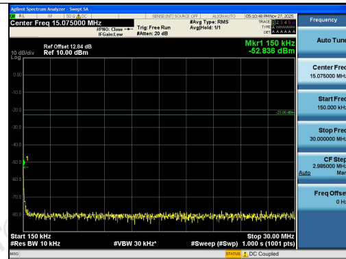
Band26(814-824)-5MHz-16QAM-26740-1RB#24-0 .15~30-PASS
