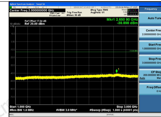
Band26(814-824)-5MHz-16QAM-26740-1RB#0-10 00~3000-PASS
