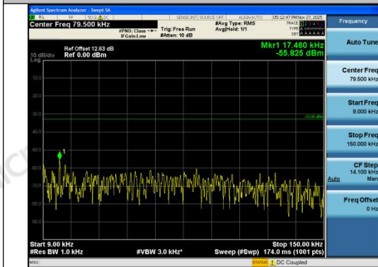
Band26(814-824)-5MHz-16QAM-26740-25RB#0-0 .009~0.15-PASS
