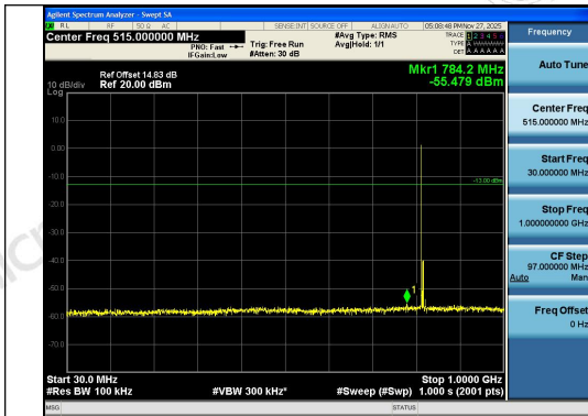
Band26(814-824)-5MHz-16QAM-26740-1RB#0-30 ~1000-PASS
