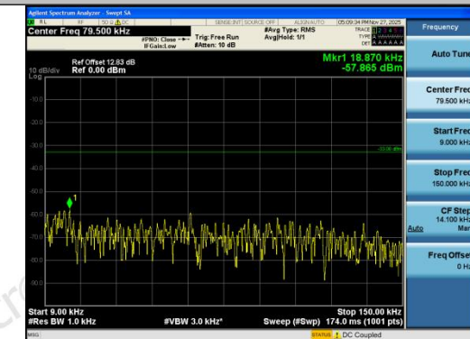
Band26(814-824)-5MHz-QPSK-26740-1RB#24-0. 009~0.15-PASS
