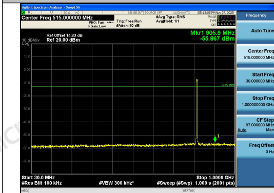
Band26(814-824)-5MHz-16QAM-26740-25RB#0-3 0~1000-PASS
