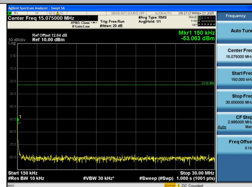
Band26(814-824)-5MHz-16QAM-26765-1RB#24-0 .15~30-PASS
