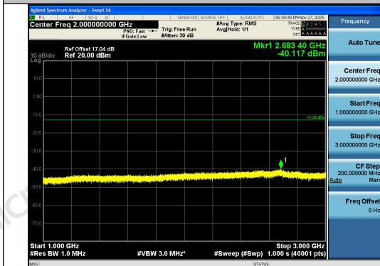
Band26(814-824)-5MHz-QPSK-26765-25RB#0-10 00~3000-PASS
