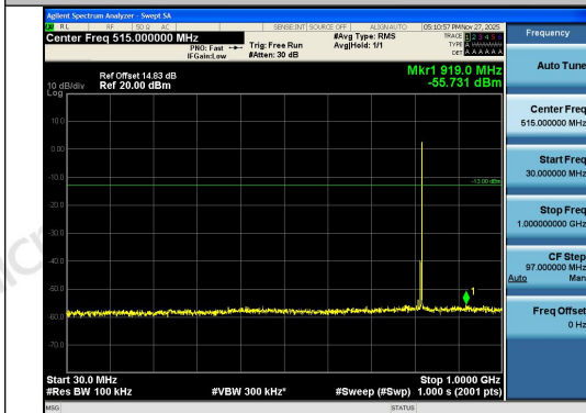
Band26(814-824)-5MHz-16QAM-26740-1RB#24-3 0~1000-PASS
