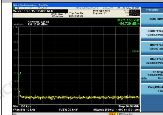
Band26(814-824)-5MHz-QPSK-26740-25RB#0-0. 15~30-PASS
