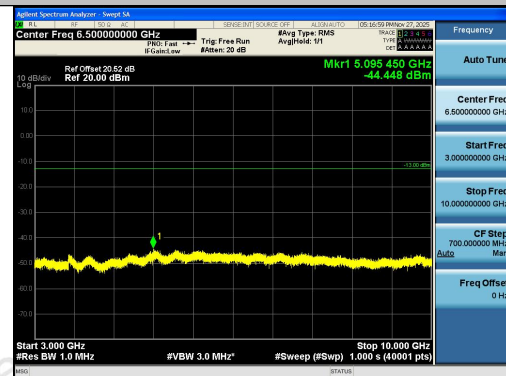
Band26(814-824)-5MHz-QPSK-26765-1RB#24-30 00~10000-PASS
