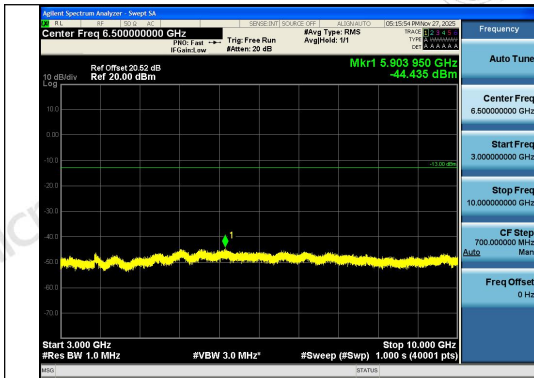
Band26(814-824)-5MHz-16QAM-26765-1RB#0-30 00~10000-PASS
