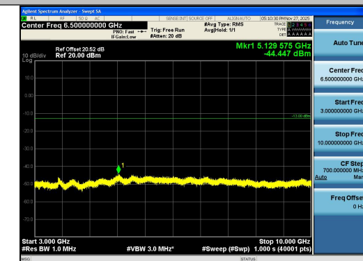
Band26(814-824)-5MHz-QPSK-26740-1RB#24-30 00~10000-PASS
