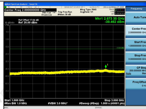
Band26(814-824)-5MHz-16QAM-26740-1RB#24-1 000~3000-PASS
