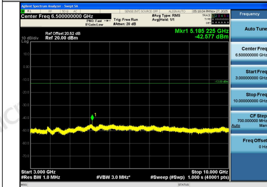
Band26(814-824)-5MHz-16QAM-26765-1RB#24-3 000~10000-PASS
