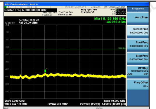
Band26(814-824)-5MHz-QPSK-26765-25RB#0-30 00~10000-PASS
