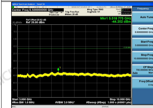
Band26(814-824)-5MHz-16QAM-26740-1RB#24-3 000~10000-PASS
