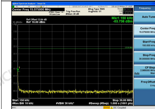
Band26(814-824)-5MHz-QPSK-26765-25RB#0-0. 15~30-PASS
