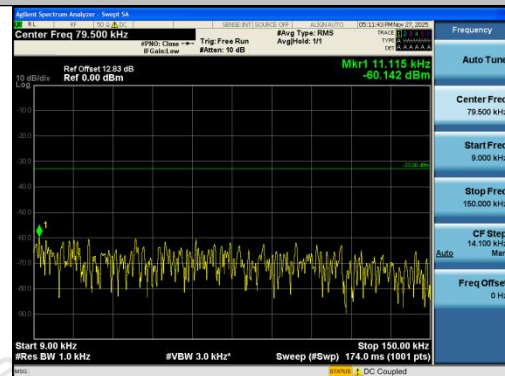
Band26(814-824)-5MHz-QPSK-26740-25RB#0-0. 009~0.15-PASS
