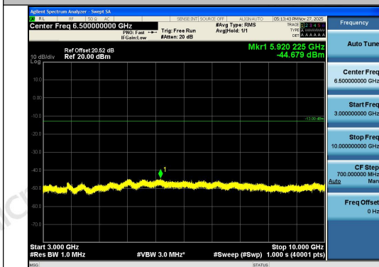
Band26(814-824)-5MHz-16QAM-26740-25RB#0-3 000~10000-PASS
