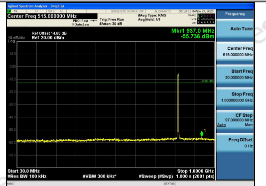
Band26(814-824)-5MHz-QPSK-26765-25RB#0-30 ~1000-PASS
