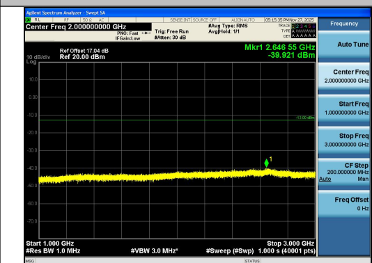
Band26(814-824)-5MHz-16QAM-26765-1RB#0-10 00~3000-PASS
