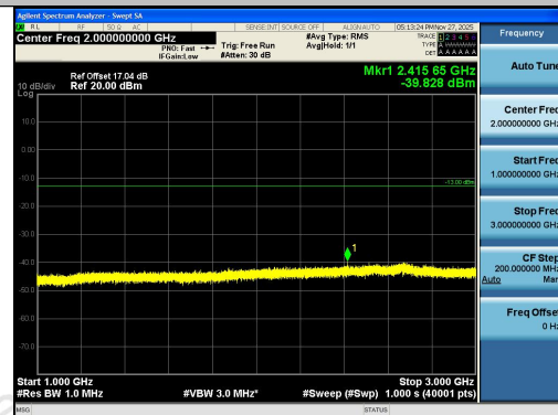
Band26(814-824)-5MHz-16QAM-26740-25RB#0-1 000~3000-PASS
