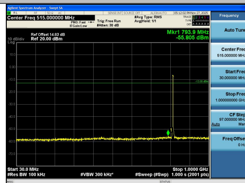
Band26(814-824)-5MHz-QPSK-26740-25RB#0-30 ~1000-PASS
