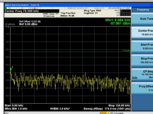
Band26(814-824)-5MHz-QPSK-26765-1RB#0-0.0 09~0.15-PASS
