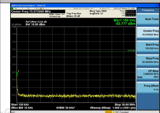
Band26(814-824)-5MHz-16QAM-26765-1RB#0-0. 15~30-PASS
