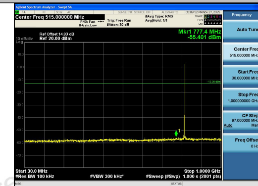
Band26(814-824)-5MHz-QPSK-26740-1RB#24-30 ~1000-PASS
