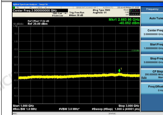
Band26(814-824)-5MHz-QPSK-26765-1RB#24-10 00~3000-PASS
