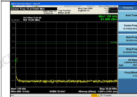
Band26(814-824)-5MHz-QPSK-26765-1RB#24-0. 15~30-PASS
