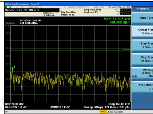
Band26(814-824)-5MHz-QPSK-26765-1RB#24-0. 009~0.15-PASS
