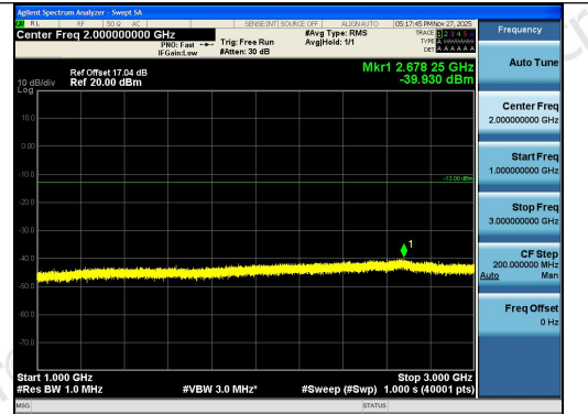
Band26(814-824)-5MHz-16QAM-26765-1RB#24-1 000~3000-PASS
