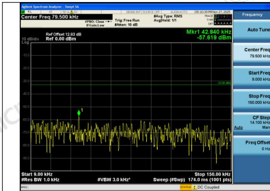
Band26(814-824)-5MHz-16QAM-26740-1RB#24-0 009~0.15-PASS
