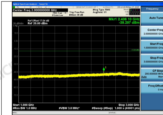
Band26(814-824)-5MHz-QPSK-26740-25RB#0-10 00~3000-PASS
