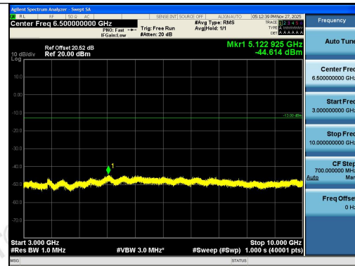
Band26(814-824)-5MHz-QPSK-26740-25RB#0-30 00~10000-PASS
