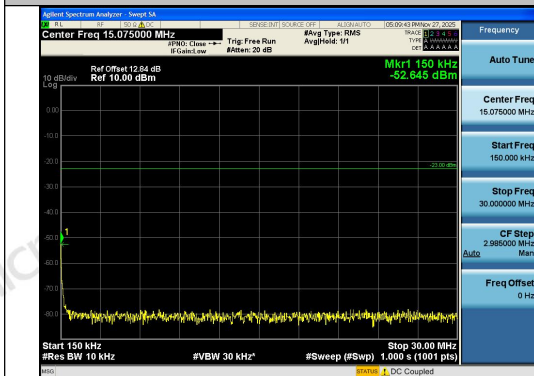
Band26(814-824)-5MHz-QPSK-26740-1RB#24-0. 15~30-PASS
