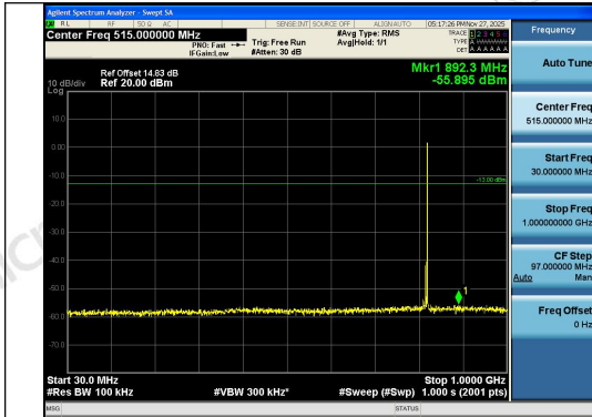
Band26(814-824)-5MHz-16QAM-26765-1RB#24-3 0~1000-PASS
