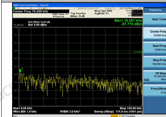
Band26(814-824)-5MHz-16QAM-26765-1RB#24-0 .009~0.15-PASS
