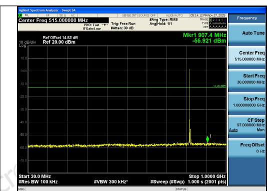
Band26(814-824)-5MHz-QPSK-26765-1RB#0-30~ 1000-PASS
