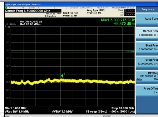
Band26(814-824)-10MHz-QPSK-26740-50RB#0-3 000~10000-PASS
