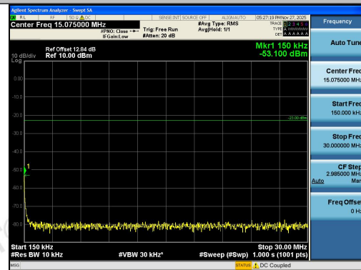
Band26(814-824)-10MHz-16QAM-26740-1RB#0-0 .15~30-PASS
