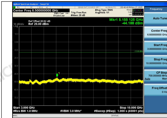
Band26(824-849)-1.4MHz-16QAM-26797-1RB#0- 3000~10000-PASS
