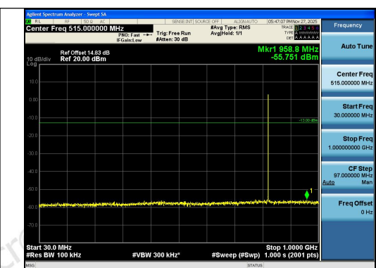
Band26(824-849)-1.4MHz-QPSK-26797-1RB#0-3 0~1000-PASS
