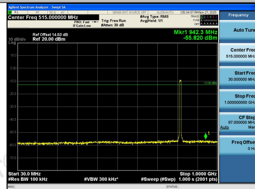
Band26(814-824)-10MHz-QPSK-26740-50RB#0-3 0~1000-PASS
