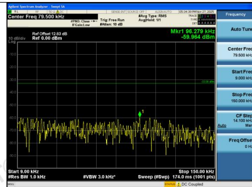
Band26(814-824)-10MHz-QPSK-26740-50RB#0-0 .009~0.15-PASS
