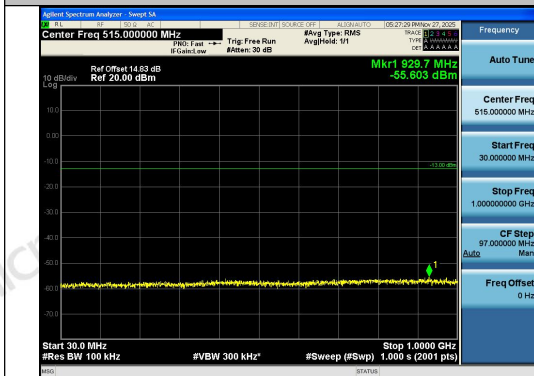
Band26(814-824)-10MHz-16QAM-26740-1RB#0-3 0~1000-PASS
