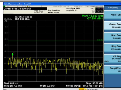
Band26(814-824)-10MHz-QPSK-26740-1RB#49-0 .009~0.15-PASS
