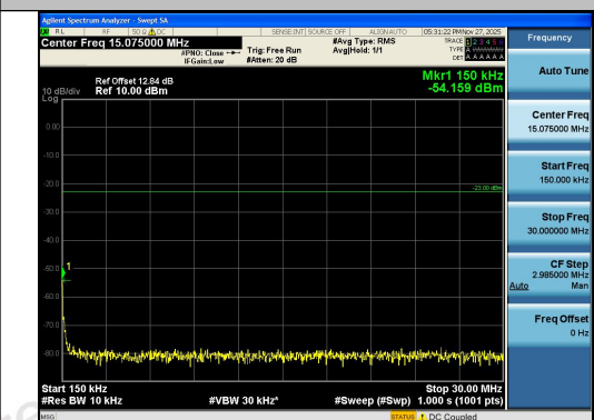
Band26(814-824)-10MHz-16QAM-26740-1RB#49- 0.15~30-PASS
