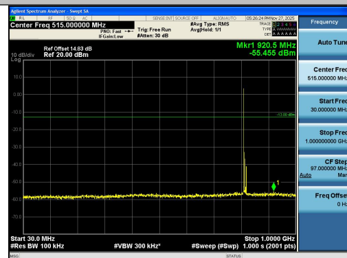
Band26(814-824)-10MHz-QPSK-26740-1RB#0-30 ~1000-PASS
