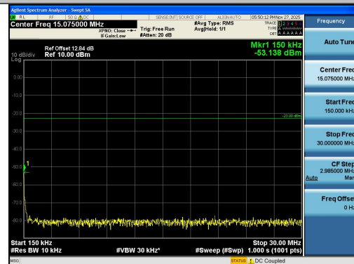
Band26(824-849)-1.4MHz-16QAM-26797-1RB#5- 0.15~30-PASS
