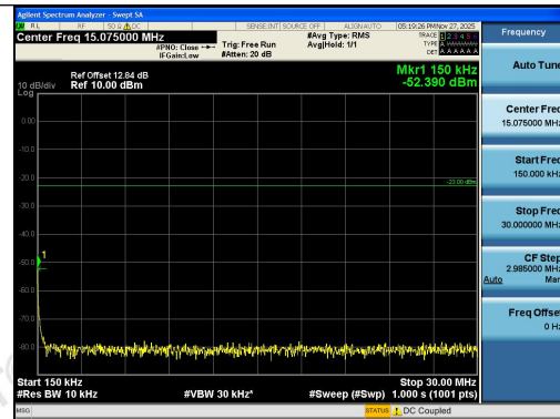
Band26(814-824)-5MHz-16QAM-26765-25RB#0-0 .15~30-PASS
