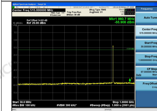
Band26(814-824)-5MHz-16QAM-26765-25RB#0-3 0~1000-PASS
