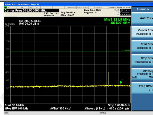
Band26(824-849)-1.4MHz-QPSK-26797-1RB#5-3 0~1000-PASS
