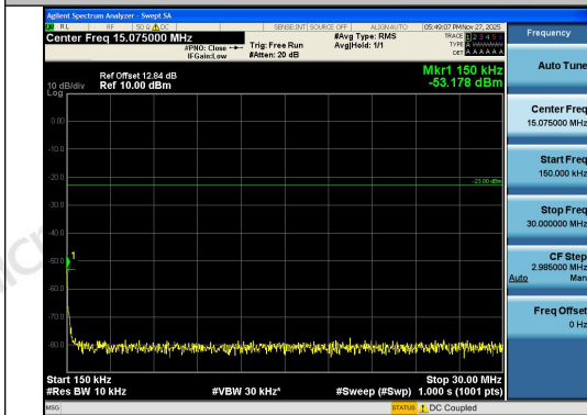
Band26(824-849)-1.4MHz-QPSK-26797-1RB#5-0. 15~30-PASS
