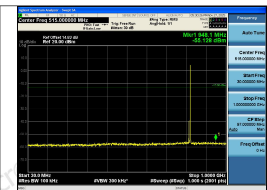
Band26(814-824)-10MHz-QPSK-26740-1RB#49-3 0~1000-PASS
