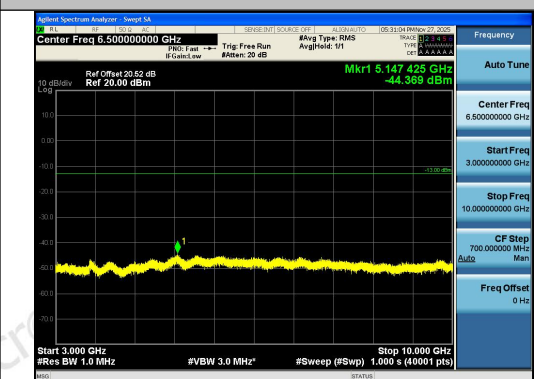
Band26(814-824)-10MHz-QPSK-26740-1RB#49-3 000~10000-PASS
