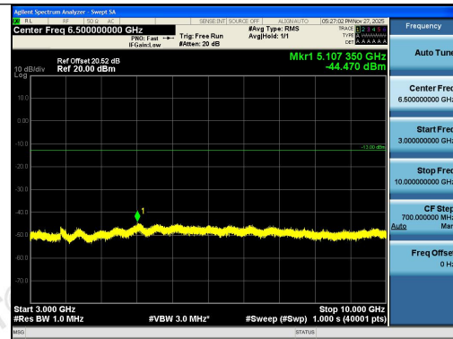
Band26(814-824)-10MHz-QPSK-26740-1RB#0-30 00~10000-PASS
