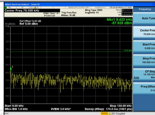
Band26(814-824)-10MHz-QPSK-26740-1RB#0-0. 009~0.15-PASS
