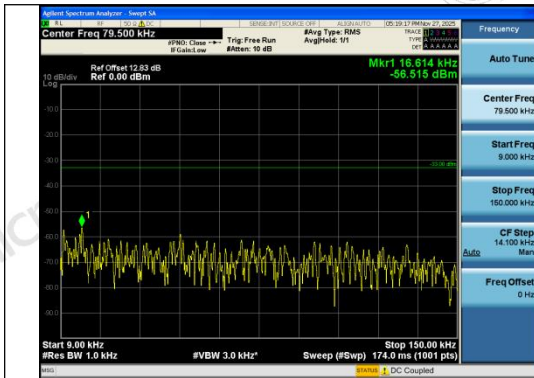
Band26(814-824)-5MHz-16QAM-26765-25RB#0-0 009~0.15-PASS
