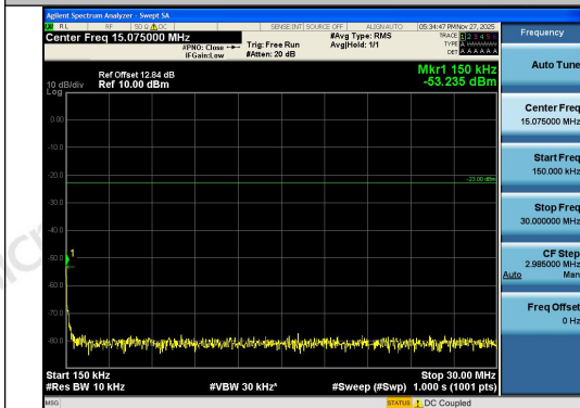
Band26(814-824)-10MHz-QPSK-26740-50RB#0-0 .15~30-PASS
