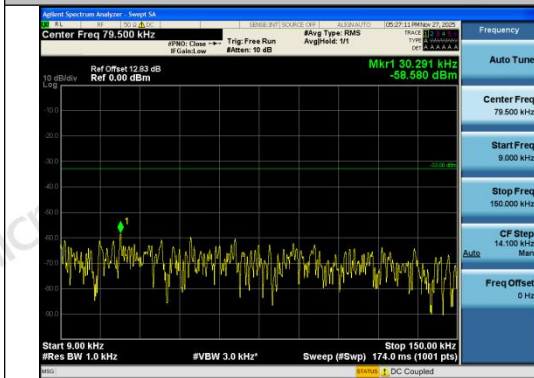
Band26(814-824)-10MHz-16QAM-26740-1RB#0-0 .009~0.15-PASS
