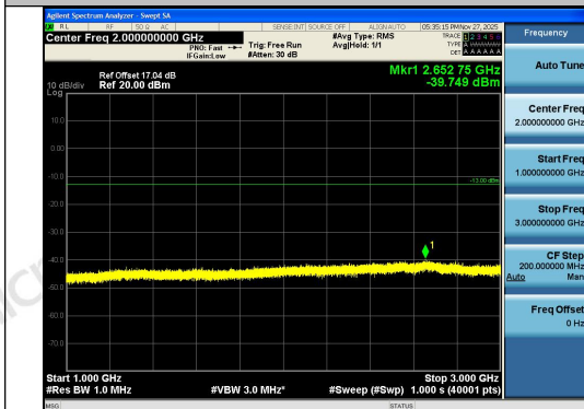
Band26(814-824)-10MHz-QPSK-26740-50RB#0-1 000~3000-PASS
