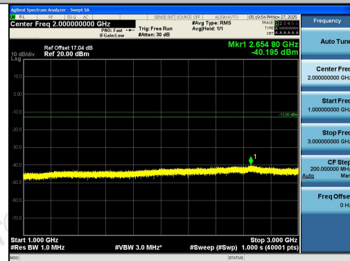
Band26(814-824)-5MHz-16QAM-26765-25RB#0-1 000~3000-PASS
