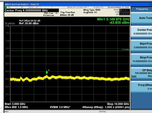
Band26(824-849)-1.4MHz-QPSK-26797-1RB#5-3 000~10000-PASS
