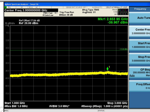
Band26(814-824)-10MHz-16QAM-26740-1RB#0-1 000~3000-PASS
