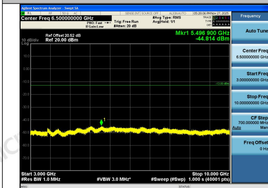
Band26(814-824)-10MHz-16QAM-26740-1RB#0-3 000~10000-PASS
