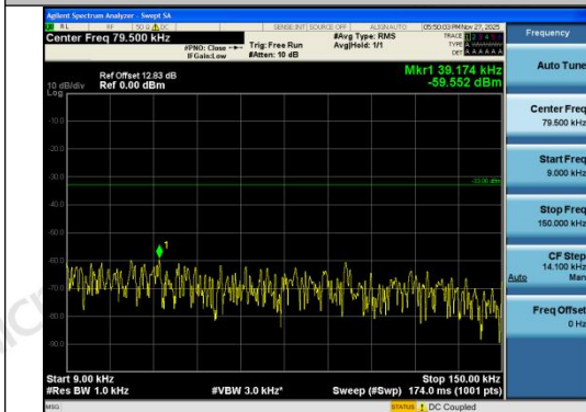
Band26(824-849)-1.4MHz-16QAM-26797-1RB#5- 0.009~0.15-PASS
