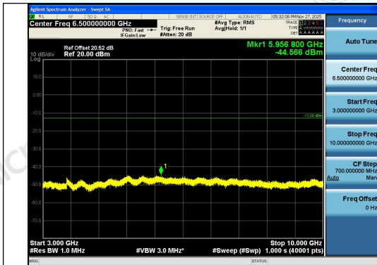
Band26(814-824)-10MHz-16QAM-26740-1RB#49- 3000~10000-PASS
