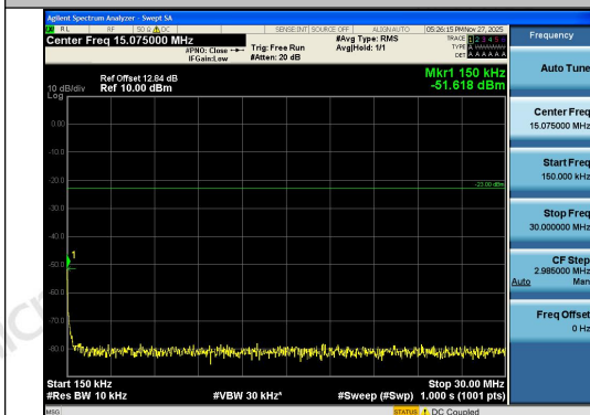
Band26(814-824)-10MHz-QPSK-26740-1RB#0-0. 15~30-PASS
