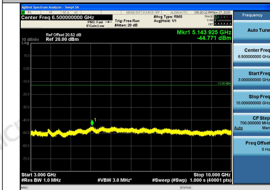
Band26(814-824)-5MHz-16QAM-26765-25RB#0-3 000~10000-PASS
