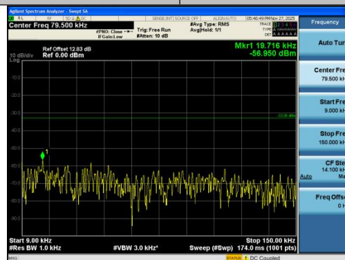
Band26(824-849)-1.4MHz-QPSK-26797-1RB#0-0.009~0.15-PASS
