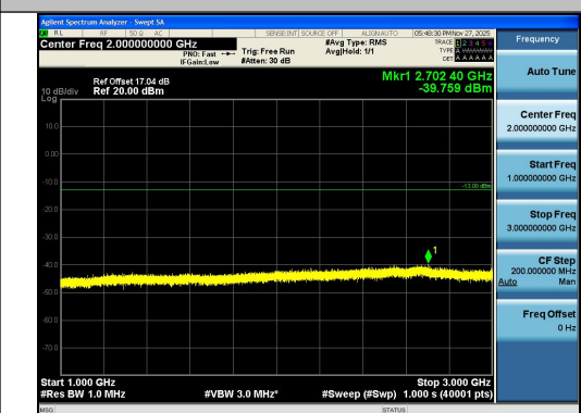
Band26(824-849)-1.4MHz-16QAM-26797-1RB#0- 1000~3000-PASS
