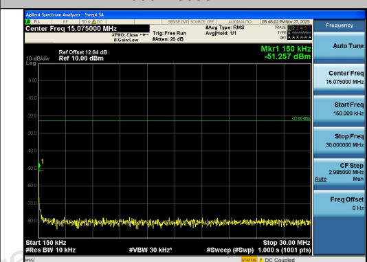
Band26(824-849)-1.4MHz-16QAM-26797-1RB#0- 0.15~30-PASS
