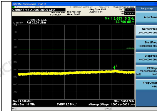
Band26(814-824)-10MHz-QPSK-26740-1RB#0-10 00~3000-PASS
