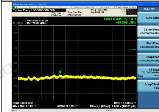
Band26(824-849)-1.4MHz-16QAM-26797-1RB#5- 3000~10000-PASS
