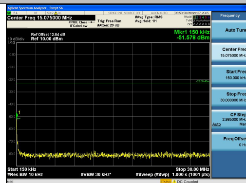
Band26(824-849)-1.4MHz-16QAM-26915-6RB#0- 0.15~30-PASS
