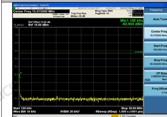
Band26(824-849)-1.4MHz-QPSK-26915-1RB#0-0. 15~30-PASS
