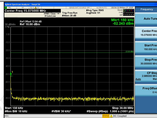
Band26(824-849)-1.4MHz-16QAM-26915-1RB#0- 0.15~30-PASS
