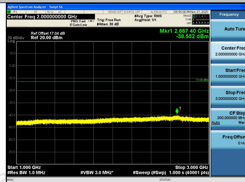
Band26(824-849)-1.4MHz-16QAM-26915-1RB#0- 1000~3000-PASS
