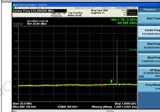
Band26(824-849)-1.4MHz-16QAM-26915-1RB#5- 30~1000-PASS
