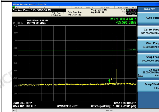
Band26(824-849)-1.4MHz-16QAM-26915-1RB#0- 30~1000-PASS
