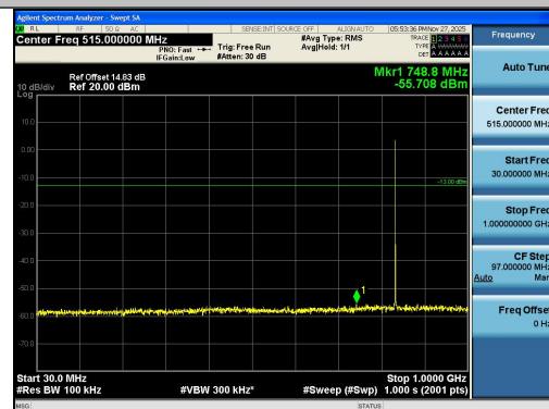
Band26(824-849)-1.4MHz-QPSK-26915-1RB#0-3 0~1000-PASS
