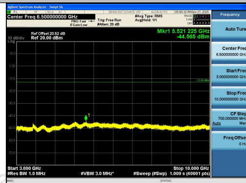
Band26(824-849)-1.4MHz-QPSK-26915-6RB#0-3 000~10000-PASS
