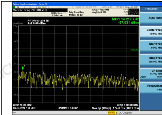
Band26(824-849)-1.4MHz-16QAM-26797-6RB#0- 0.009~0.15-PASS
