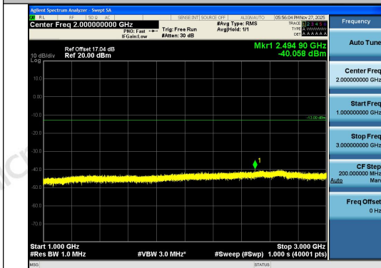
Band26(824-849)-1.4MHz-QPSK-26915-1RB#5-1 000~3000-PASS
