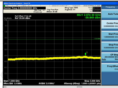
Band26(824-849)-1.4MHz-16QAM-26797-6RB#0- 1000~3000-PASS
