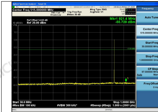
Band26(824-849)-1.4MHz-16QAM-26797-1RB#5- 30~1000-PASS
