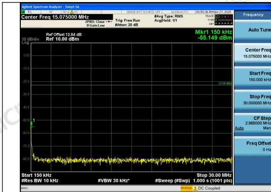
Band26(824-849)-1.4MHz-QPSK-26915-1RB#5-0. 15~30-PASS
