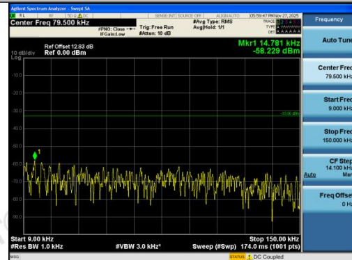
Band26(824-849)-1.4MHz-QPSK-27033-1RB#0-0.009~0.15-PASS
