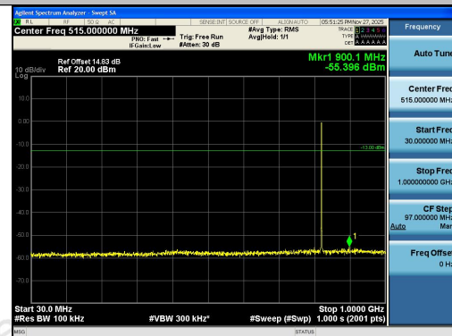
Band26(824-849)-1.4MHz-QPSK-26797-6RB#0-3 0~1000-PASS
