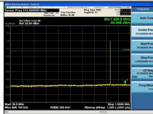
Band26(824-849)-1.4MHz-QPSK-26915-6RB#0-3 0~1000-PASS
