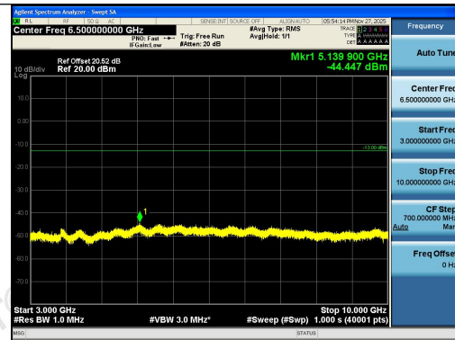
Band26(824-849)-1.4MHz-QPSK-26915-1RB#0-3 000~10000-PASS
