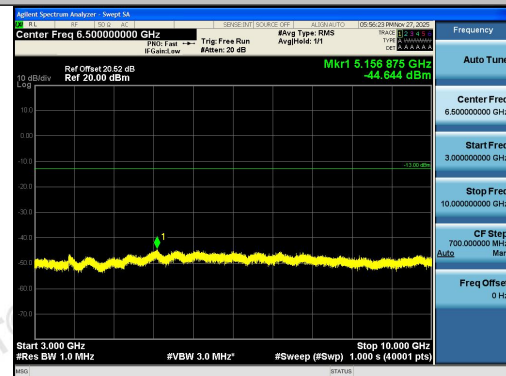
Band26(824-849)-1.4MHz-QPSK-26915-1RB#5-3 000~10000-PASS
