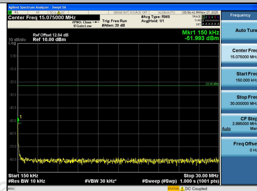
Band26(824-849)-1.4MHz-16QAM-26915-1RB#5- 0.15~30-PASS
