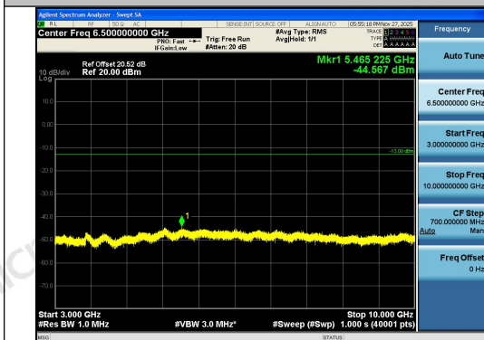
Band26(824-849)-1.4MHz-16QAM-26915-1RB#0- 3000~10000-PASS
