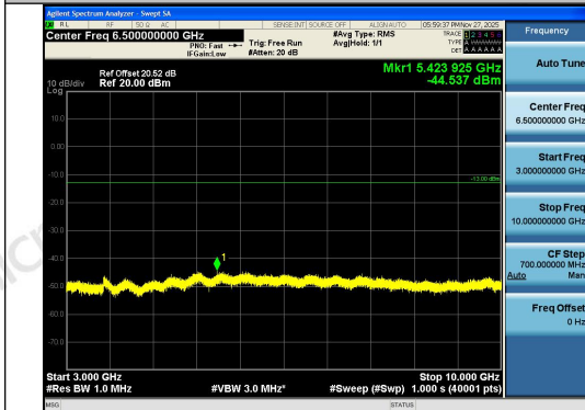
Band26(824-849)-1.4MHz-16QAM-26915-6RB#0-3000~10000-PASS
