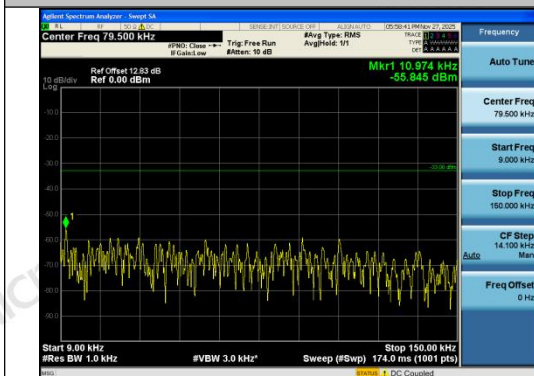
Band26(824-849)-1.4MHz-16QAM-26915-6RB#0- 0.009~0.15-PASS
