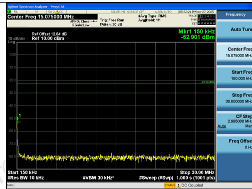
Band26(824-849)-1.4MHz-16QAM-26797-6RB#0- 0.15~30-PASS
