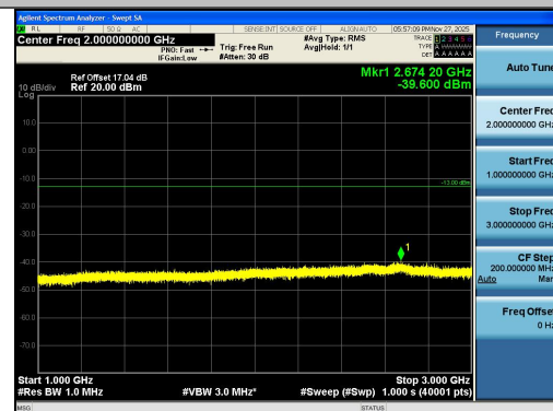
Band26(824-849)-1.4MHz-16QAM-26915-1RB#5- 1000~3000-PASS
