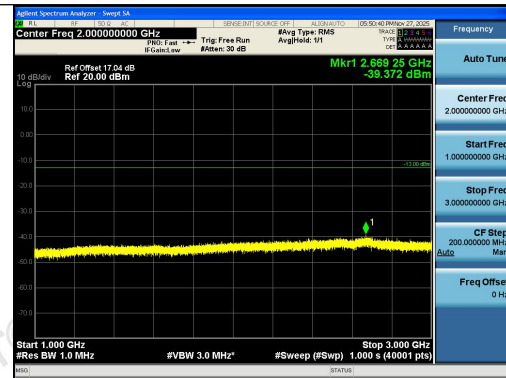
Band26(824-849)-1.4MHz-16QAM-26797-1RB#5- 1000~3000-PASS
