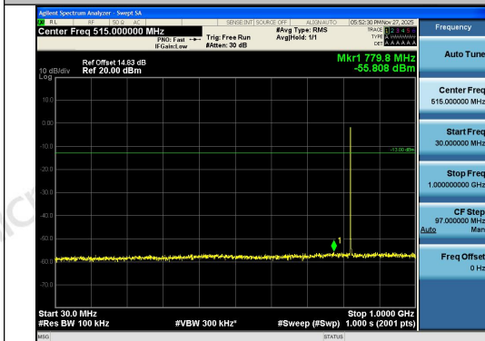
Band26(824-849)-1.4MHz-16QAM-26797-6RB#0- 30~1000-PASS
