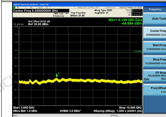
Band26(824-849)-1.4MHz-16QAM-26797-6RB#0- 3000~10000-PASS
