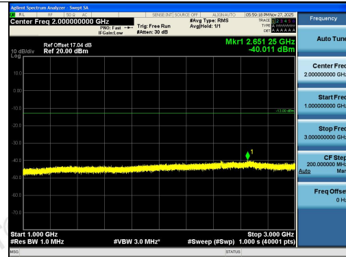
Band26(824-849)-1.4MHz-16QAM-26915-6RB#0-1000~3000-PASS
