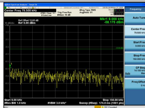
Band26(824-849)-1.4MHz-QPSK-26915-1RB#5-0. 009~0.15-PASS
