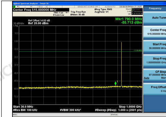
Band26(824-849)-1.4MHz-16QAM-26915-6RB#0-30~1000-PASS
