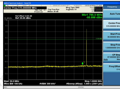
Band26(824-849)-1.4MHz-QPSK-26915-1RB#5-3 0~1000-PASS
