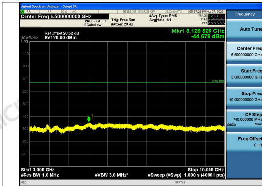
Band26(824-849)-1.4MHz-16QAM-26915-1RB#5- 3000~10000-PASS
