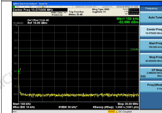
Band26(824-849)-1.4MHz-QPSK-27033-1RB#0-0.15~30-PASS
