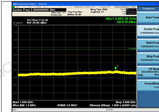
Band26(824-849)-1.4MHz-QPSK-26915-1RB#0-1 000~3000-PASS
