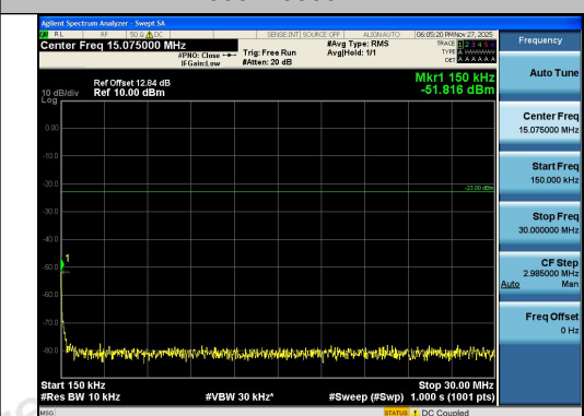
Band26(824-849)-1.4MHz-16QAM-27033-6RB#0- 0.15~30-PASS
