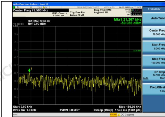
Band26(824-849)-3MHz-16QAM-26805-1RB#14-0 009~0.15-PASS
