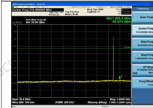
Band26(824-849)-1.4MHz-16QAM-27033-1RB#0- 30~1000-PASS
