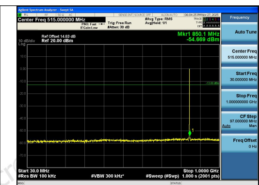
Band26(824-849)-1.4MHz-QPSK-27033-6RB#0-3 0~1000-PASS
