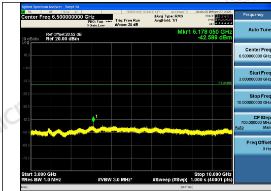
Band26(824-849)-1.4MHz-16QAM-27033-6RB#0-3000~10000-PASS
