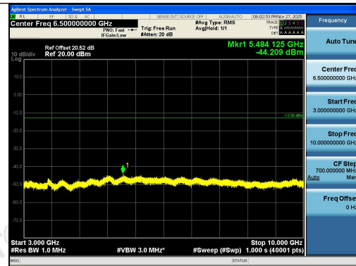
Band26(824-849)-1.4MHz-QPSK-27033-1RB#5-3 000~10000-PASS
