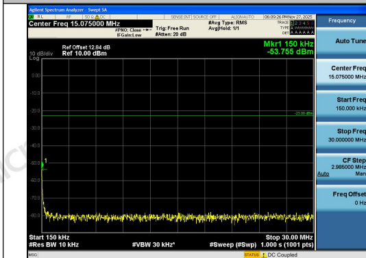
Band26(824-849)-3MHz-QPSK-26805-1RB#0-0.15~0.30-PASS
