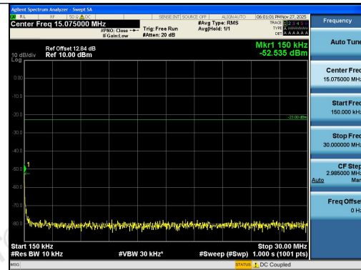
Band26(824-849)-1.4MHz-16QAM-27033-1RB#0- 0.15~30-PASS
