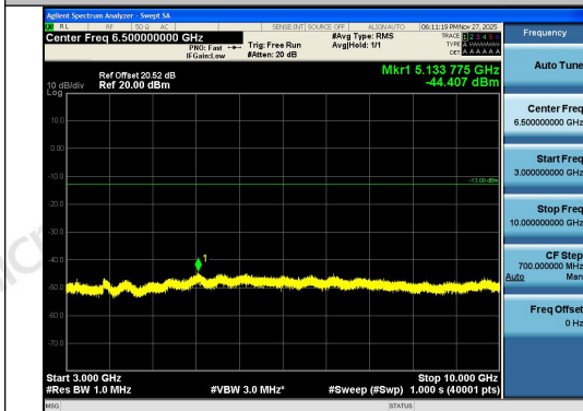
Band26(824-849)-3MHz-16QAM-26805-1RB#0-30 00~10000-PASS
