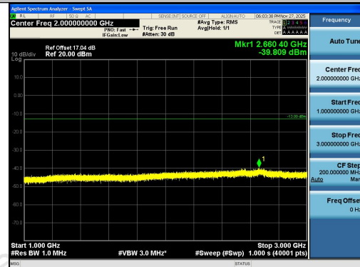
Band26(824-849)-1.4MHz-16QAM-27033-1RB#5- 1000~3000-PASS
