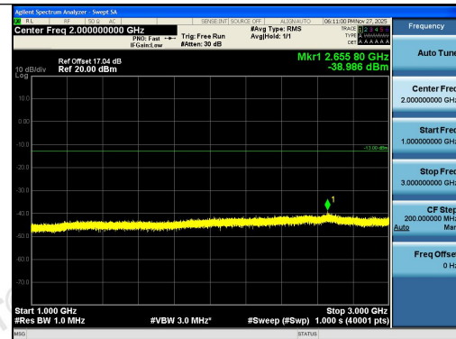
Band26(824-849)-3MHz-16QAM-26805-1RB#0-10 00~3000-PASS
