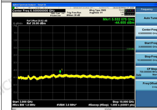
Band26(824-849)-1.4MHz-16QAM-27033-1RB#5- 3000~10000-PASS
