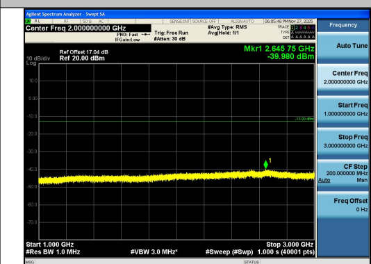
Band26(824-849)-1.4MHz-16QAM-27033-6RB#0- 1000~3000-PASS
