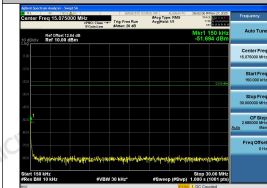
Band26(824-849)-1.4MHz-QPSK-27033-1RB#5-0. 15~30-PASS
