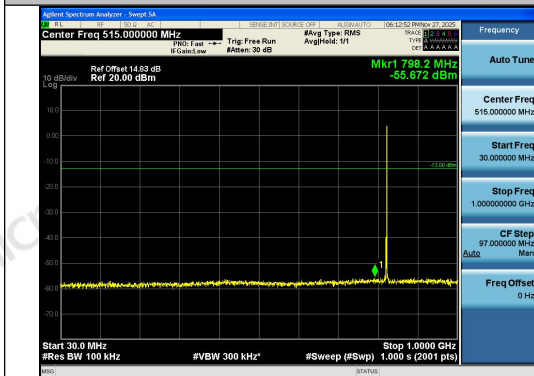
Band26(824-849)-3MHz-16QAM-26805-1RB#14-3 0~1000-PASS
