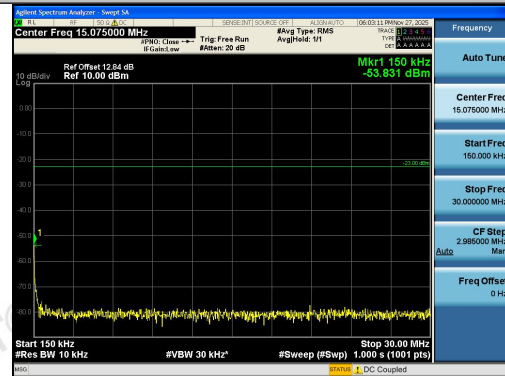
Band26(824-849)-1.4MHz-16QAM-27033-1RB#5- 0.15~30-PASS
