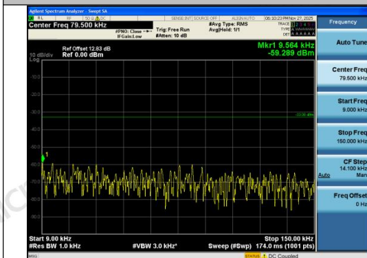
Band26(824-849)-3MHz-16QAM-26805-1RB#0-0.009~0.15-PASS
