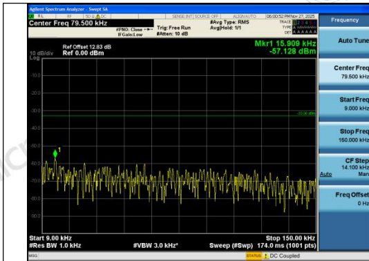
Band26(824-849)-1.4MHz-16QAM-27033-1RB#0- 0.009~0.15-PASS
