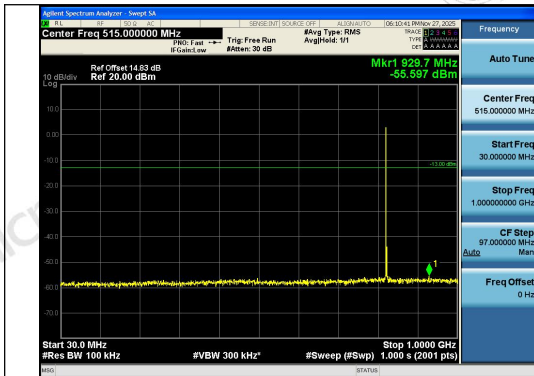
Band26(824-849)-3MHz-16QAM-26805-1RB#0-30 ~1000-PASS
