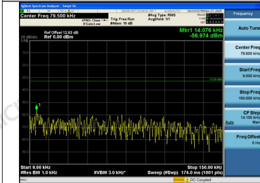
Band26(824-849)-1.4MHz-16QAM-27033-1RB#5- 0.009~0.15-PASS
