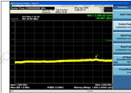
Band26(824-849)-1.4MHz-QPSK-27033-1RB#5-1 000~3000-PASS
