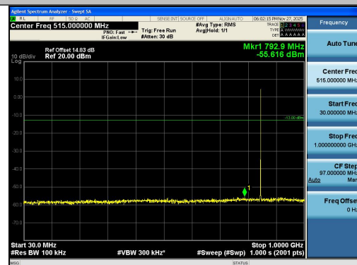
Band26(824-849)-1.4MHz-QPSK-27033-1RB#5-3 0~1000-PASS
