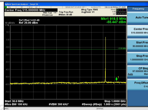
Band26(824-849)-3MHz-QPSK-26805-1RB#14-30 ~1000-PASS
