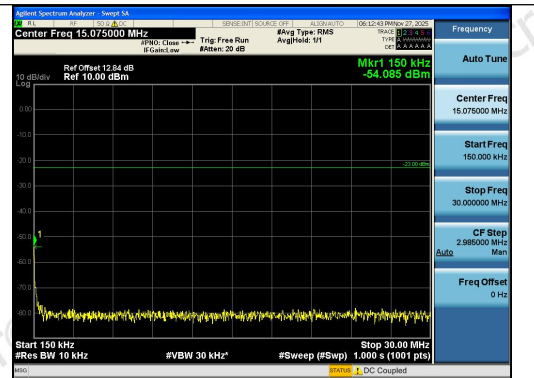
Band26(824-849)-3MHz-16QAM-26805-1RB#14-0 .15~30-PASS
