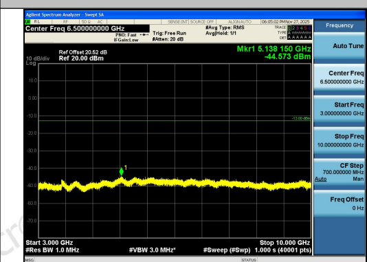
Band26(824-849)-1.4MHz-QPSK-27033-6RB#0-3 000~10000-PASS
