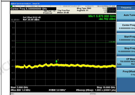
Band26(824-849)-3MHz-16QAM-26805-1RB#14-3 000~10000-PASS
