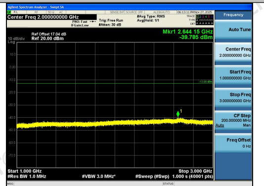
Band26(824-849)-3MHz-16QAM-26805-1RB#14-1 000~3000-PASS
