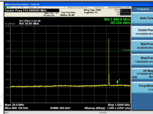
Band26(824-849)-3MHz-QPSK-26805-1RB#0-30~1000-PASS
