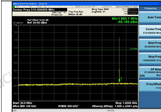
Band26(824-849)-1.4MHz-16QAM-27033-1RB#5- 30~1000-PASS
