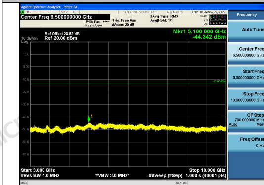
Band26(824-849)-1.4MHz-16QAM-27033-1RB#0- 3000~10000-PASS
