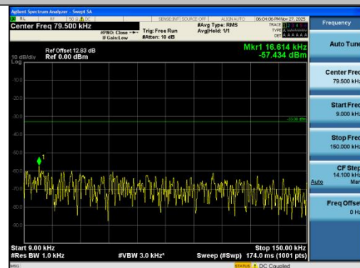
Band26(824-849)-1.4MHz-QPSK-27033-6RB#0-0. 009~0.15-PASS
