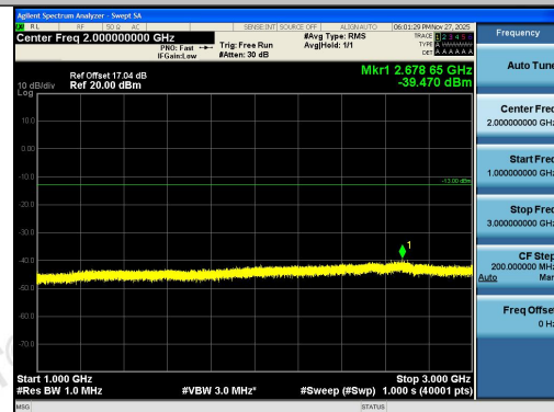
Band26(824-849)-1.4MHz-16QAM-27033-1RB#0- 1000~3000-PASS
