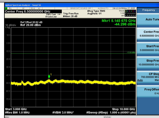
Band26(824-849)-3MHz-QPSK-26805-1RB#14-30 00~10000-PASS
