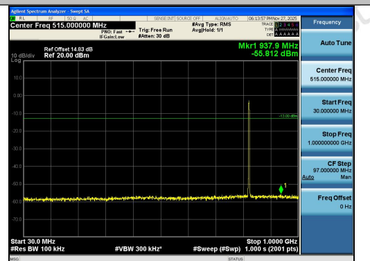
Band26(824-849)-3MHz-QPSK-26805-15RB#0-30 ~1000-PASS
