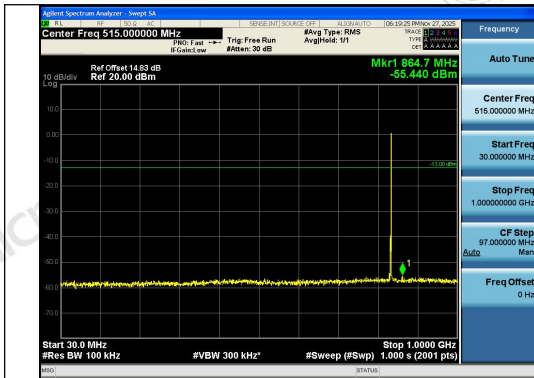
Band26(824-849)-3MHz-16QAM-26915-1RB#14-3 0~1000-PASS
