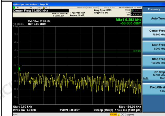
Band26(824-849)-3MHz-16QAM-26915-1RB#14-0 .009~0.15-PASS
