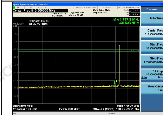
Band26(824-849)-3MHz-16QAM-26915-15RB#0-3 0~1000-PASS
