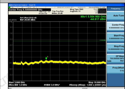
Band26(824-849)-3MHz-QPSK-26915-1RB#0-300 0~10000-PASS
