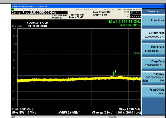
Band26(824-849)-3MHz-16QAM-26915-1RB#0-10 00~3000-PASS
