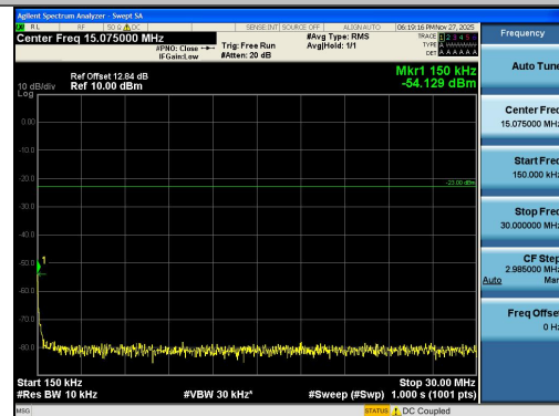
Band26(824-849)-3MHz-16QAM-26915-1RB#14-0 .15~30-PASS
