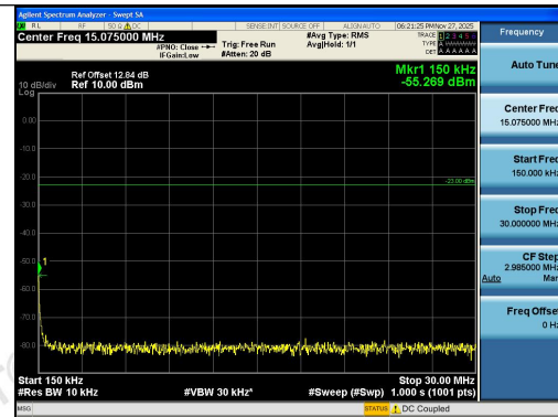
Band26(824-849)-3MHz-16QAM-26915-15RB#0-0 .15~30-PASS
