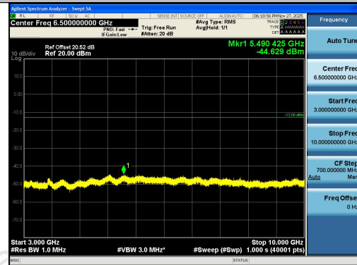
Band26(824-849)-3MHz-QPSK-26915-1RB#14-30 00~10000-PASS
