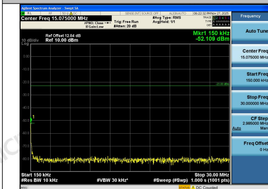
Band26(824-849)-3MHz-QPSK-27025-1RB#0-0.1 5~30-PASS
