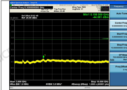
Band26(824-849)-3MHz-16QAM-26915-1RB#0-30 00~10000-PASS
