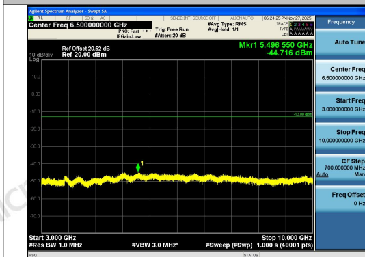
Band26(824-849)-3MHz-16QAM-27025-1RB#0-30 00~10000-PASS
