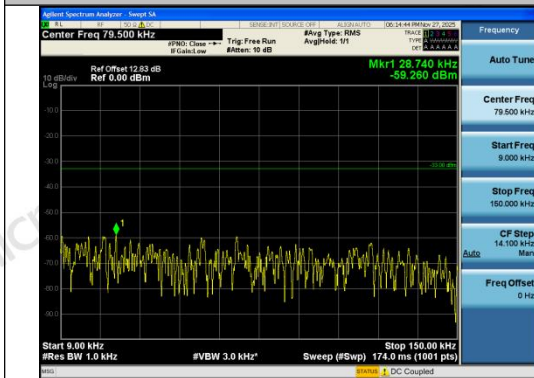
Band26(824-849)-3MHz-16QAM-26805-15RB#0-0 .009~0.15-PASS
