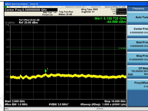
Band26(824-849)-3MHz-QPSK-27025-1RB#0-300 0~10000-PASS
