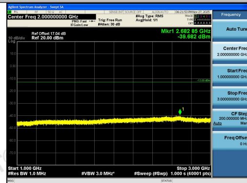
Band26(824-849)-3MHz-16QAM-26915-15RB#0-1 000~3000-PASS
