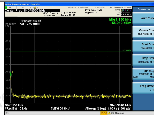
Band26(824-849)-3MHz-16QAM-27025-1RB#0-0. 15~30-PASS
