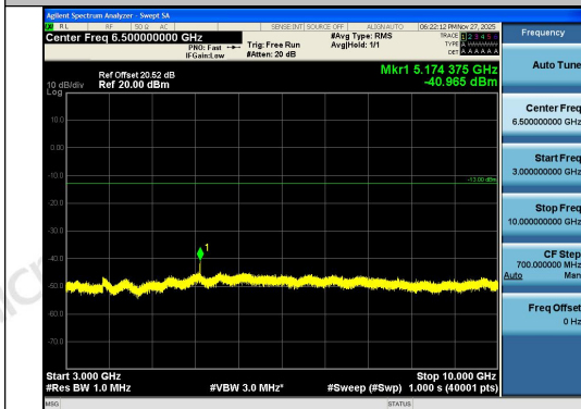
Band26(824-849)-3MHz-16QAM-26915-15RB#0-3 000~10000-PASS
