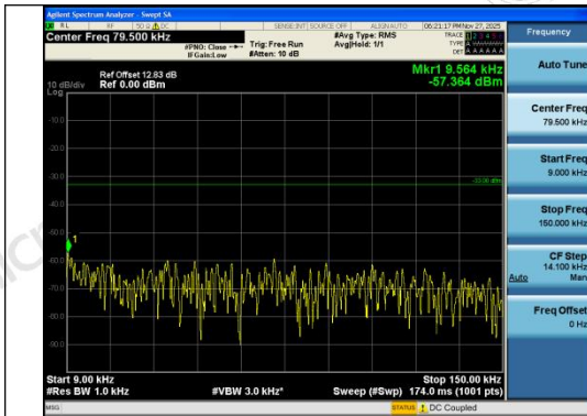
Band26(824-849)-3MHz-16QAM-26915-15RB#0-0 0.009~0.15-PASS
