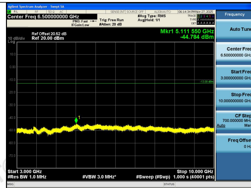
Band26(824-849)-3MHz-QPSK-26805-15RB#0-30 00~10000-PASS
