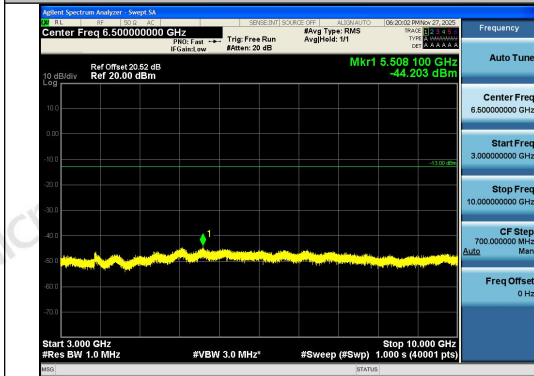
Band26(824-849)-3MHz-16QAM-26915-1RB#14-3 000~10000-PASS
