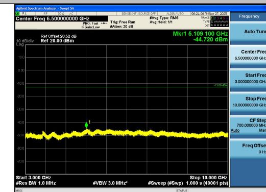
Band26(824-849)-3MHz-QPSK-26915-15RB#0-30 00~10000-PASS
