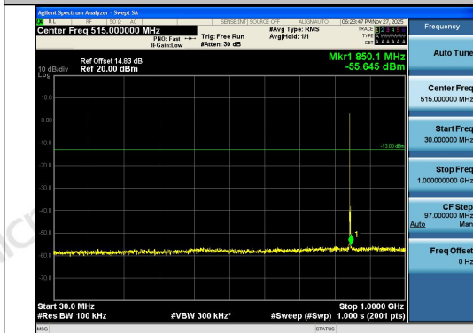
Band26(824-849)-3MHz-16QAM-27025-1RB#0-30 ~1000-PASS
