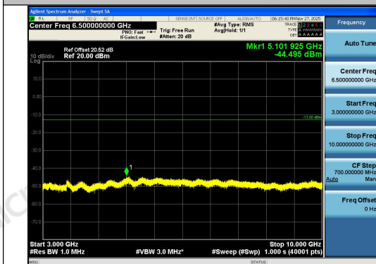
Band26(824-849)-3MHz-16QAM-26805-15RB#0-3 000~10000-PASS
