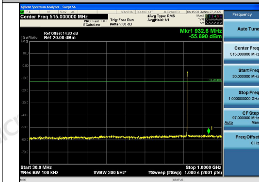
Band26(824-849)-3MHz-16QAM-26805-15RB#0-3 0~1000-PASS
