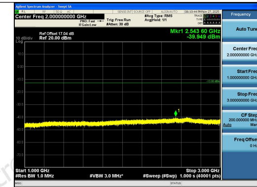
Band26(824-849)-3MHz-16QAM-26915-1RB#14-1 000~3000-PASS
