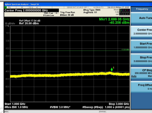
Band26(824-849)-3MHz-16QAM-26805-15RB#0-1 000~3000-PASS
