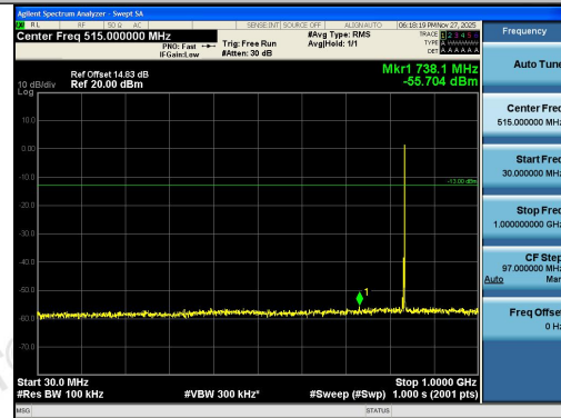
Band26(824-849)-3MHz-QPSK-26915-1RB#14-30 ~1000-PASS
