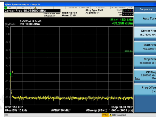
Band26(824-849)-3MHz-16QAM-26805-15RB#0-0 .15~30-PASS
