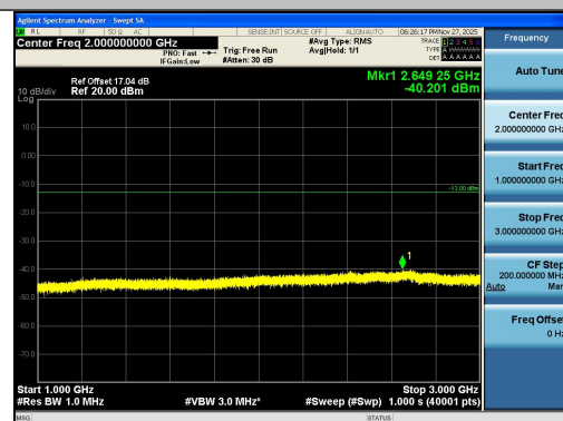
Band26(824-849)-3MHz-16QAM-27025-1RB#14-1 000~3000-PASS
