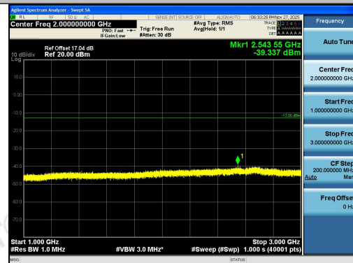
Band26(824-849)-5MHz-16QAM-26815-1RB#0-10 00~3000-PASS
