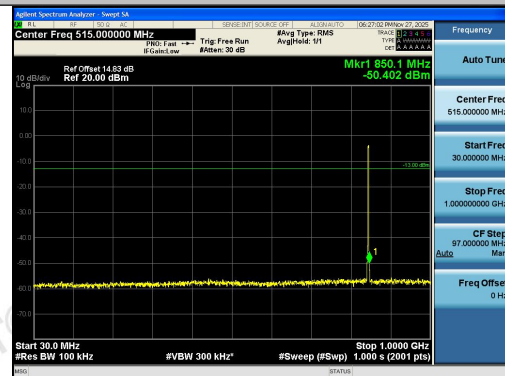
Band26(824-849)-3MHz-QPSK-27025-15RB#0-30 ~1000-PASS
