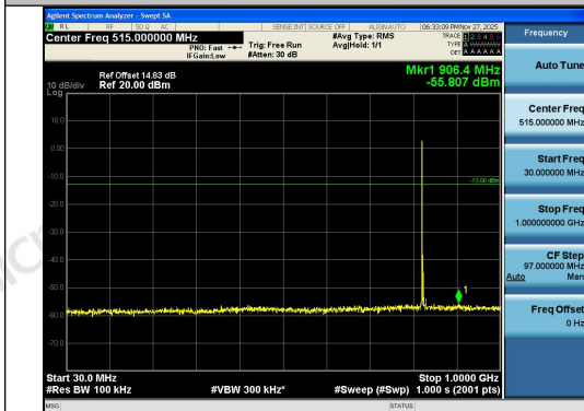
Band26(824-849)-5MHz-16QAM-26815-1RB#0-30 ~1000-PASS
