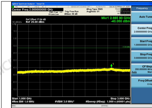
Band26(824-849)-5MHz-QPSK-26815-1RB#24-10 00~3000-PASS
