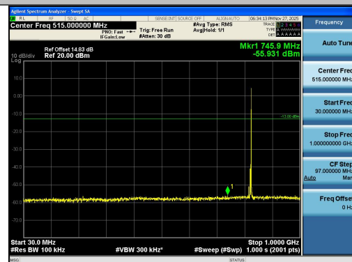
Band26(824-849)-5MHz-QPSK-26815-1RB#24-30 ~1000-PASS
