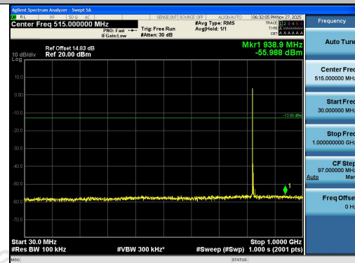
Band26(824-849)-5MHz-QPSK-26815-1RB#0-30~ 1000-PASS
