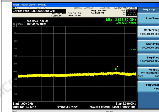
Band26(824-849)-5MHz-QPSK-26815-1RB#0-100 0~3000-PASS
