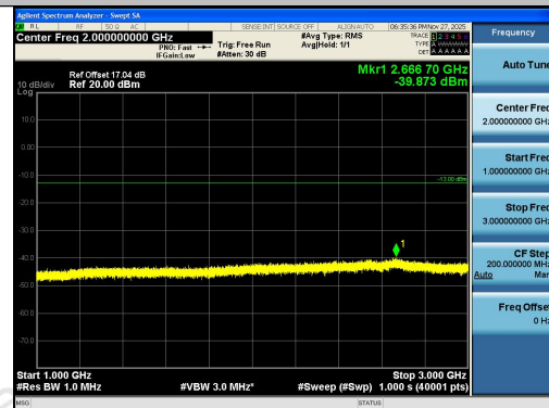
Band26(824-849)-5MHz-16QAM-26815-1RB#24-1 000~3000-PASS
