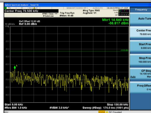
Band26(824-849)-5MHz-QPSK-26815-25RB#0-0. 009~0.15-PASS
