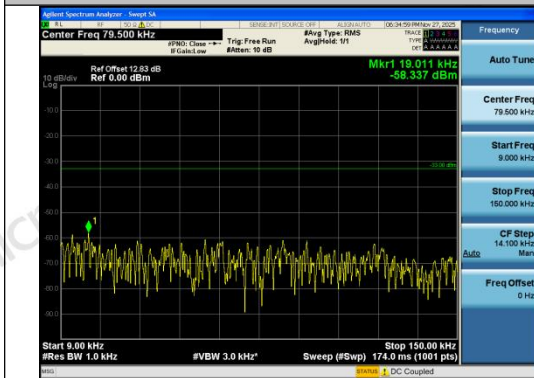
Band26(824-849)-5MHz-16QAM-26815-1RB#24-0 .009~0.15-PASS
