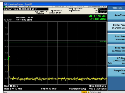
Band26(824-849)-3MHz-16QAM-27025-15RB#0-0 .15~30-PASS
