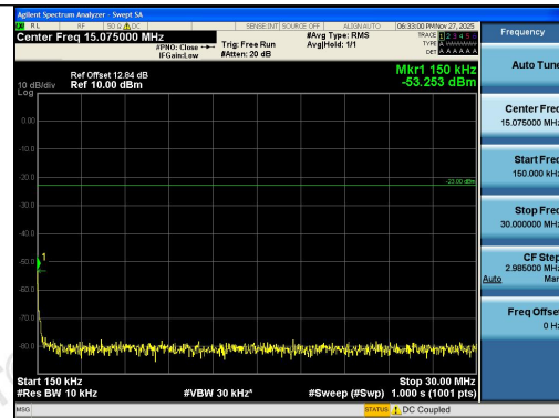
Band26(824-849)-5MHz-16QAM-26815-1RB#0-0. 15~30-PASS
