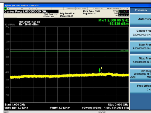
Band26(824-849)-5MHz-16QAM-26815-25RB#0-1 000~3000-PASS
