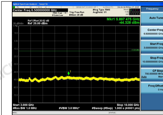
Band26(824-849)-3MHz-16QAM-27025-1RB#14-3 000~10000-PASS
