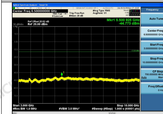
Band26(824-849)-5MHz-16QAM-26815-1RB#24-3 000~10000-PASS
