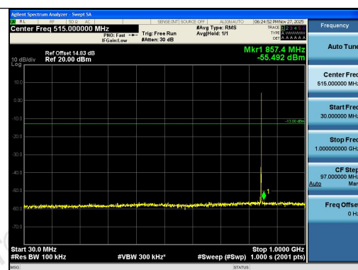
Band26(824-849)-3MHz-QPSK-27025-1RB#14-30 ~1000-PASS
