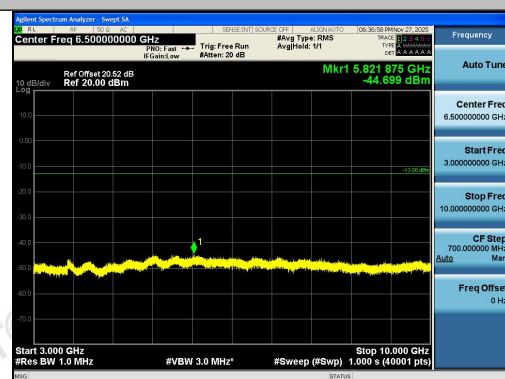
Band26(824-849)-5MHz-QPSK-26815-25RB#0-30 00~10000-PASS
