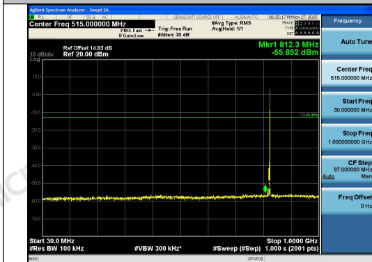
Band26(824-849)-5MHz-16QAM-26815-1RB#24-3 0~1000-PASS
