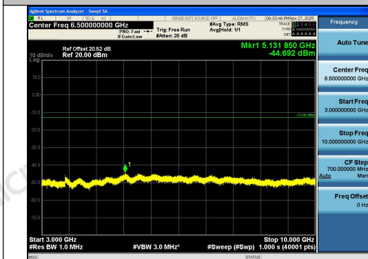
Band26(824-849)-5MHz-16QAM-26815-1RB#0-30 00~10000-PASS
