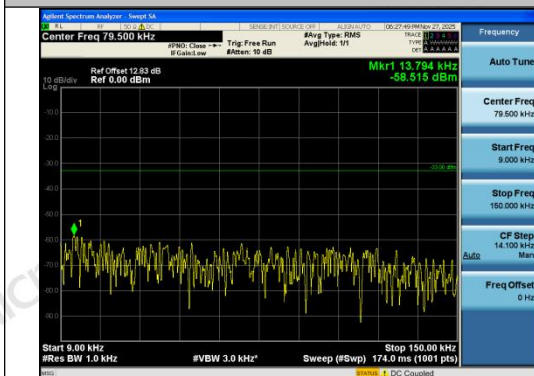
Band26(824-849)-3MHz-16QAM-27025-15RB#0-0 .009~0.15-PASS
