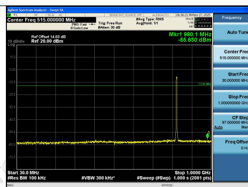
Band26(824-849)-5MHz-QPSK-26815-25RB#0-30 ~1000-PASS
