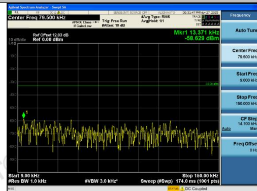
Band26(824-849)-5MHz-QPSK-26815-1RB#0-0.0 09~0.15-PASS
