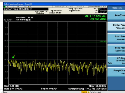
Band26(824-849)-5MHz-QPSK-26815-1RB#24-0. 009~0.15-PASS
