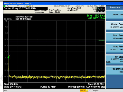
Band26(824-849)-5MHz-16QAM-26815-1RB#24-0 .15~30-PASS
