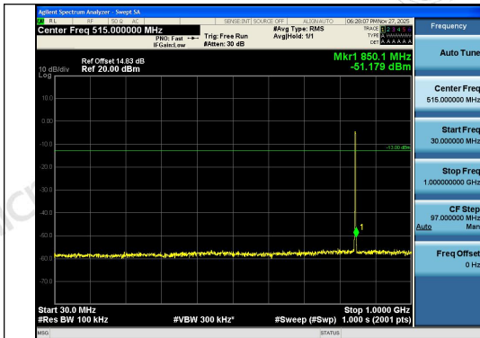
Band26(824-849)-3MHz-16QAM-27025-15RB#0-3 0~1000-PASS
