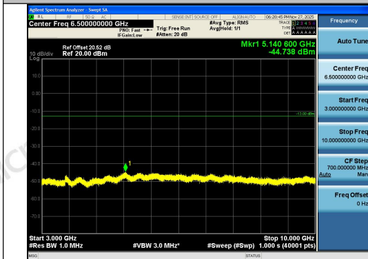
Band26(824-849)-3MHz-16QAM-27025-15RB#0-3 000~10000-PASS
