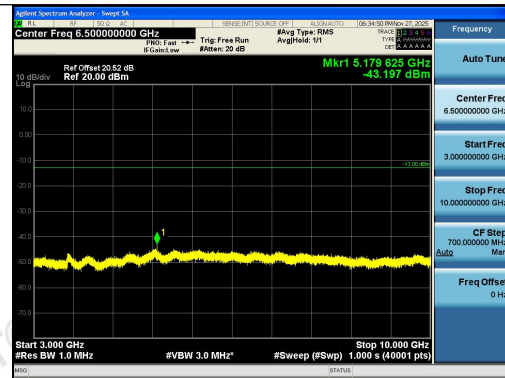
Band26(824-849)-5MHz-QPSK-26815-1RB#24-30 00~10000-PASS
