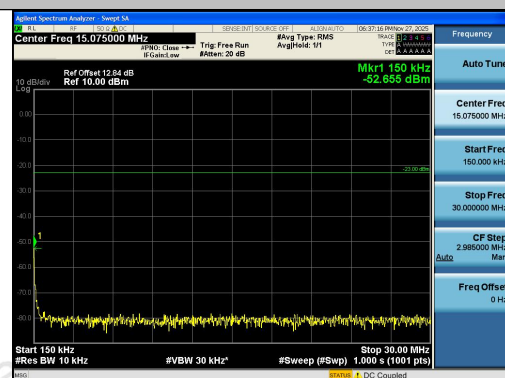
Band26(824-849)-5MHz-16QAM-26815-25RB#0-0 .15~30-PASS
