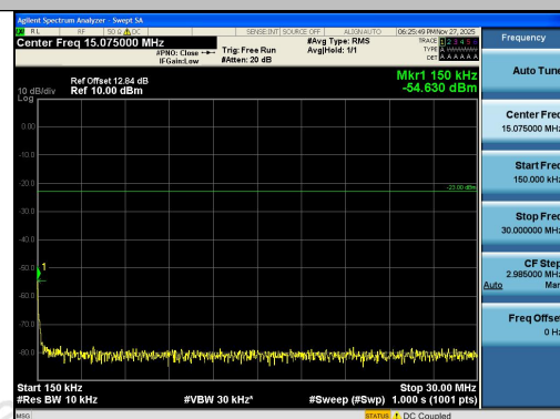
Band26(824-849)-3MHz-16QAM-27025-1RB#14-0 .15~30-PASS
