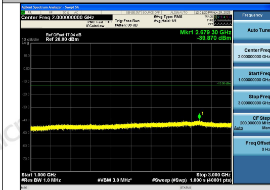
Band13-5MHz-QPSK-23255-1RB#0-1000~3000-P ASS
