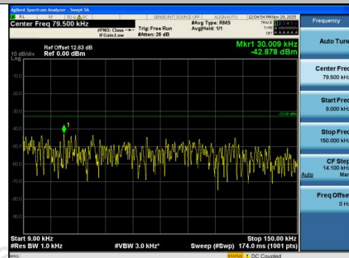
Band13-5MHz-QPSK-23255-25RB#0-0.009~0.15- PASS
