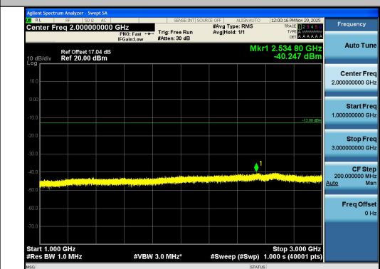
Band13-5MHz-16QAM-23230-25RB#0-1000~300
