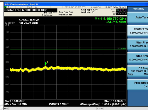
Band13-5MHz-QPSK-23255-1RB#0-3000~10000- PASS
