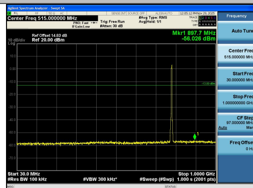
Band13-5MHz-QPSK-23255-25RB#0-30~1000-PA SS
