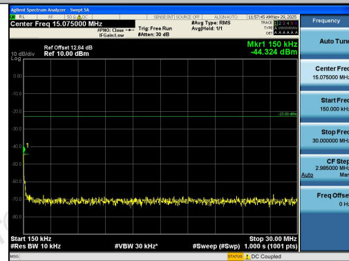
Band13-5MHz-16QAM-23230-1RB#24-0.15~30-P ASS
