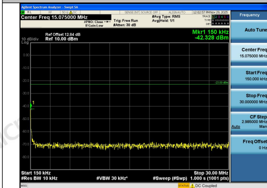
Band13-5MHz-QPSK-23255-1RB#24-0.15~30-PA
