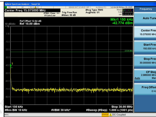
Band13-5MHz-16QAM-23255-1RB#24-0.15~30-P ASS
