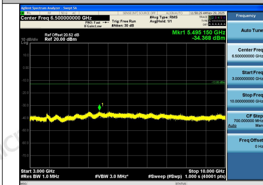
Band13-5MHz-16QAM-23230-1RB#24-3000~100 00-PASS
