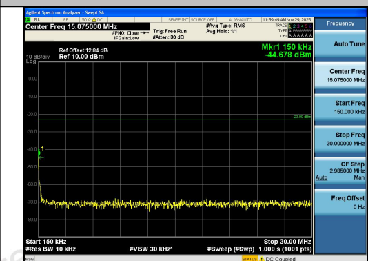
Band13-5MHz-16QAM-23230-25RB#0-0.15~30-P
