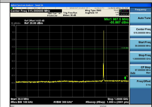
Band13-5MHz-QPSK-23230-1RB#24-30~1000-PA
