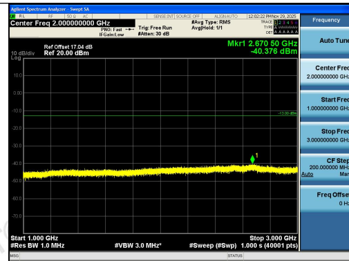
Band13-5MHz-16QAM-23255-1RB#0-1000~3000-
