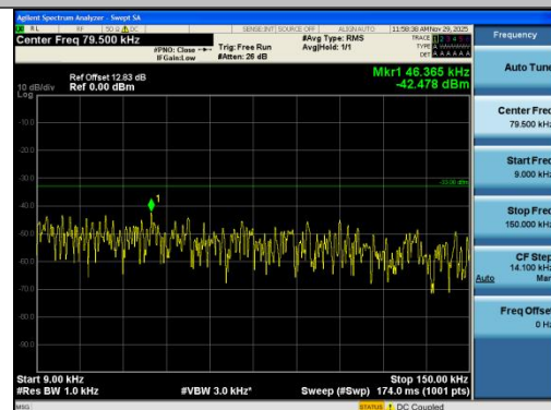
Band13-5MHz-QPSK-23230-25RB#0-0.009~0.15- PASS
