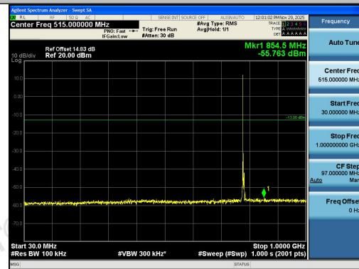
Band13-5MHz-QPSK-23255-1RB#0-30~1000-PA SS
