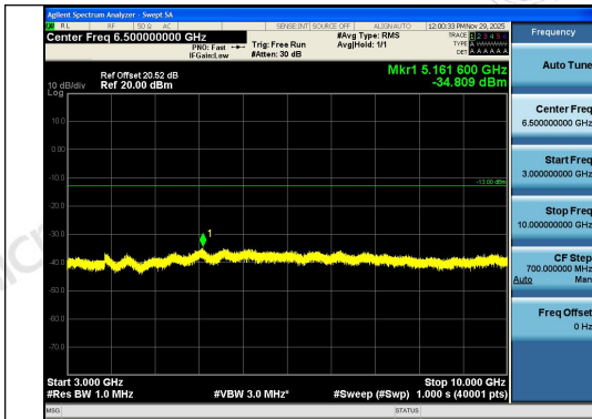
Band13-5MHz-16QAM-23230-25RB#0-3000~100 00-PASS
