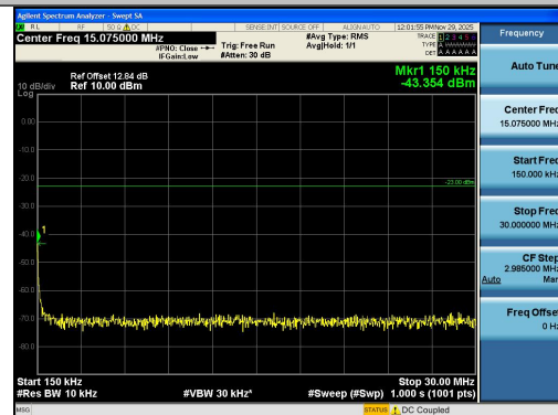
Band13-5MHz-16QAM-23255-1RB#0-0.15~30-PA SS
