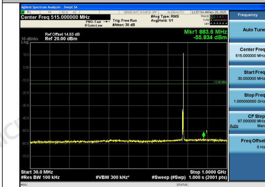
Band13-5MHz-16QAM-23230-1RB#24-30~1000-P ASS
