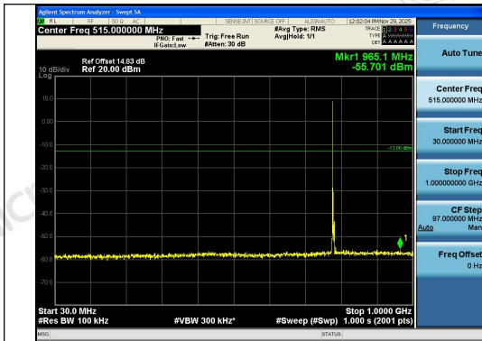
Band13-5MHz-16QAM-23255-1RB#0-30~1000-PA
