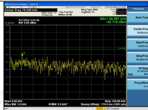
Band13-5MHz-QPSK-23255-1RB#24-0.009~0.15-
