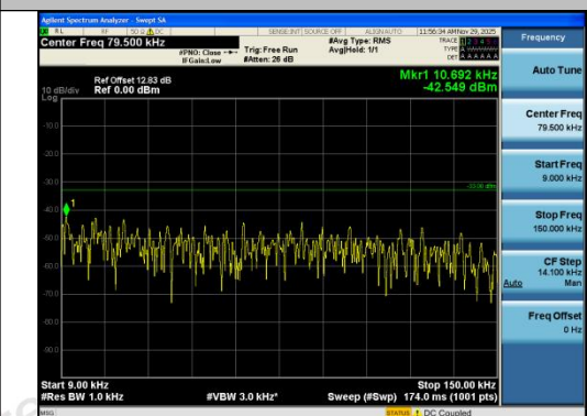
Band13-5MHz-QPSK-23230-1RB#24-0.009~0.15-
