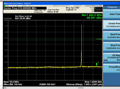
Band13-5MHz-QPSK-23255-1RB#24-30~1000-PA
