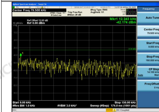
Band13-5MHz-16QAM-23230-1RB#24-0.009~0.1 5-PASS
