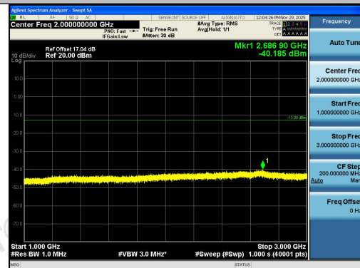
Band13-5MHz-16QAM-23255-1RB#24-1000~300 0-PASS
