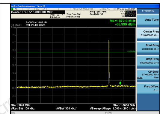
Band13-5MHz-QPSK-23230-25RB#0-30~1000-PA
