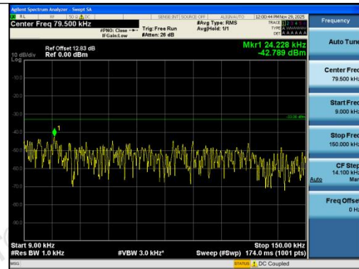
Band13-5MHz-QPSK-23255-1RB#0-0.009~0.15-P ASS
