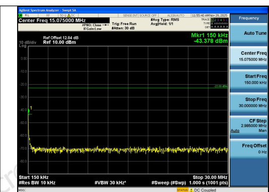
Band13-5MHz-16QAM-23230-1RB#0-0.15~30-PA
