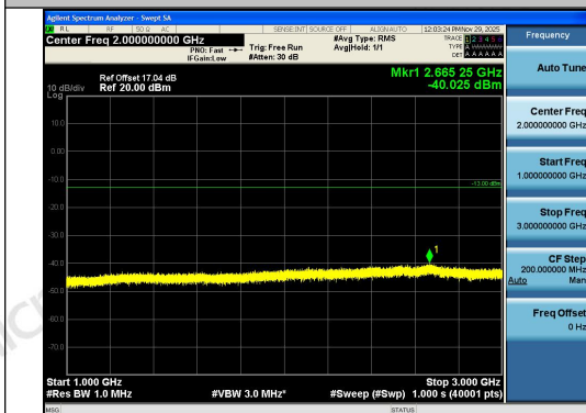
Band13-5MHz-QPSK-23255-1RB#24-1000~3000-
