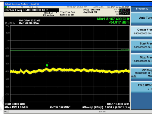
Band13-5MHz-QPSK-23230-1RB#24-3000~1000 0-PASS
