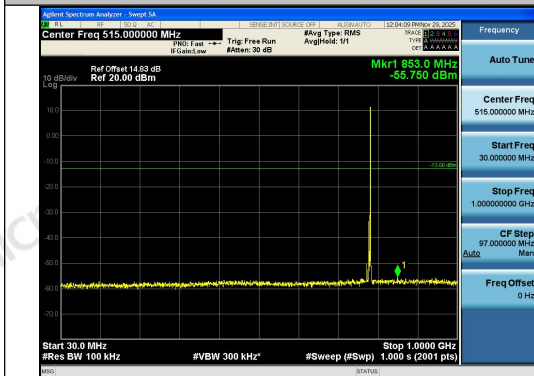
Band13-5MHz-16QAM-23255-1RB#24-30~1000-P ASS
