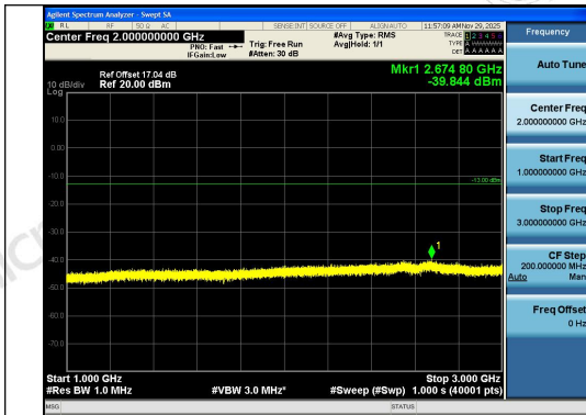
Band13-5MHz-QPSK-23230-1RB#24-1000~3000- PASS
