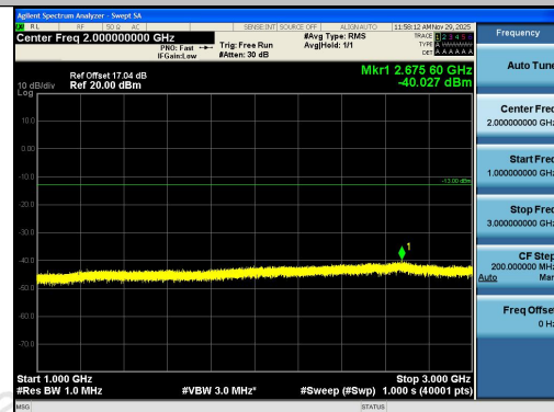
Band13-5MHz-16QAM-23230-1RB#24-1000~300 0-PASS
