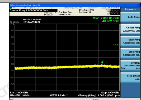
Band13-5MHz-16QAM-23230-1RB#0-1000~3000-
