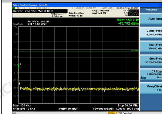
Band13-5MHz-QPSK-23255-25RB#0-0.15~30-PA SS
