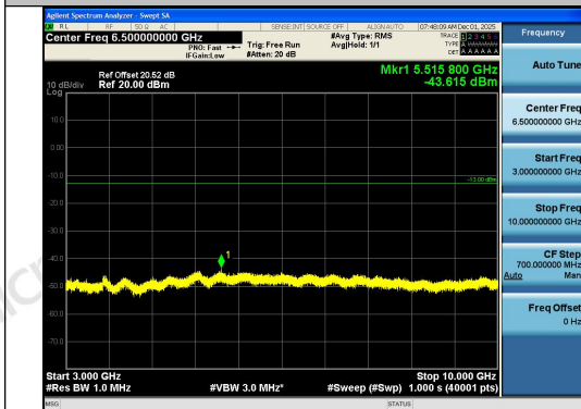
Band26(824-849)-10MHz-QPSK-26840-1RB#0-30 00~10000-PASS
