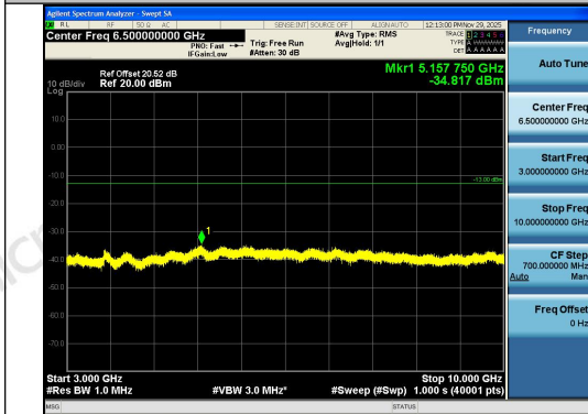
Band13-10MHz-16QAM-23230-1RB#49-3000~10000- 000-PASS
