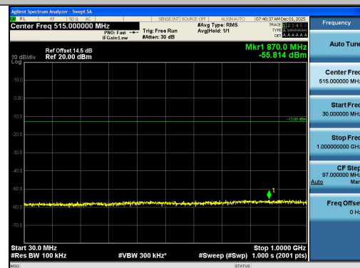
Band26(824-849)-10MHz-16QAM-26840-1RB#0-3 0~1000-PASS
