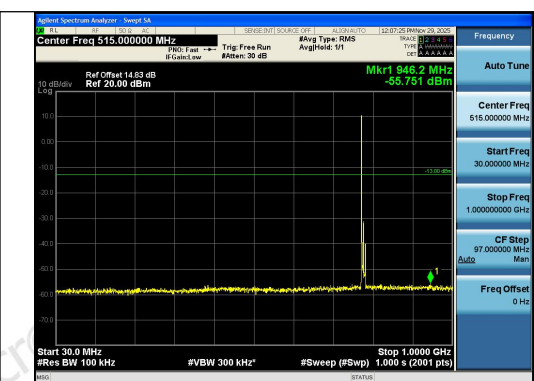
Band13-10MHz-QPSK-23230-1RB#0-30~1000-PA
