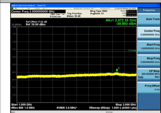
Band13-10MHz-16QAM-23230-1RB#0-1000~300
