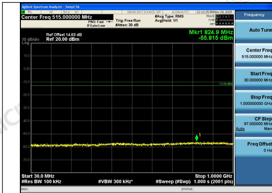
Band13-10MHz-16QAM-23230-1RB#49-30~1000- PASS
