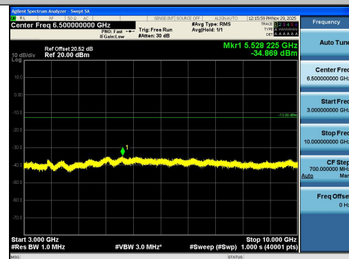
Band13-10MHz-QPSK-23230-50RB#0-3000~10000- 00-PASS
