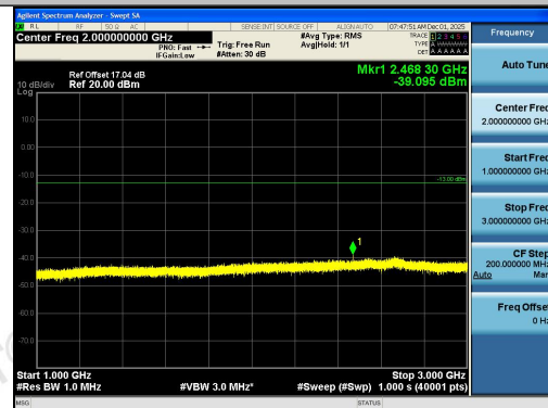
Band26(824-849)-10MHz-QPSK-26840-1RB#0-10 00~3000-PASS
