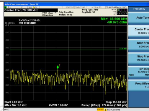
Band26(824-849)-10MHz-16QAM-26840-1RB#0-0. .009~0.15-PASS
