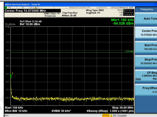
Band26(824-849)-10MHz-QPSK-26840-1RB#49-0 .15~30-PASS
