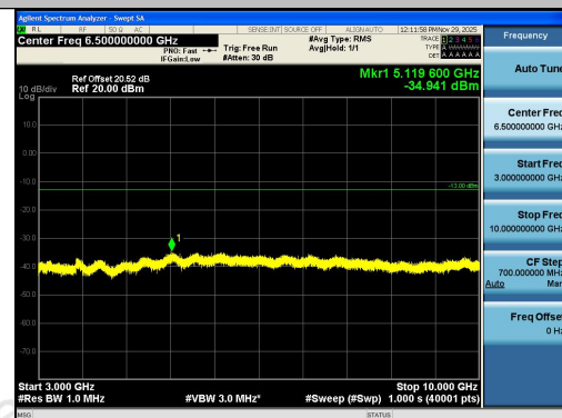
Band13-10MHz-QPSK-23230-1RB#49-3000~100 00-PASS
