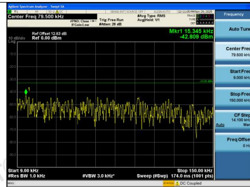
Band13-10MHz-QPSK-23230-1RB#49-0.009~0.1 5-PASS
