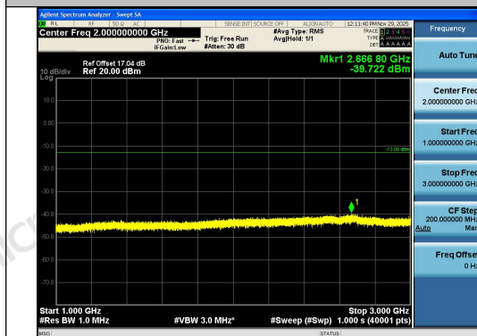
Band13-10MHz-QPSK-23230-1RB#49-1000~300 0-PASS
