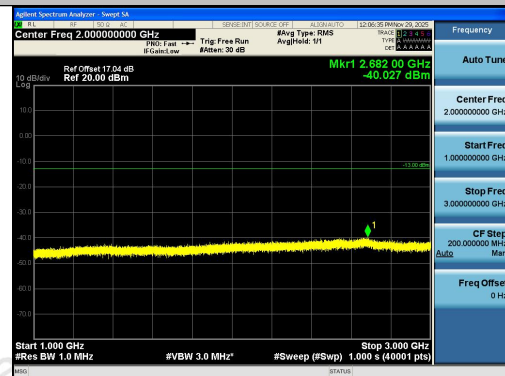
Band13-5MHz-16QAM-23255-25RB#0-1000~300- 0-PASS
