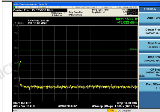
Band13-10MHz-QPSK-23230-1RB#49-0.15~30-P ASS
