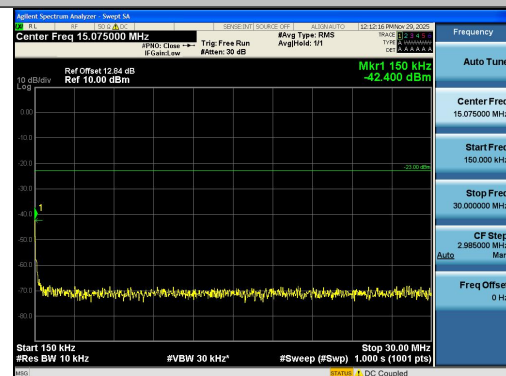
Band13-10MHz-16QAM-23230-1RB#49-0.15~30-PASS
