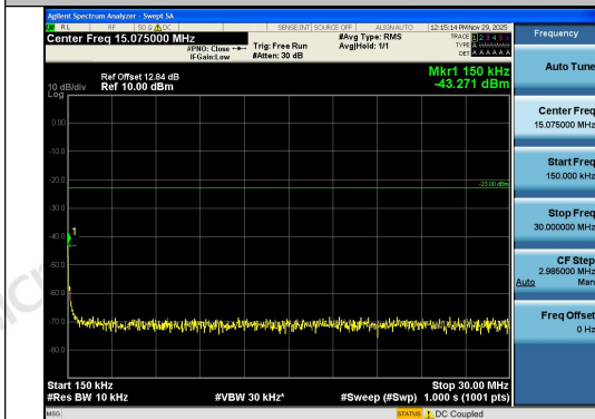
Band13-10MHz-QPSK-23230-50RB#0-0.15~30-PASS
