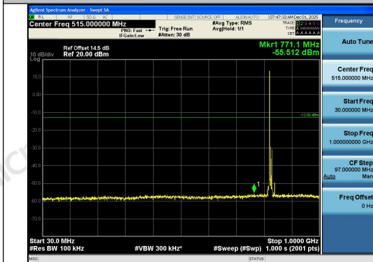
Band26(824-849)-10MHz-QPSK-26840-1RB#0-30 ~1000-PASS
