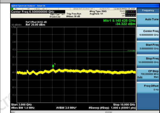
Band13-10MHz-QPSK-23230-1RB#0-3000~1000
