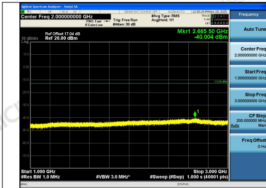
Band13-5MHz-QPSK-23255-25RB#0-1000~3000- PASS
