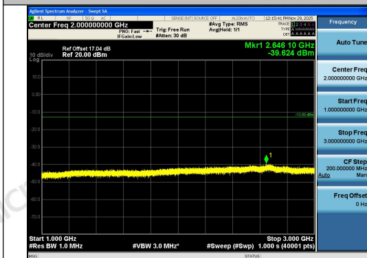
Band13-10MHz-QPSK-23230-50RB#0-1000~3000- 0-PASS
