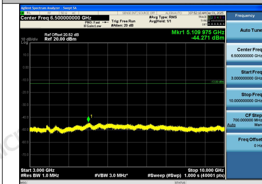
Band26(824-849)-10MHz-QPSK-26840-1RB#49-3 000~10000-PASS
