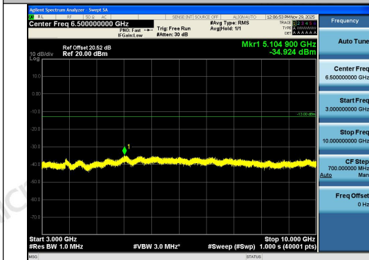
Band13-5MHz-16QAM-23255-25RB#0-3000~100- 00-PASS
