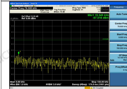
Band26(824-849)-10MHz-QPSK-26840-1RB#49-0 .009~0.15-PASS
