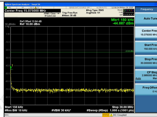
Band13-5MHz-16QAM-23255-25RB#0-0.15~30-P- ASS
