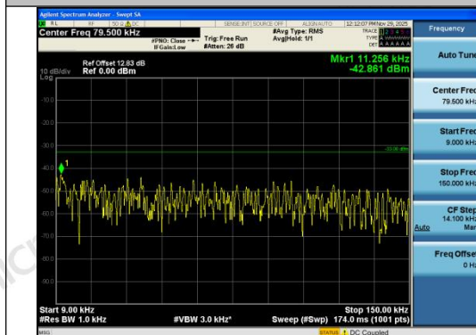
Band13-10MHz-16QAM-23230-1RB#49-0.009~0.1 15-PASS
