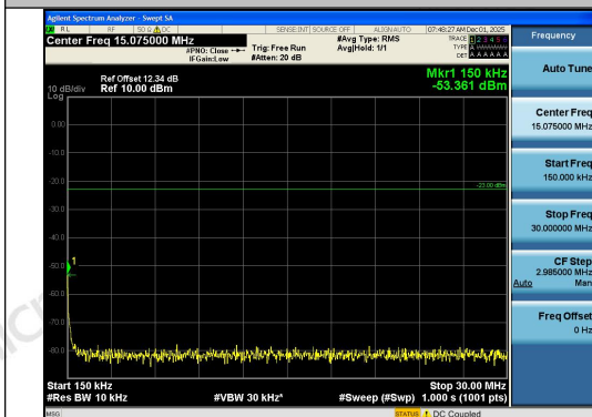
Band26(824-849)-10MHz-16QAM-26840-1RB#0-0. .15~30-PASS
