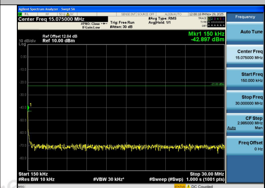
Band13-10MHz-16QAM-23230-1RB#0-0.15~30-P
