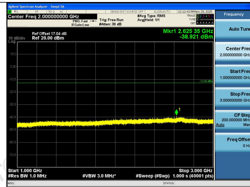
Band13-10MHz-16QAM-23230-1RB#49-1000~3000- 00-PASS
