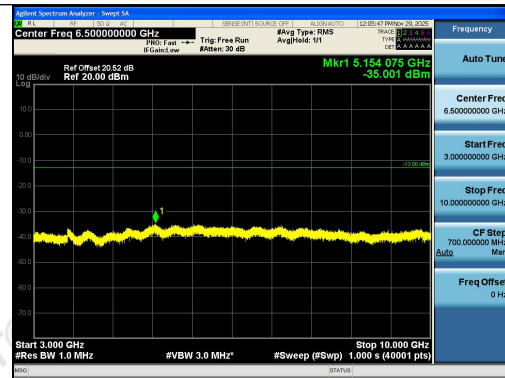
Band13-5MHz-QPSK-23255-25RB#0-3000~1000- 0-PASS
