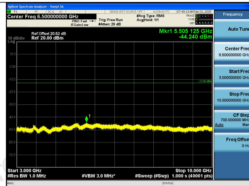
Band26(824-849)-10MHz-16QAM-26840-1RB#0-3 000~10000-PASS
