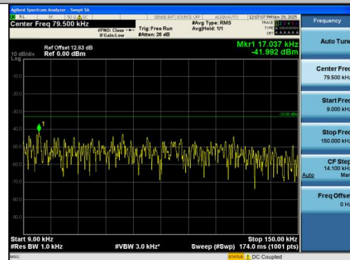
Band13-10MHz-QPSK-23230-1RB#0-0.009~0.15- PASS
