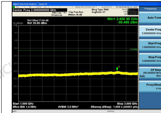
Band26(824-849)-10MHz-16QAM-26840-1RB#0-1 000~3000-PASS
