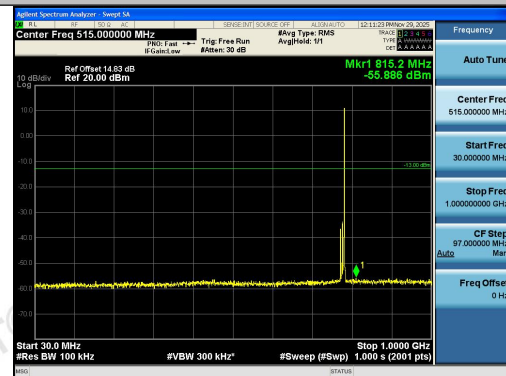
Band13-10MHz-QPSK-23230-1RB#49-30~1000-P ASS
