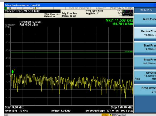
Band26(824-849)-10MHz-16QAM-26840-1RB#49-9 0.009~0.15-PASS
