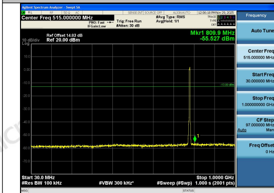
Band13-5MHz-16QAM-23255-25RB#0-30~1000-P- ASS
