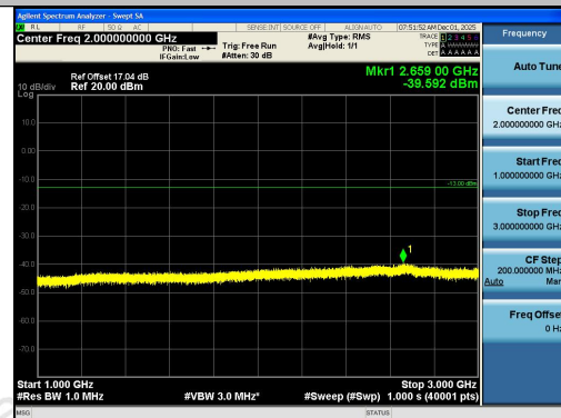
Band26(824-849)-10MHz-QPSK-26840-1RB#49-1 000~3000-PASS
