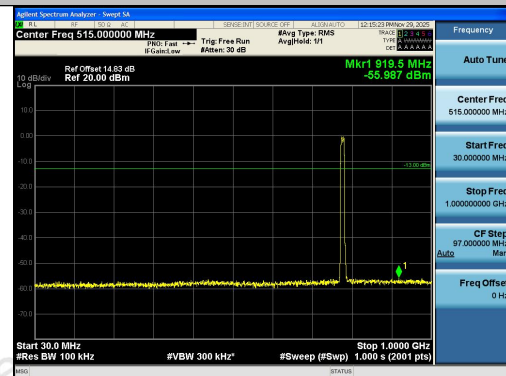
Band13-10MHz-QPSK-23230-50RB#0-30~1000-PASS
