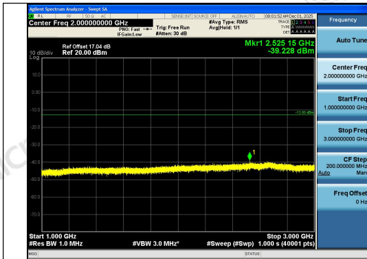
Band26(824-849)-10MHz-16QAM-26990-1RB#0-1 000~3000-PASS
