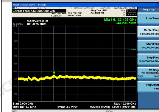
Band26(824-849)-10MHz-QPSK-26990-1RB#49-3 000~10000-PASS
