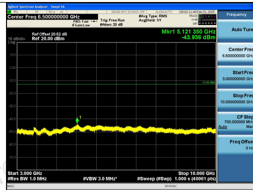
Band26(824-849)-10MHz-16QAM-26990-1RB#0-3 000~10000-PASS
