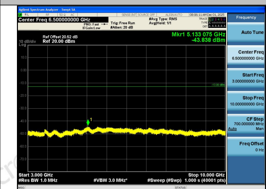
Band26(824-849)-10MHz-16QAM-26990-1RB#49- 3000~10000-PASS
