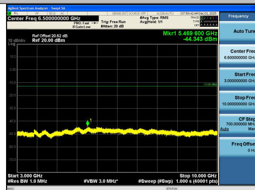
Band26(824-849)-10MHz-16QAM-26915-1RB#49- 3000~10000-PASS
