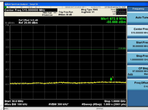
Band26(824-849)-10MHz-16QAM-26915-1RB#49- 30~1000-PASS
