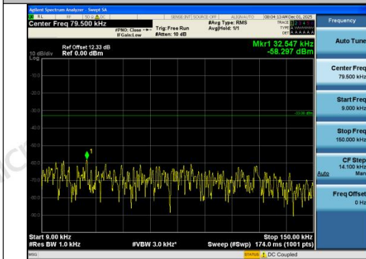
Band26(824-849)-10MHz-QPSK-26990-1RB#49-0 .009~0.15-PASS
