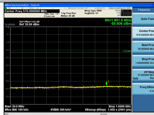
Band26(824-849)-10MHz-16QAM-26990-1RB#0-3 0~1000-PASS
