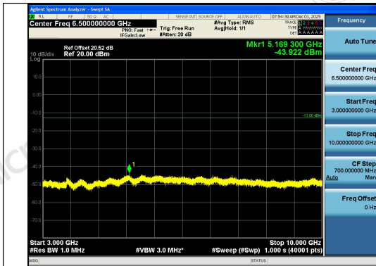
Band26(824-849)-10MHz-QPSK-26915-1RB#0-30 00~10000-PASS
