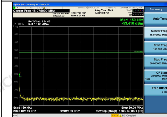
Band26(824-849)-10MHz-16QAM-26915-1RB#49- 0.15~30-PASS
