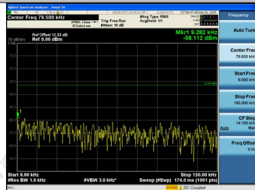
Band26(824-849)-10MHz-16QAM-26915-1RB#49- 0.009~0.15-PASS
