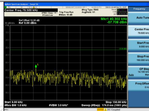
Band26(824-849)-10MHz-16QAM-26990-1RB#0-0. .009~0.15-PASS
