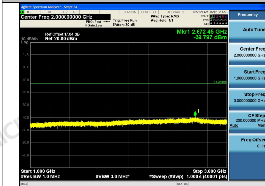
Band26(824-849)-10MHz-16QAM-26915-1RB#0-1 000~3000-PASS
