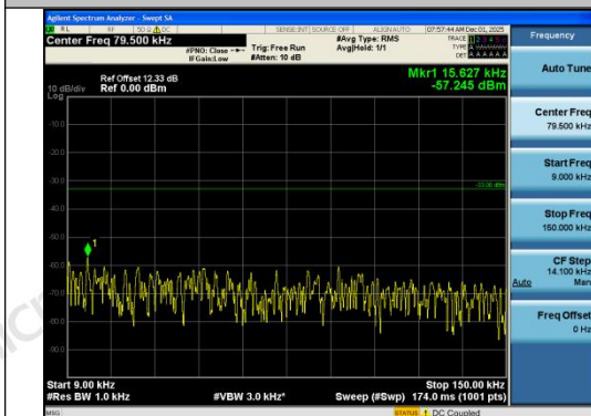
Band26(824-849)-10MHz-QPSK-26915-1RB#49-0 .009~0.15-PASS
