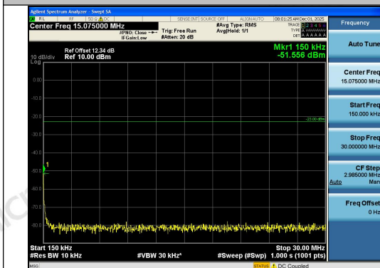
Band26(824-849)-10MHz-16QAM-26990-1RB#0-0. .15~30-PASS
