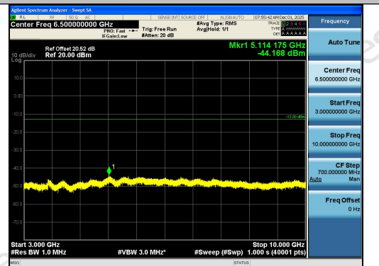
Band26(824-849)-10MHz-16QAM-26915-1RB#0-3 000~10000-PASS
