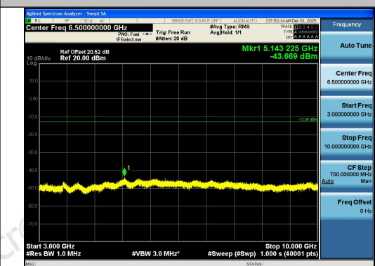
Band26(824-849)-10MHz-16QAM-26840-1RB#49- 3000~10000-PASS
