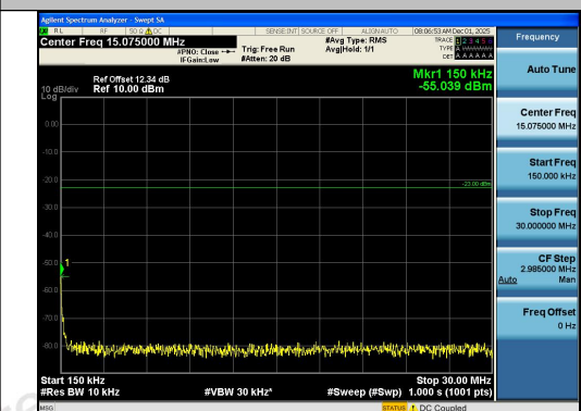
Band26(824-849)-10MHz-QPSK-26840-50RB#0-0 .15~30-PASS
