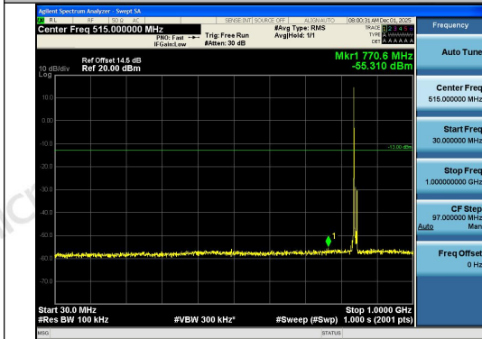
Band26(824-849)-10MHz-QPSK-26990-1RB#0-30 ~1000-PASS
