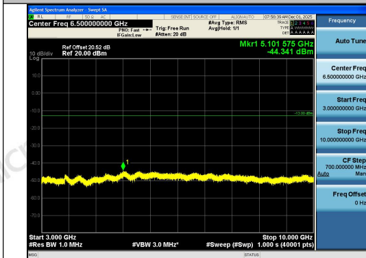
Band26(824-849)-10MHz-QPSK-26915-1RB#49-3 000~10000-PASS
