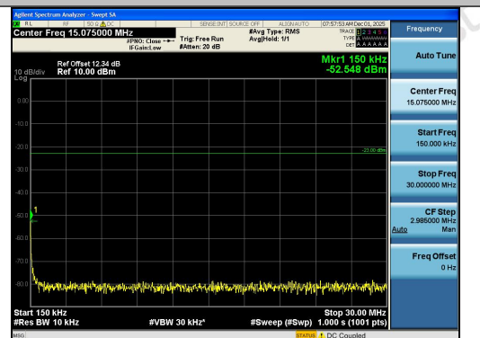
Band26(824-849)-10MHz-QPSK-26915-1RB#49-0 .15~30-PASS
