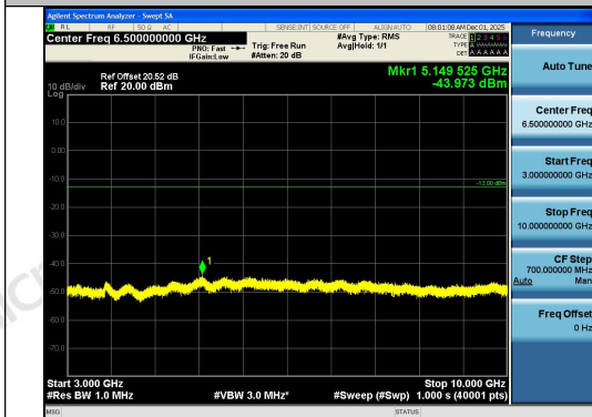
Band26(824-849)-10MHz-QPSK-26990-1RB#0-30 00~10000-PASS
