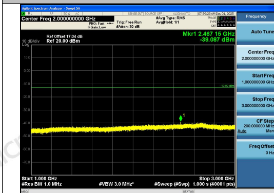
Band26(824-849)-10MHz-16QAM-26915-1RB#49- 1000~3000-PASS
