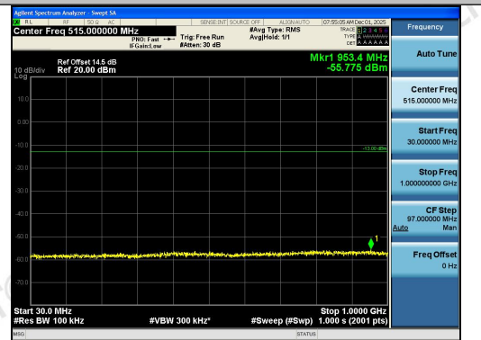
Band26(824-849)-10MHz-16QAM-26915-1RB#0-3 0~1000-PASS
