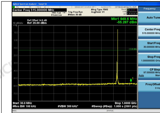
Band26(824-849)-10MHz-QPSK-26915-1RB#49-3 0~1000-PASS
