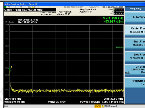
Band26(824-849)-10MHz-QPSK-26990-1RB#49-0 .15~30-PASS
