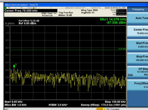
Band26(824-849)-10MHz-16QAM-26990-1RB#49-9 0.009~0.15-PASS
