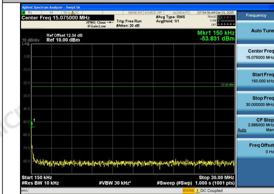
Band26(824-849)-10MHz-16QAM-26915-1RB#0-0 .15~30-PASS
