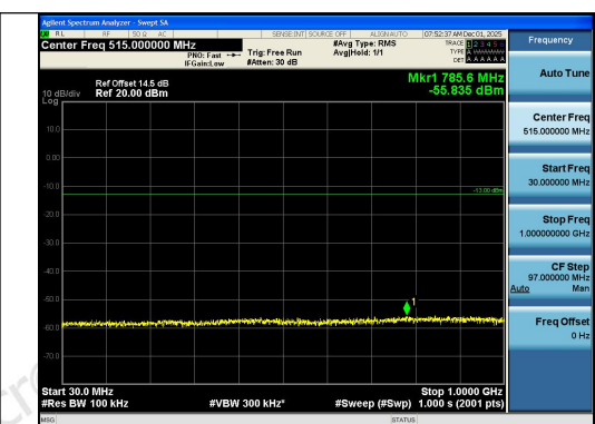
Band26(824-849)-10MHz-16QAM-26840-1RB#49- 30~1000-PASS
