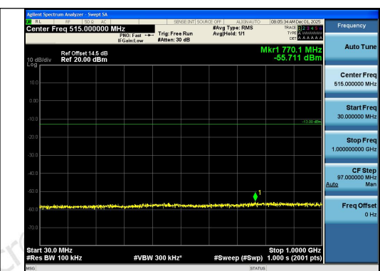
Band26(824-849)-10MHz-16QAM-26990-1RB#49- 30~1000-PASS
