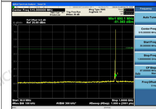
Band26(824-849)-10MHz-QPSK-26990-1RB#49-3 0~1000-PASS
