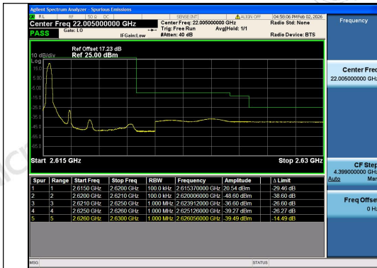
Band38-5MHz-QPSK-38225-1RB#0-PASS
