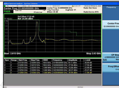
Band38-5MHz-16QAM-38225-1RB#24-PASS
