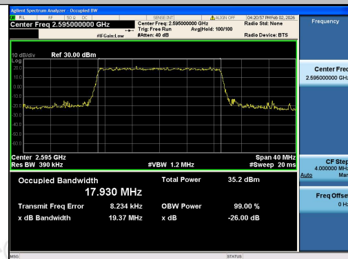
Band38-20MHz-QPSK-38000-100RB#0-PASS
