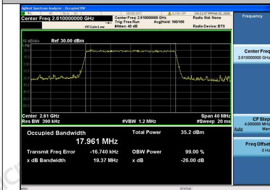
Band38-20MHz-QPSK-38150-100RB#0-PASS
