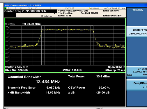
Band38-15MHz-QPSK-38000-75RB#0-PASS
