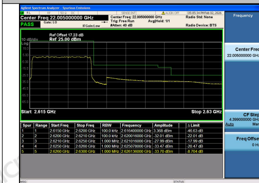
Band38-5MHz-QPSK-38225-25RB#0-PASS
