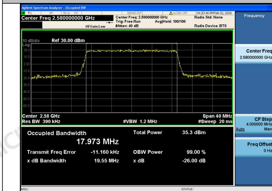
Band38-20MHz-QPSK-37850-100RB#0-PASS
