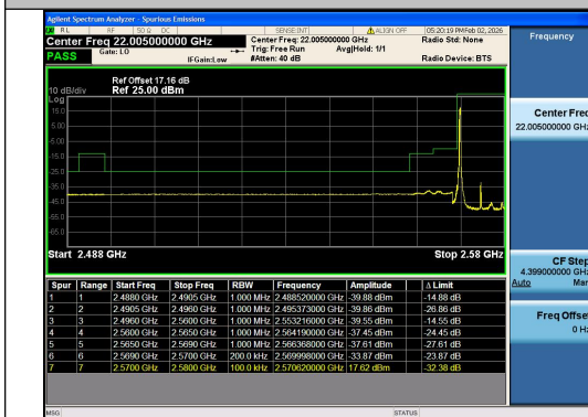
Band38-10MHz-QPSK-37800-1RB#0-PASS
