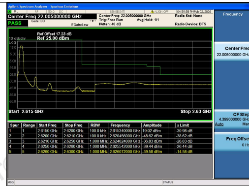
Band38-5MHz-16QAM-38225-1RB#0-PASS
