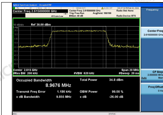
Band38-10MHz-QPSK-38200-50RB#0-PASS
