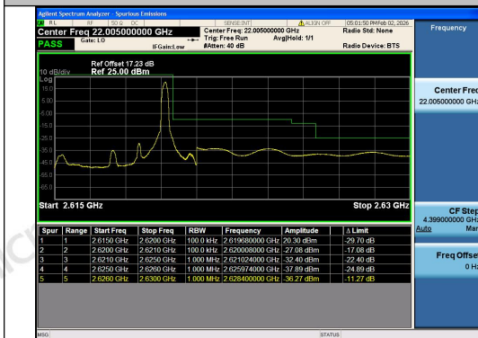
Band38-5MHz-QPSK-38225-1RB#24-PASS
