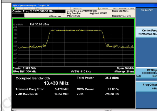
Band38-15MHz-QPSK-37825-75RB#0-PASS
