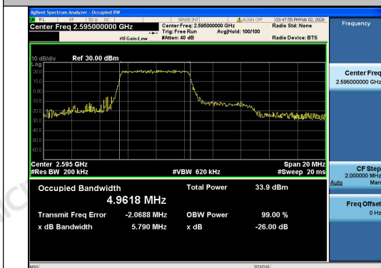
Band38-10MHz-16QAM-38000-27RB#0-PASS
