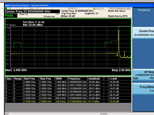
Band38-10MHz-16QAM-37800-1RB#0-PASS
