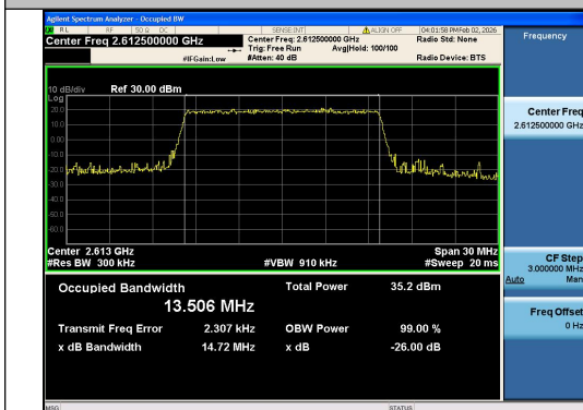
Band38-15MHz-QPSK-38175-75RB#0-PASS
