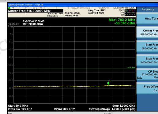
Band38-5MHz-QPSK-37775-25RB#0-30~1000-P
