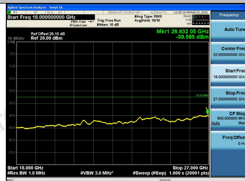
Band38-5MHz-16QAM-37775-25RB#0-18000~270
