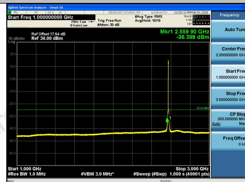
Band38-5MHz-QPSK-37775-25RB#0-1000~3000-
