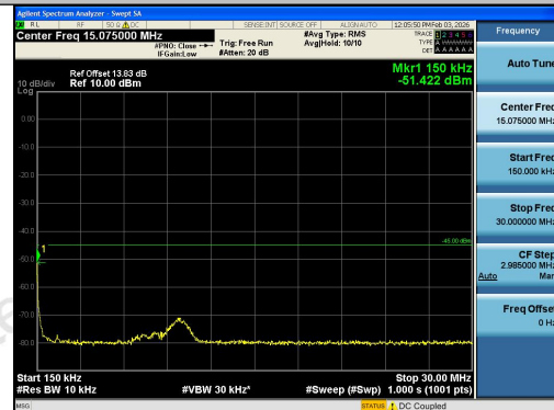
Band38-5MHz-QPSK-38000-1RB#0-0.15~30-PAS
