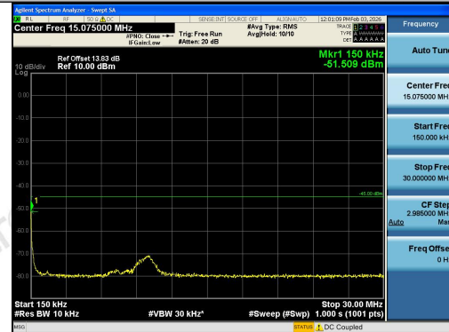
Band38-5MHz-QPSK-37775-25RB#0-0.15~30-PA
