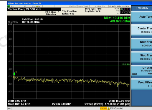
Band38-5MHz-QPSK-37775-25RB#0-0.009~0.15
