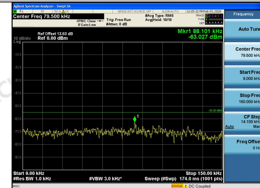
Band38-5MHz-QPSK-38000-1RB#0-0.009~0.15-
