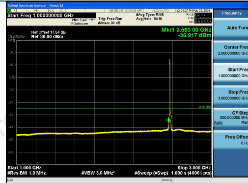
Band38-5MHz-16QAM-37775-25RB#0-1000~3000
