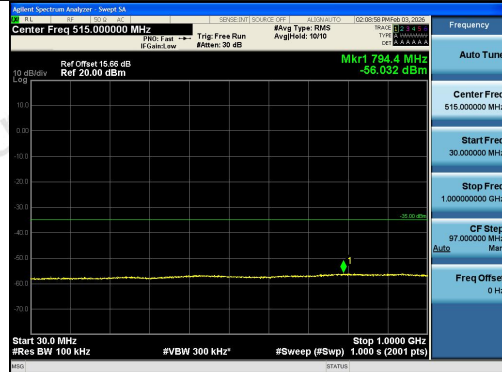
Band38-20MHz-QPSK-38000-1RB#99-30~1000-
