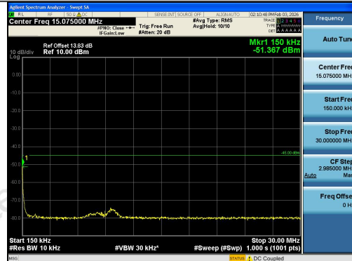
Band38-20MHz-16QAM-38000-1RB#99-0.15~30-P
