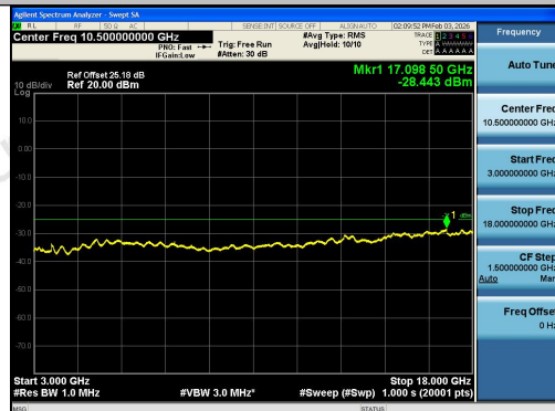
Band38-20MHz-QPSK-38000-1RB#99-3000~180
