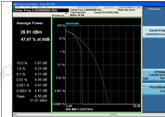
Band41-5MHz-16QAM-40620-1RB#0-PASS
