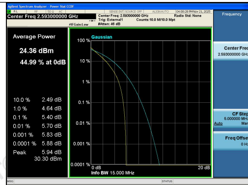
Band41-15MHz-QPSK-40620-75RB#0-PASS
