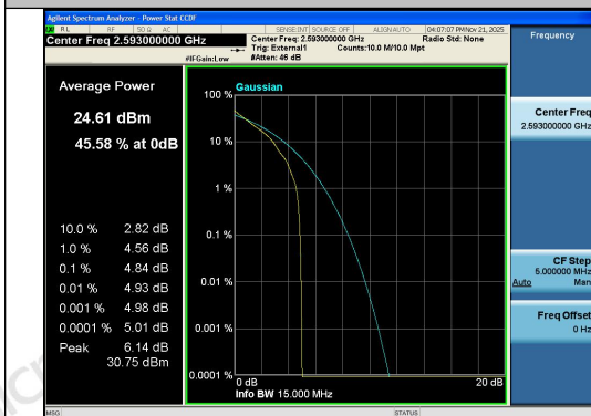
Band41-15MHz-QPSK-40620-1RB#0-PASS
