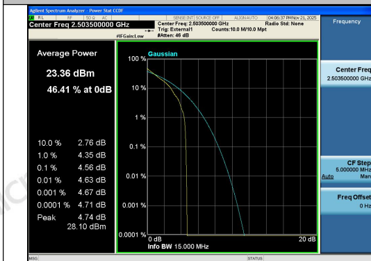
Band41-15MHz-QPSK-39725-1RB#0-PASS
