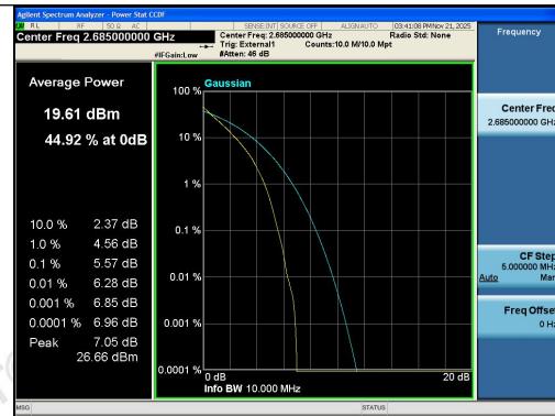
Band41-10MHz-QPSK-41540-50RB#0-PASS
