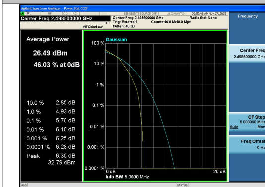
Band41-5MHz-16QAM-39675-25RB#0-PASS
