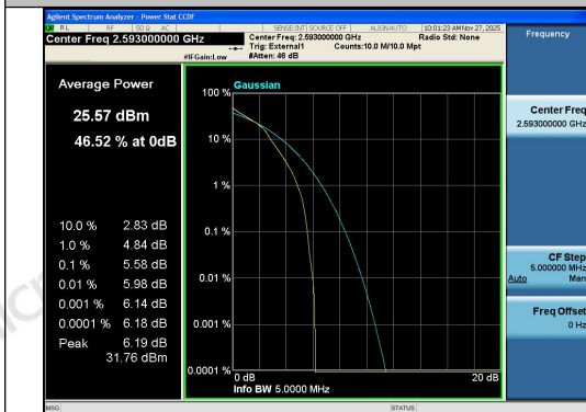
Band41-5MHz-16QAM-40620-25RB#0-PASS
