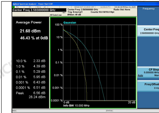
Band41-10MHz-QPSK-40620-50RB#0-PASS
