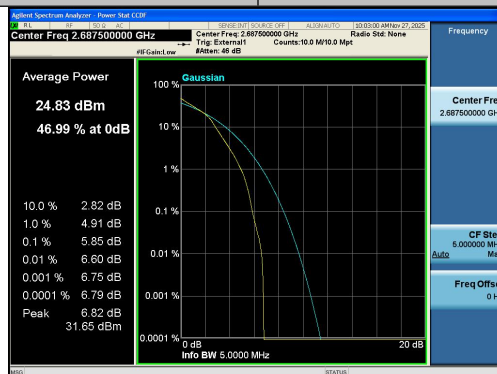
Band41-5MHz-16QAM-41565-25RB#0-PASS
