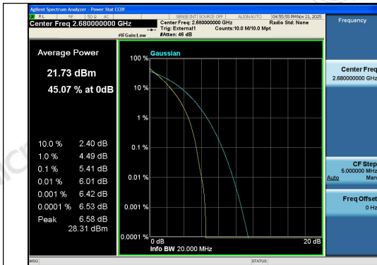
Band41-20MHz-QPSK-41490-100RB#0-PASS
