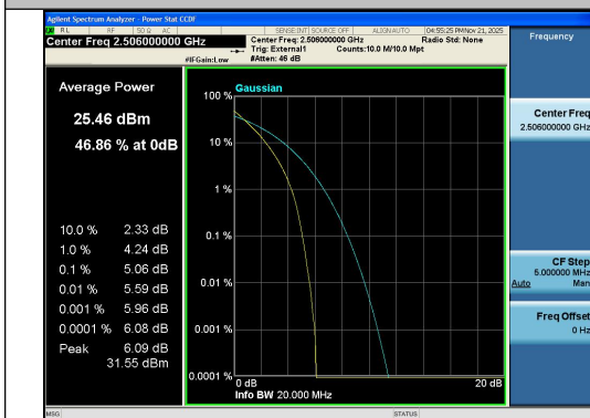
Band41-20MHz-QPSK-39750-100RB#0-PASS
