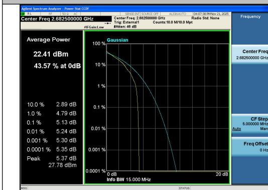
Band41-15MHz-QPSK-41515-1RB#0-PASS
