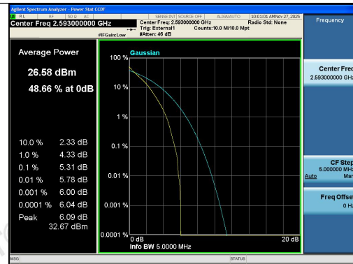
Band41-5MHz-QPSK-40620-25RB#0-PASS
