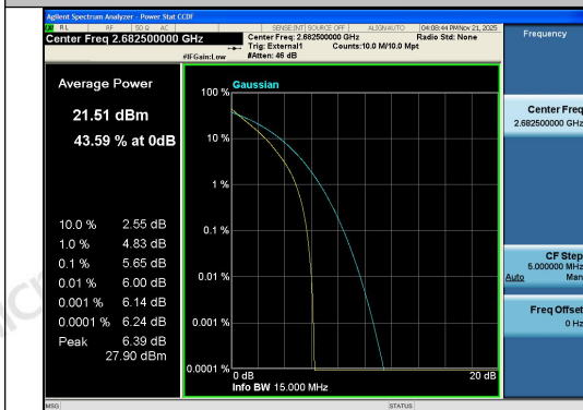
Band41-15MHz-QPSK-41515-75RB#0-PASS
