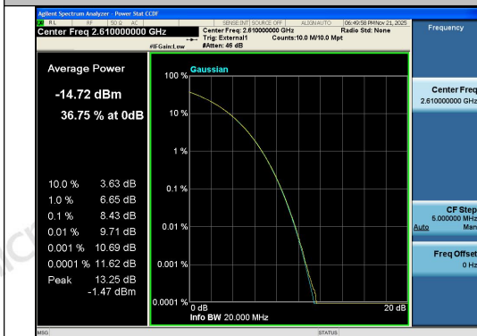
Band38-20MHz-16QAM-38150-100RB#0-PASS
