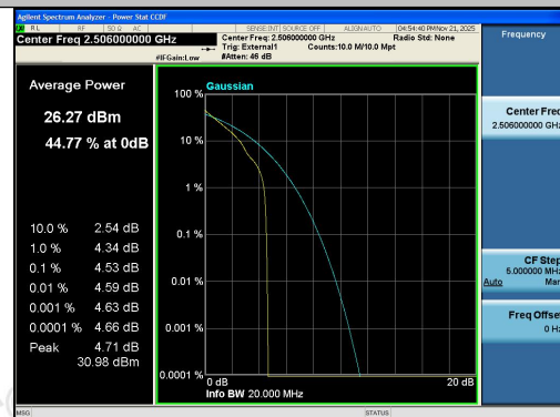
Band41-20MHz-QPSK-39750-1RB#0-PASS
