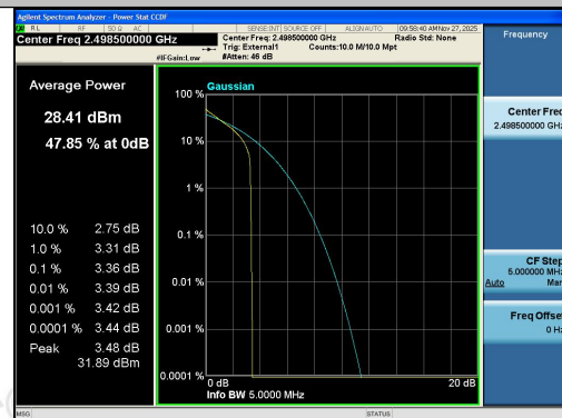
Band41-5MHz-QPSK-39675-1RB#0-PASS
