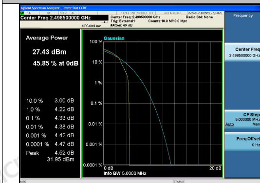
Band41-5MHz-16QAM-39675-1RB#0-PASS
