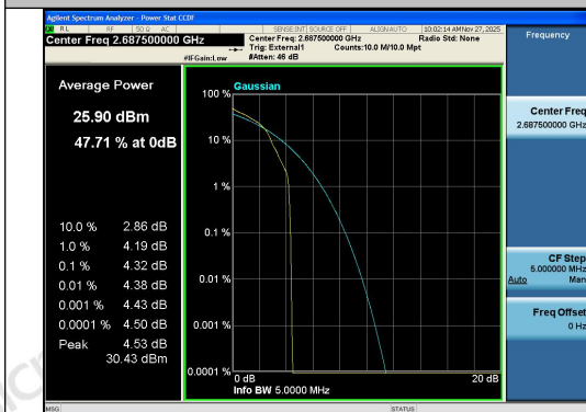
Band41-5MHz-16QAM-41565-1RB#0-PASS
