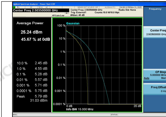
Band41-15MHz-QPSK-39725-75RB#0-PASS
