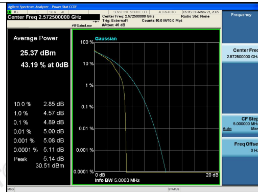
Band38-5MHz-QPSK-37775-1RB#0-PASS
