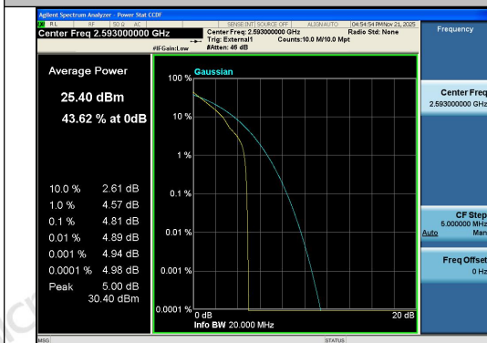
Band41-20MHz-QPSK-40620-1RB#0-PASS
