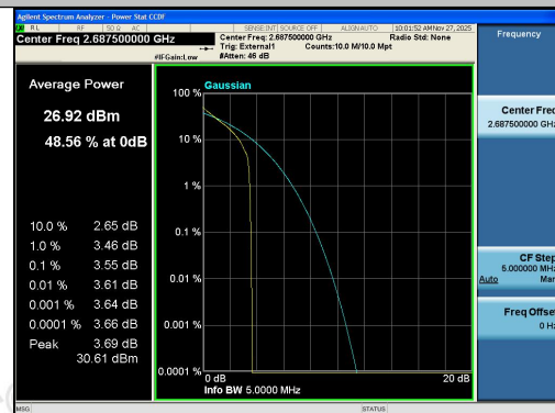
Band41-5MHz-QPSK-41565-1RB#0-PASS
