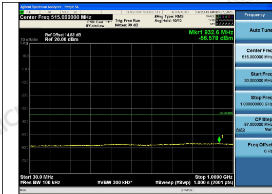
Band41-5MHz-QPSK-40620-1RB#0-30~1000-PA SS
