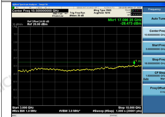
Band41-5MHz-16QAM-39675-1RB#0-3000~1800 0-PASS
