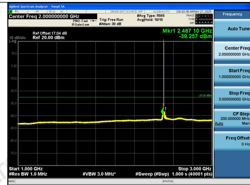
Band41-5MHz-QPSK-39675-1RB#24-1000~3000-P PASS
