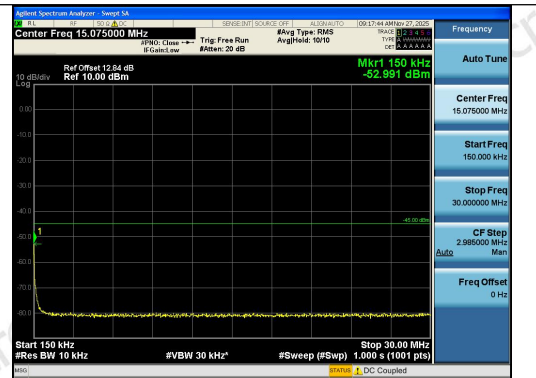
Band41-5MHz-16QAM-39675-1RB#0-0.15~30-PA SS
