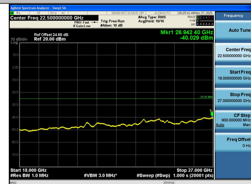
Band41-5MHz-QPSK-39675-25RB#0-18000~2700 0-PASS
