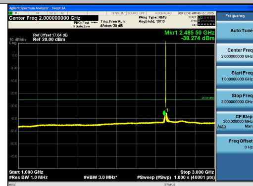
Band41-5MHz-16QAM-39675-1RB#24-1000~3000 -PASS
