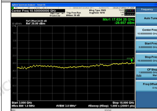
Band41-5MHz-QPSK-39675-25RB#0-3000~1800 0-PASS
