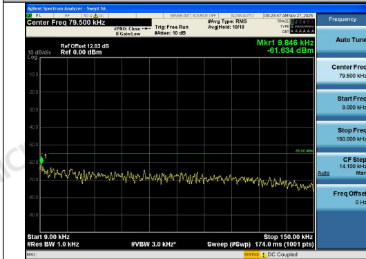
Band41-5MHz-QPSK-39675-25RB#0-0.009~0.15 -PASS
