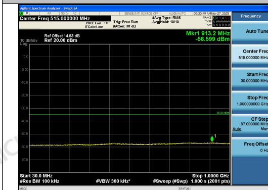
Band41-5MHz-16QAM-40620-1RB#0-0-30~1000-P ASS
