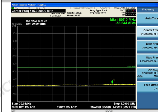
Band41-5MHz-16QAM-39675-1RB#24-30~1000-P PASS
