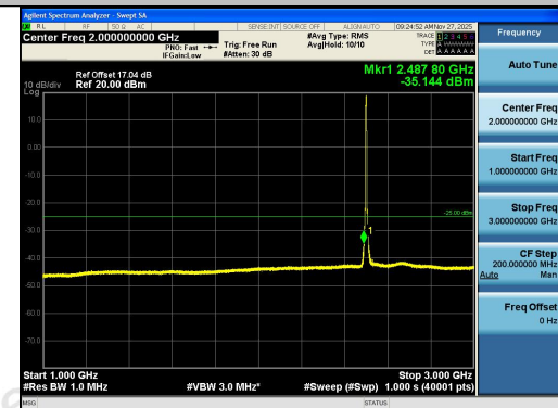
Band41-5MHz-QPSK-39675-25RB#0-1000~3000- PASS
