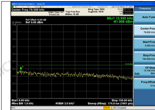
Band41-5MHz-16QAM-39675-1RB#0-0.009~0.15 -PASS
