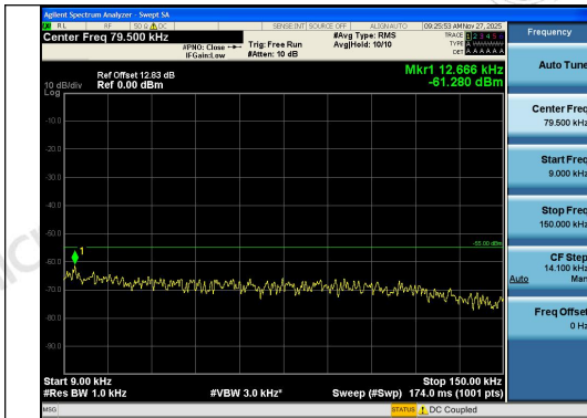
Band41-5MHz-16QAM-39675-25RB#0-0.009~0.1 5-PASS
