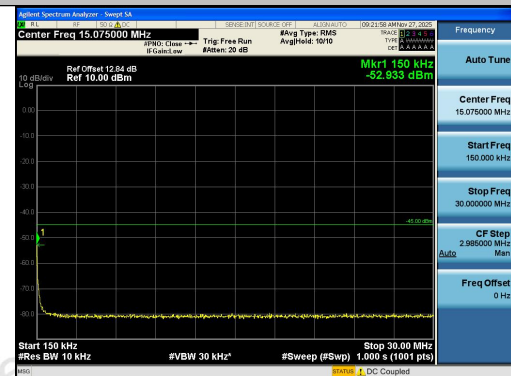
Band41-5MHz-16QAM-39675-1RB#24-0.15~30-P ASS
