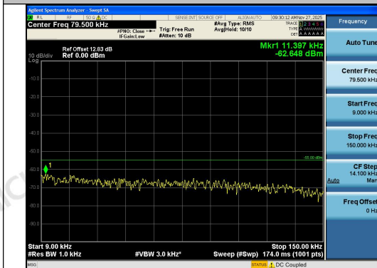
Band41-5MHz-16QAM-40620-1RB#0-0.009~0.15 -PASS
