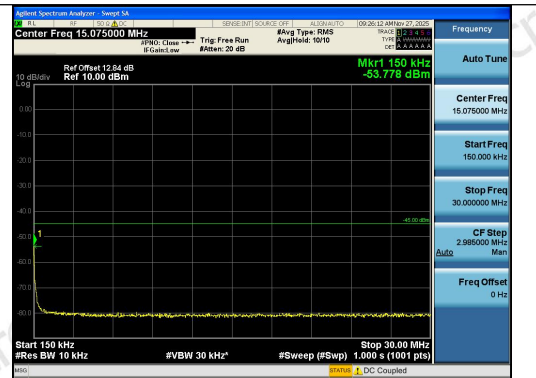
Band41-5MHz-16QAM-39675-25RB#0-0.15~30-P ASS
