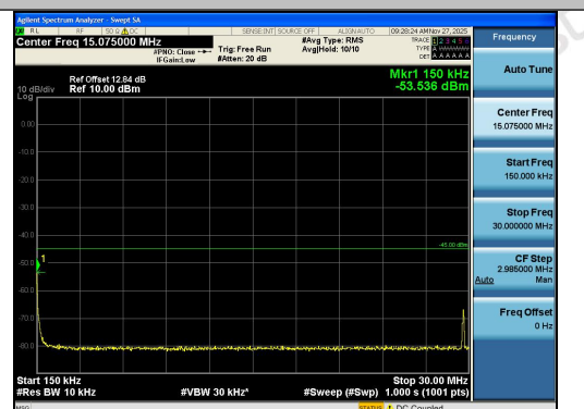
Band41-5MHz-QPSK-40620-1RB#0-0.15~30-PAS S
