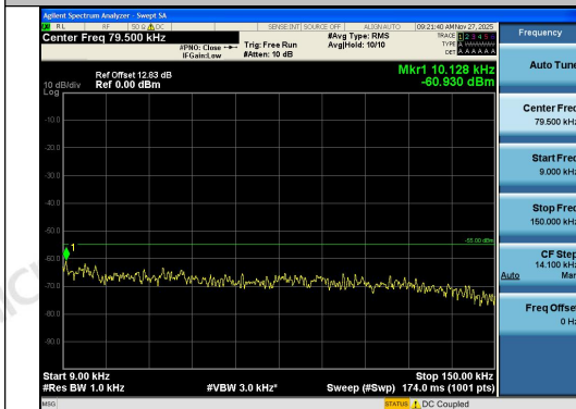
Band41-5MHz-16QAM-39675-1RB#24-0.009~0.1 5-PASS
