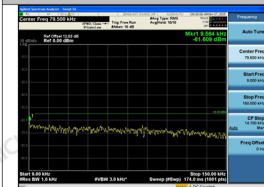
Band41-5MHz-QPSK-40620-1RB#0-0.009~0.15- PASS
