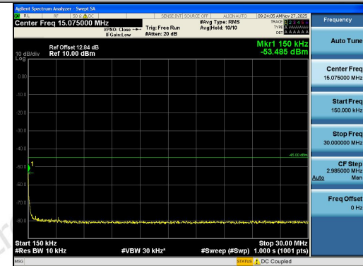
Band41-5MHz-QPSK-39675-25RB#0-0.15~30-PA SS
