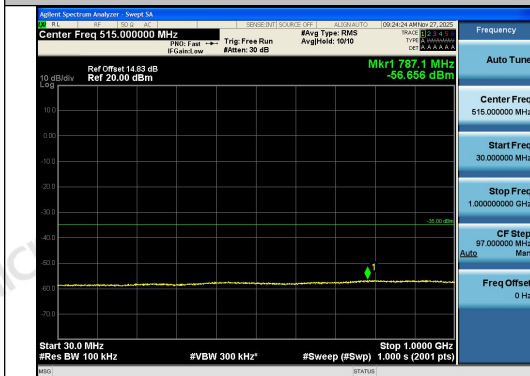
Band41-5MHz-QPSK-39675-25RB#0-30~1000-P ASS
