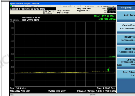
Band41-5MHz-16QAM-39675-25RB#0-30~1000- PASS
