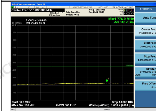
Band41-5MHz-16QAM-39675-1RB#0-30~1000-P ASS
