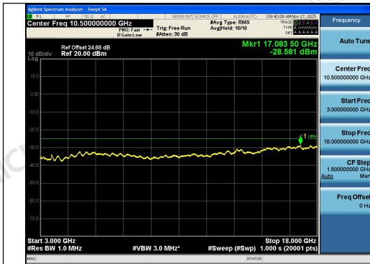
Band41-5MHz-16QAM-40620-25RB#0-3000~180 00-PASS
