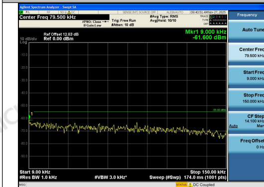
Band41-5MHz-QPSK-41565-1RB#0-0.009~0.15- PASS
