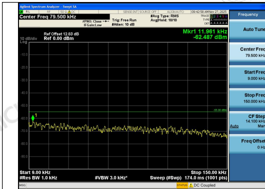
Band41-5MHz-16QAM-41565-1RB#0-0.009~0.15 -PASS
