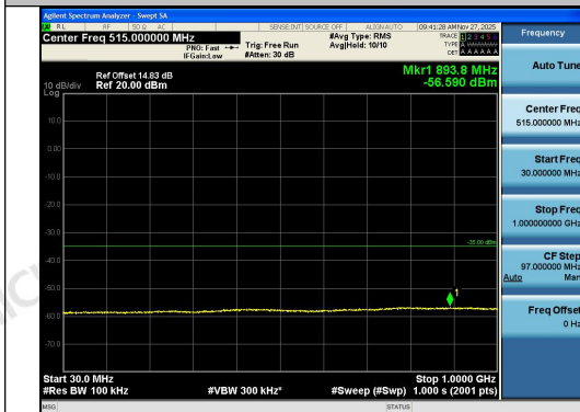
Band41-5MHz-QPSK-41565-1RB#0-30~1000-PA SS
