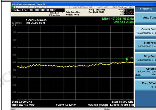
Band41-5MHz-16QAM-40620-1RB#24-3000~18000- 00-PASS
