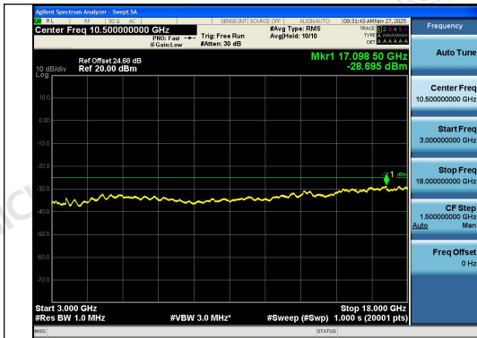
Band41-5MHz-16QAM-40620-1RB#0-3000~1800 0-PASS
