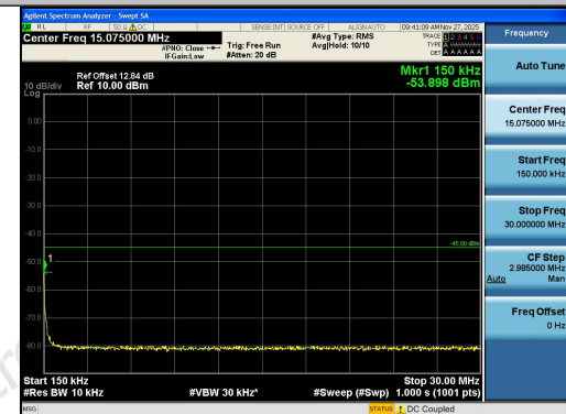
Band41-5MHz-QPSK-41565-1RB#0-0.15~30-PAS S
