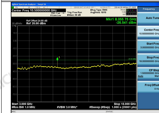
Band41-5MHz-16QAM-41565-1RB#0-3000~1800 0-PASS
