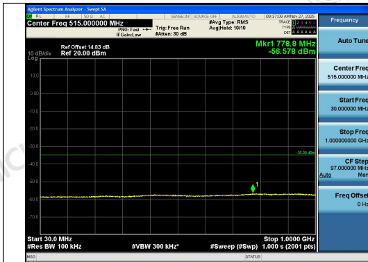
Band41-5MHz-QPSK-40620-25RB#0-30~1000-P ASS
