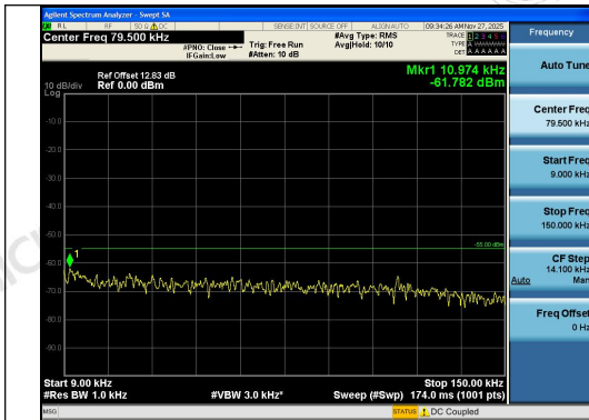
Band41-5MHz-16QAM-40620-1RB#24-0.009~0.1 5-PASS
