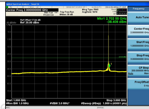
Band41-5MHz-QPSK-41565-1RB#0-1000~3000-P ASS
