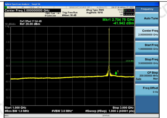
Band41-5MHz-QPSK-40620-25RB#0-1000~3000- PASS
