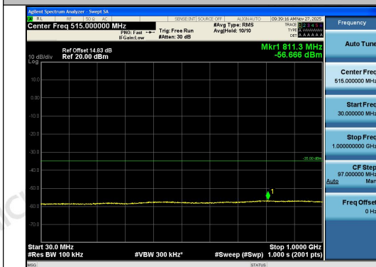
Band41-5MHz-16QAM-40620-25RB#0-30~1000- PASS
