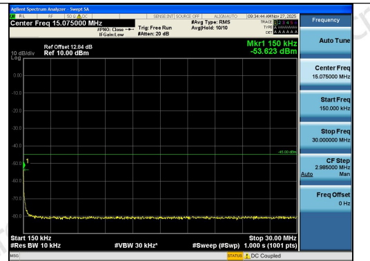
Band41-5MHz-16QAM-40620-1RB#24-0.15~30-P ASS
