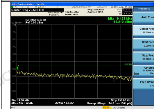
Band41-5MHz-16QAM-40620-25RB#0-0.009~0.1 5-PASS
