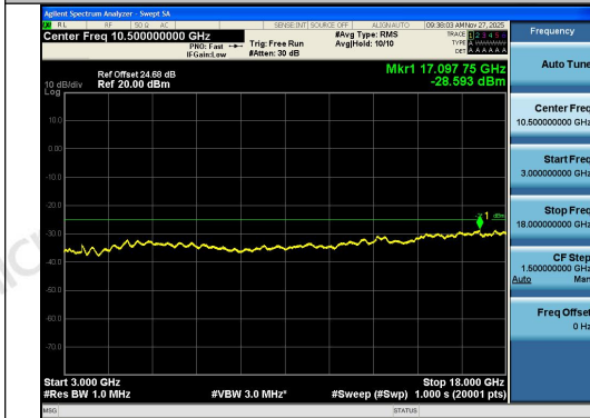
Band41-5MHz-QPSK-40620-25RB#0-3000~1800 0-PASS
