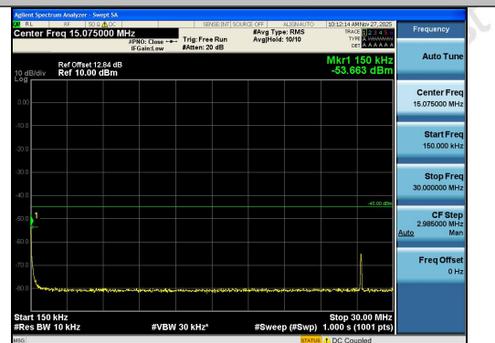
Band41-10MHz-QPSK-40620-1RB#0-0.15~30-PA SS
