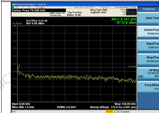
Band41-10MHz-16QAM-40620-1RB#0-0.009~0.1 5-PASS
