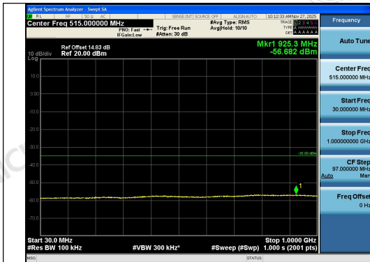
Band41-10MHz-QPSK-40620-1RB#0-30~1000-P ASS
