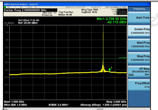
Band41-10MHz-QPSK-40620-1RB#49-1000~3000 -PASS
