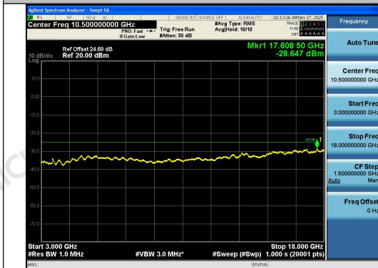
Band41-10MHz-QPSK-40620-1RB#0-3000~1800 0-PASS
