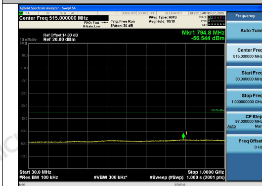
Band41-10MHz-16QAM-41540-1RB#0-30~1000- PASS
