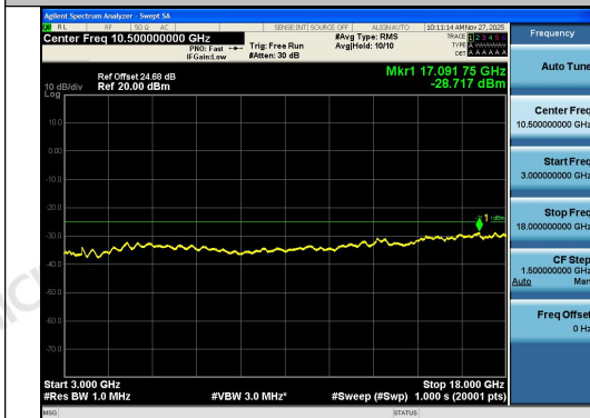
Band41-10MHz-16QAM-39700-1RB#49-3000~18000-PASS 000-PASS
