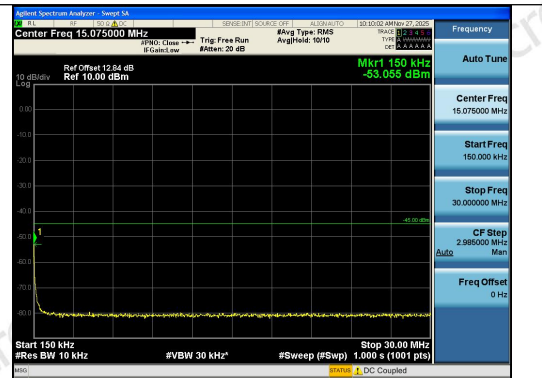
Band41-10MHz-16QAM-39700-1RB#49-0.15~30-P ASS
