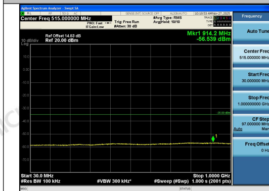
Band41-10MHz-16QAM-40620-1RB#49-30~1000-PASS
