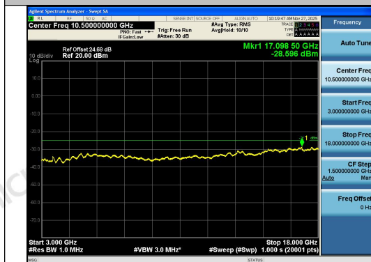
Band41-10MHz-16QAM-40620-1RB#49-3000~18000-PASS
