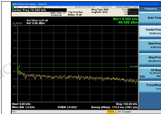
Band41-10MHz-16QAM-39700-1RB#49-0.009~0. 15-PASS
