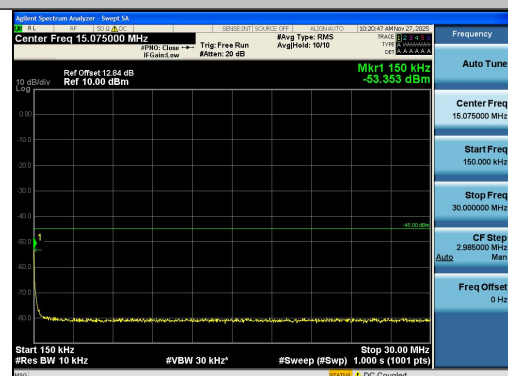
Band41-10MHz-QPSK-41540-1RB#0-0.15~30-PA SS
