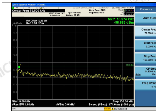
Band41-10MHz-16QAM-40620-1RB#49-0.009~0.15-PASS
