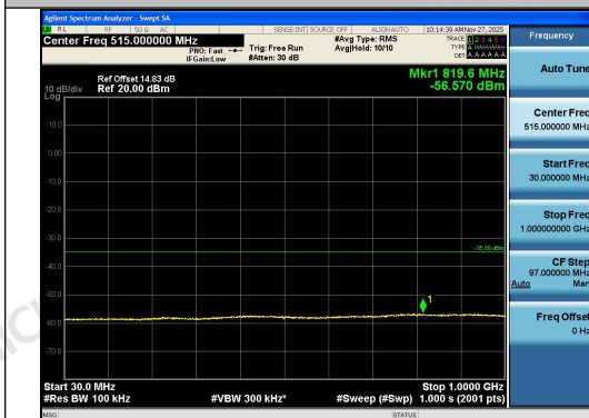
Band41-10MHz-16QAM-40620-1RB#0-30~1000- PASS
