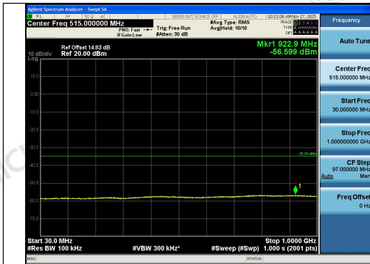
Band41-10MHz-QPSK-41540-1RB#0-30~1000-P ASS
