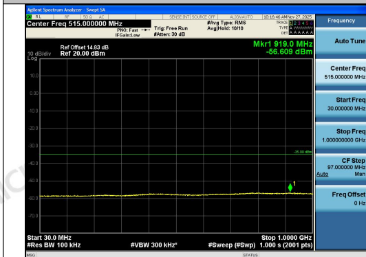
Band41-10MHz-QPSK-40620-1RB#49-30~1000- PASS
