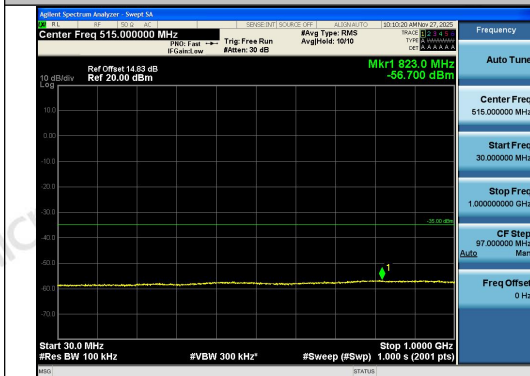
Band41-10MHz-16QAM-39700-1RB#49-30~1000 -PASS
