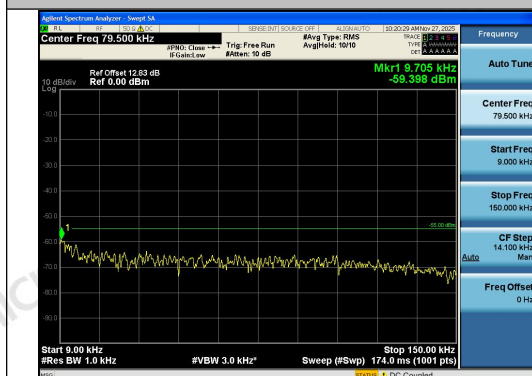
Band41-10MHz-QPSK-41540-1RB#0-0.009~0.15-PASS
