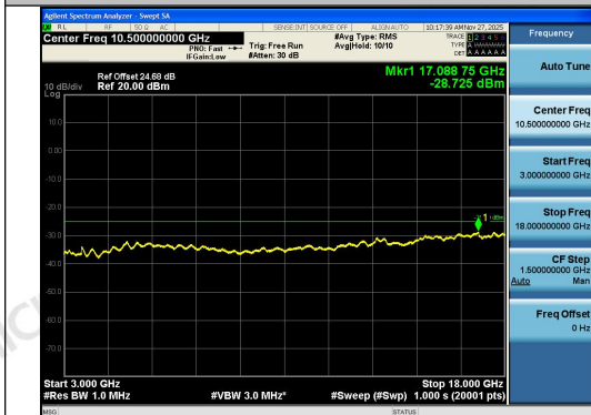
Band41-10MHz-QPSK-40620-1RB#49-3000~180 00-PASS
