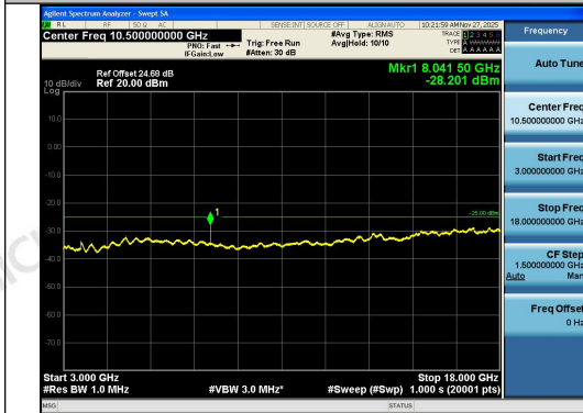
Band41-10MHz-QPSK-41540-1RB#0-3000~1800 0-PASS
