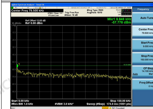
Band41-10MHz-QPSK-40620-1RB#0-0.009~0.15 -PASS
