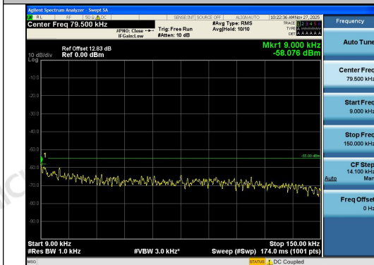
Band41-10MHz-16QAM-41540-1RB#0-0.009~0.1 5-PASS
