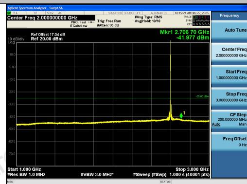
Band41-10MHz-16QAM-40620-1RB#49-1000~3000-PASS
