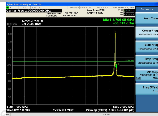
Band41-10MHz-QPSK-41540-50RB#0-1000~3000- PASS
