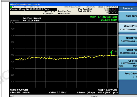
Band41-10MHz-QPSK-41540-1RB#49-3000~180 00-PASS
