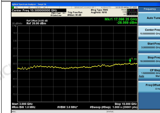
Band41-10MHz-QPSK-39700-50RB#0-3000~180 00-PASS
