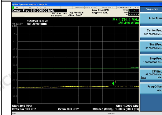
Band41-10MHz-QPSK-41540-50RB#0-30~1000- PASS
