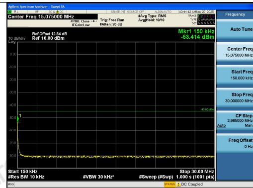
Band41-15MHz-QPSK-39725-1RB#0-0.15~30-PA SS
