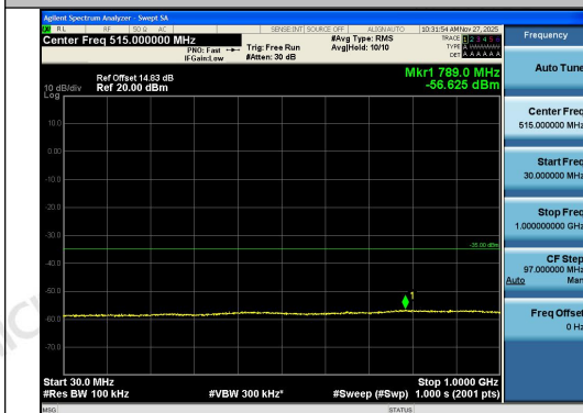
Band41-10MHz-QPSK-40620-50RB#0-30~1000- PASS
