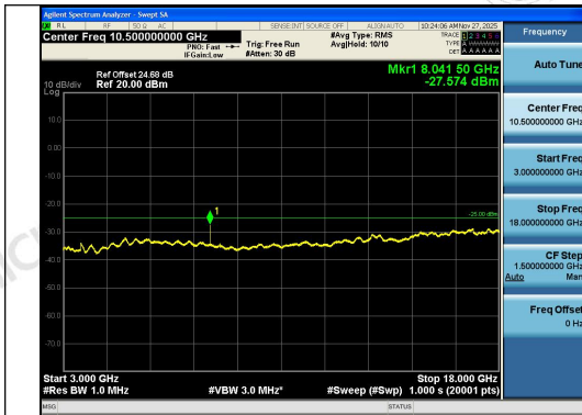
Band41-10MHz-16QAM-41540-1RB#0-3000~180 00-PASS
