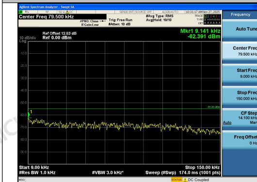
Band41-10MHz-QPSK-40620-50RB#0-0.009~0.1 5-PASS
