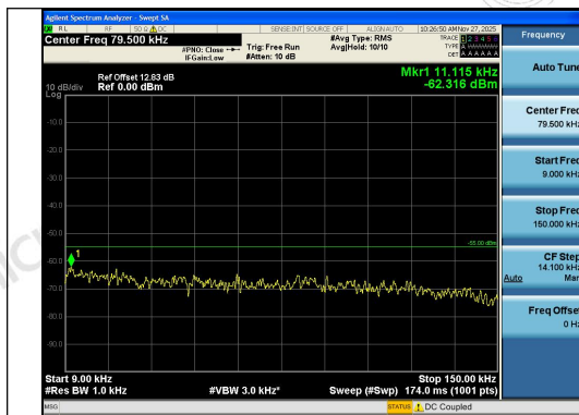
Band41-10MHz-16QAM-41540-1RB#49-0.009~0.15-PASS
