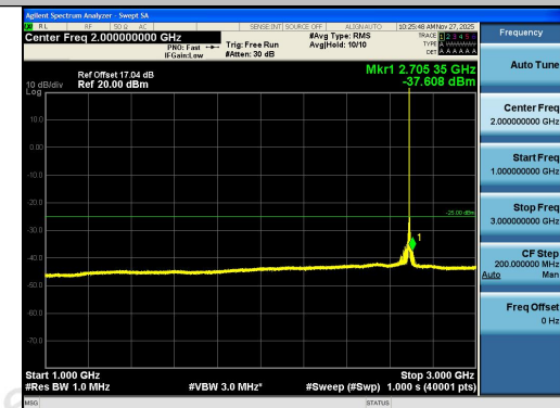
Band41-10MHz-QPSK-41540-1RB#49-1000~3000-PASS
