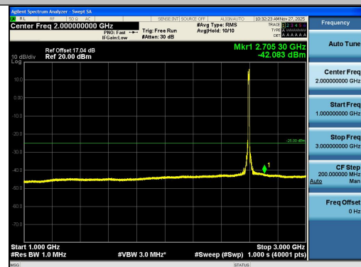
Band41-10MHz-QPSK-40620-50RB#0-1000~3000 -PASS
