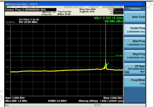
Band41-10MHz-16QAM-41540-1RB#49-1000~3000-PASS
