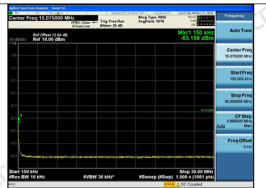
Band41-10MHz-16QAM-41540-1RB#49-0.15~30-P ASS
