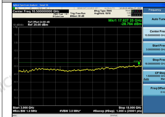
Band41-10MHz-16QAM-41540-1RB#49-3000~18000-PASS
