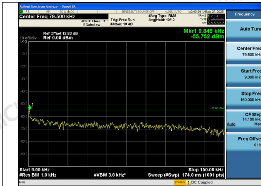
Band41-15MHz-QPSK-39725-1RB#0-0.009~0.15 -PASS
