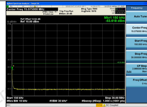
Band41-10MHz-QPSK-41540-1RB#49-0.15~30-PA SS
