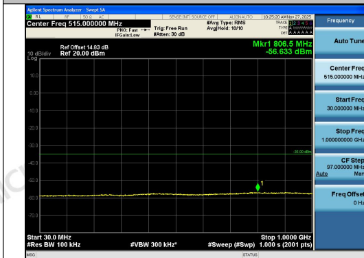
Band41-10MHz-QPSK-41540-1RB#49-30~1000-PASS
