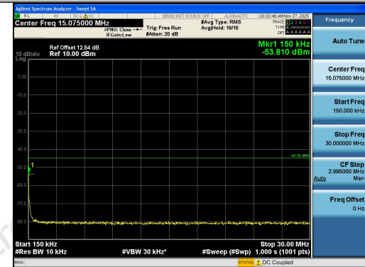
Band41-10MHz-QPSK-41540-50RB#0-0.15~30-PA SS
