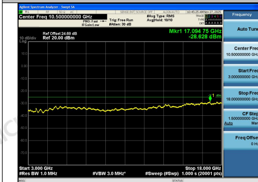
Band41-15MHz-QPSK-39725-1RB#0-3000~1800 0-PASS
