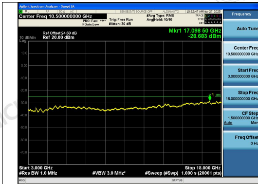
Band41-10MHz-QPSK-40620-50RB#0-3000~180 00-PASS
