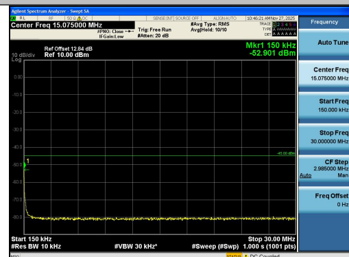
Band41-15MHz-16QAM-39725-1RB#0-0.15~30-P ASS
