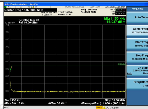
Band41-10MHz-QPSK-40620-50RB#0-0.15~30-PA SS
