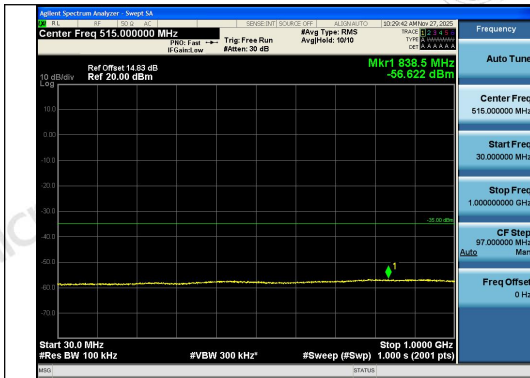
Band41-10MHz-QPSK-39700-50RB#0-30~1000- PASS
