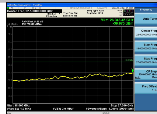
Band41-10MHz-QPSK-41540-1RB#49-18000~270 00-PASS
