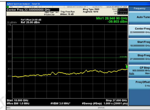
Band41-10MHz-16QAM-41540-1RB#0-18000~270 00-PASS
