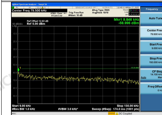
Band41-15MHz-QPSK-39725-1RB#74-0.009~0.1- 5-PASS
