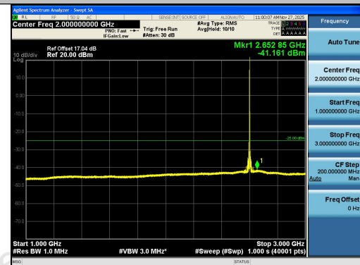
Band41-15MHz-16QAM-40620-1RB#74-1000~300 0-PASS
