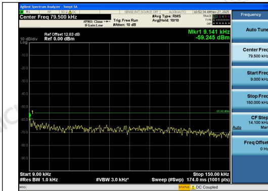
Band41-15MHz-QPSK-40620-1RB#0-0.009~0.15 -PASS
