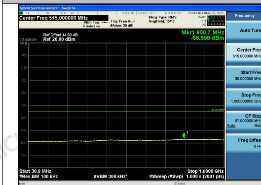
Band41-15MHz-QPSK-39725-1RB#74-30~1000- PASS
