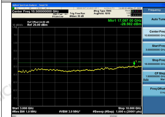
Band41-15MHz-16QAM-40620-1RB#74-3000~18 000-PASS
