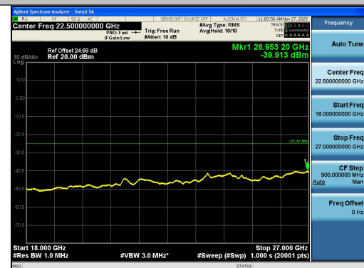
Band41-15MHz-16QAM-40620-1RB#74-18000~27 000-PASS
