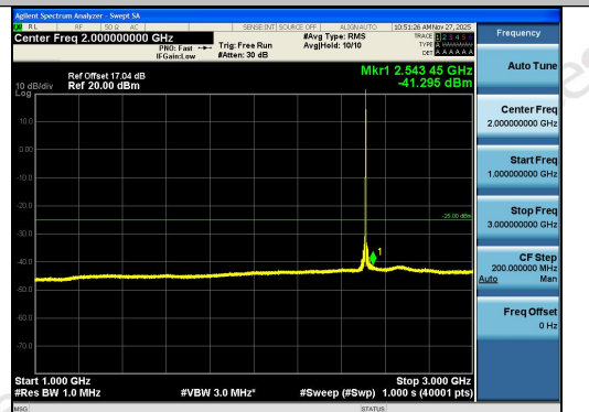
Band41-15MHz-16QAM-39725-1RB#74-1000~300 0-PASS
