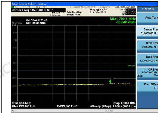
Band41-15MHz-16QAM-40620-1RB#0-30~1000- PASS
