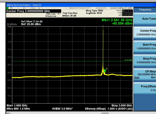
Band41-15MHz-QPSK-39725-1RB#74-1000~3000- -PASS
