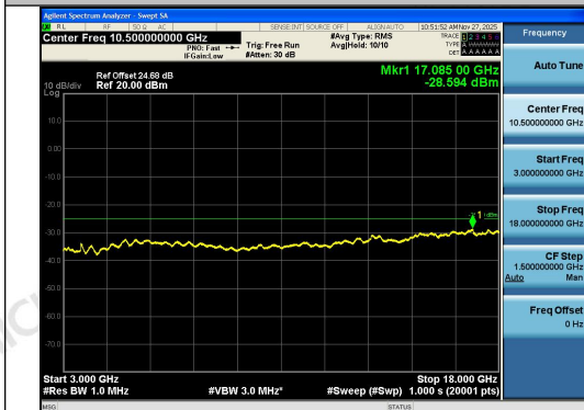
Band41-15MHz-16QAM-39725-1RB#74-3000~18 000-PASS
