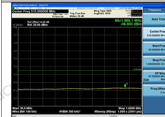
Band41-15MHz-QPSK-40620-1RB#74-30~1000- PASS
