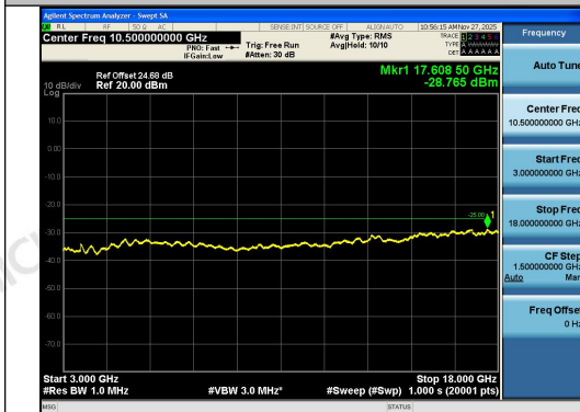
Band41-15MHz-16QAM-40620-1RB#0-3000~18000- 00-PASS
