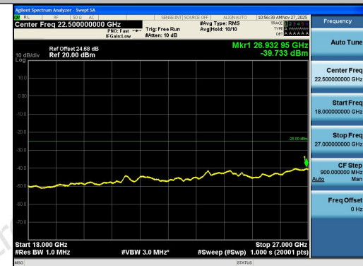
Band41-15MHz-16QAM-40620-1RB#0-18000~27000- 00-PASS
