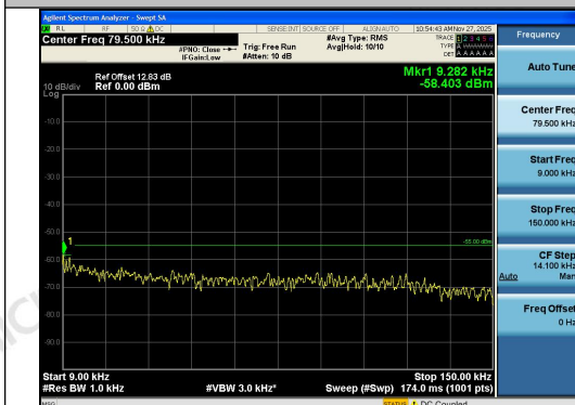
Band41-15MHz-16QAM-40620-1RB#0-0.009~0.1 5-PASS
