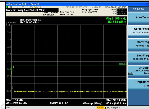
Band41-15MHz-QPSK-39725-1RB#74-0.15~30-PA- SS
