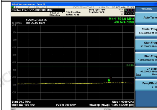
Band41-15MHz-16QAM-39725-1RB#74-30~1000 -PASS
