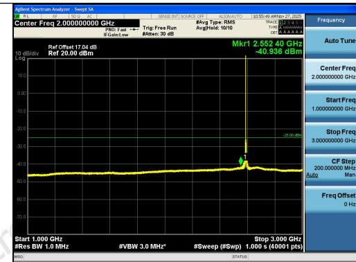
Band41-15MHz-16QAM-40620-1RB#0-1000~3000- -PASS
