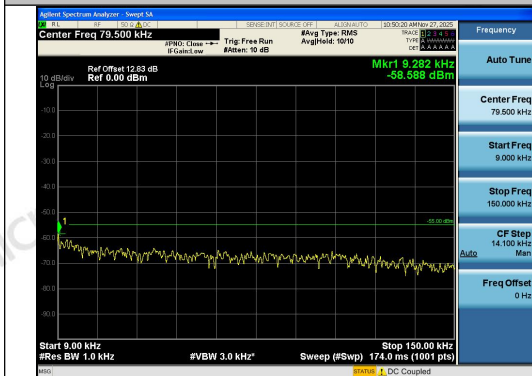
Band41-15MHz-16QAM-39725-1RB#74-0.009~0. 15-PASS
