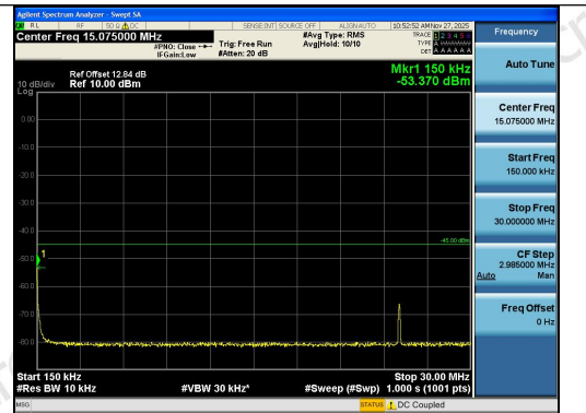
Band41-15MHz-QPSK-40620-1RB#0-0.15~30-PA SS
