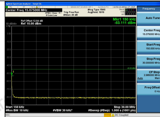
Band41-15MHz-16QAM-40620-1RB#74-0.15~30-P ASS
