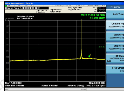
Band41-15MHz-16QAM-39725-1RB#0-1000~3000- -PASS
