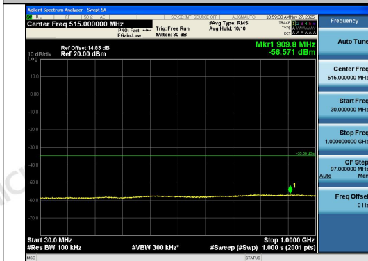
Band41-15MHz-16QAM-40620-1RB#74-30~1000 -PASS
