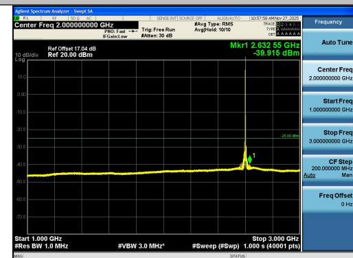
Band41-15MHz-QPSK-40620-1RB#74-1000~3000- -PASS
