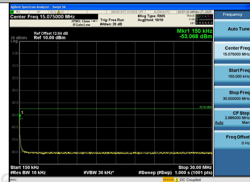
Band41-15MHz-QPSK-40620-1RB#74-0.15~30-PA- SS
