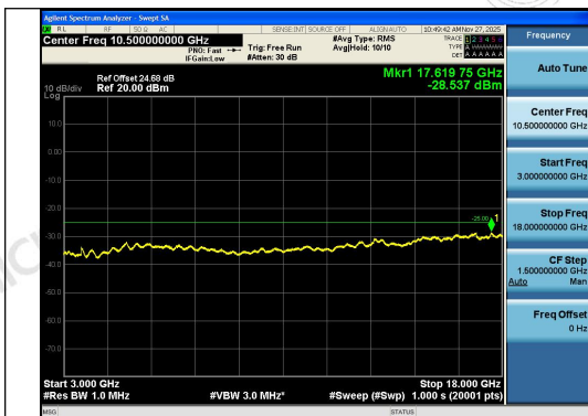
Band41-15MHz-QPSK-39725-1RB#74-3000~180 00-PASS
