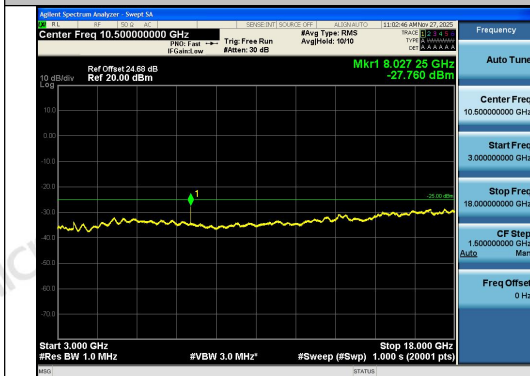
Band41-15MHz-QPSK-41515-1RB#0-3000~1800 0-PASS
