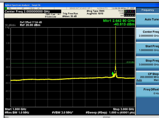
Band41-15MHz-QPSK-41515-1RB#74-1000~3000 -PASS
