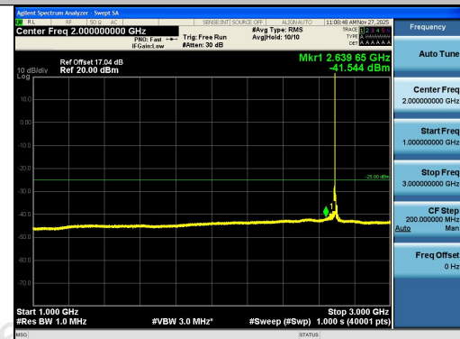
Band41-15MHz-16QAM-41515-1RB#74-1000~300 0-PASS
