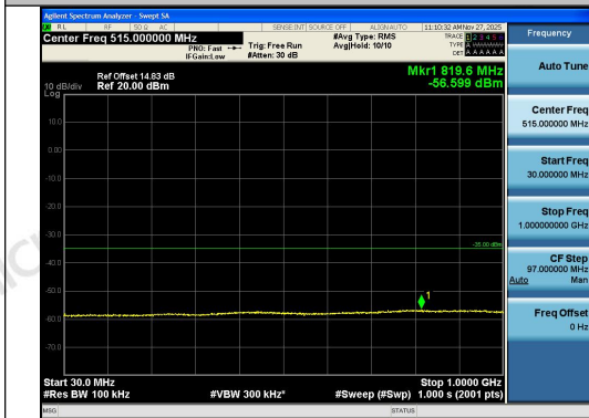
Band41-15MHz-QPSK-39725-75RB#0-30~1000- PASS
