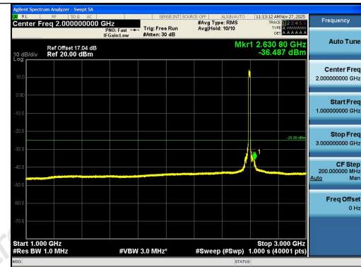
Band41-15MHz-QPSK-40620-75RB#0-1000~3000 -PASS
