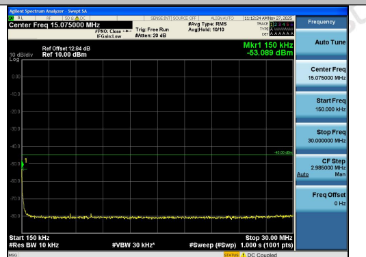
Band41-15MHz-QPSK-40620-75RB#0-0.15~30-PA SS
