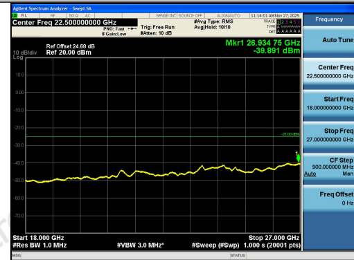
Band41-15MHz-QPSK-40620-75RB#0-18000~270 00-PASS
