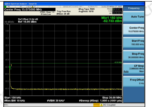
Band41-15MHz-QPSK-41515-1RB#0-0.15~30-PA SS
