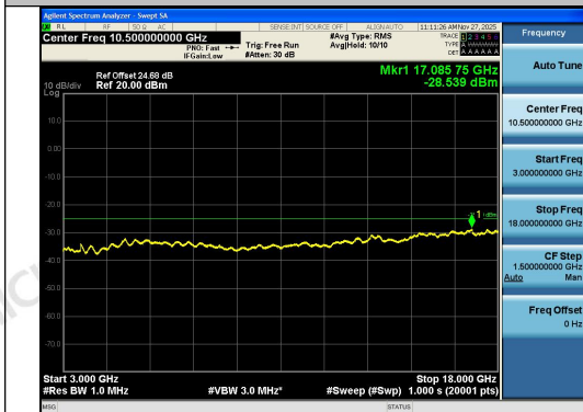
Band41-15MHz-QPSK-39725-75RB#0-3000~18000- 00-PASS
