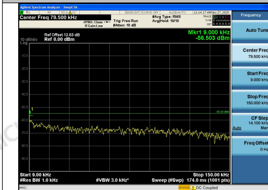
Band41-15MHz-QPSK-41515-75RB#0-0.009~0.1 5-PASS
