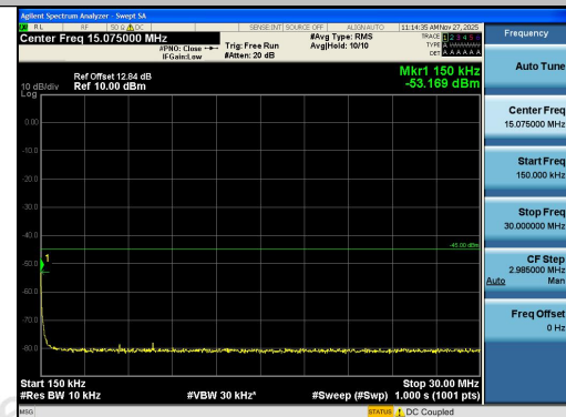
Band41-15MHz-QPSK-41515-75RB#0-0.15~30-PA SS
