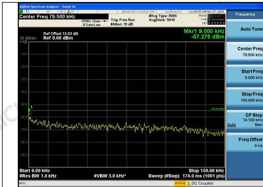
Band41-15MHz-QPSK-39725-75RB#0-0.009~0.1 5-PASS
