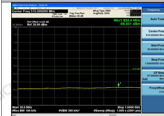
Band41-15MHz-QPSK-41515-75RB#0-30~1000- PASS
