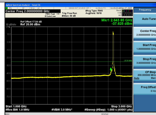
Band41-15MHz-QPSK-41515-75RB#0-1000~3000 -PASS
