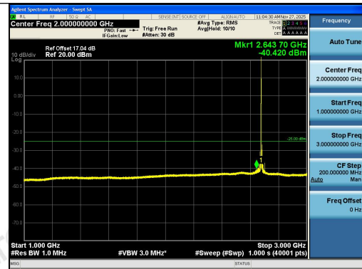
Band41-15MHz-16QAM-41515-1RB#0-1000~3000 -PASS
