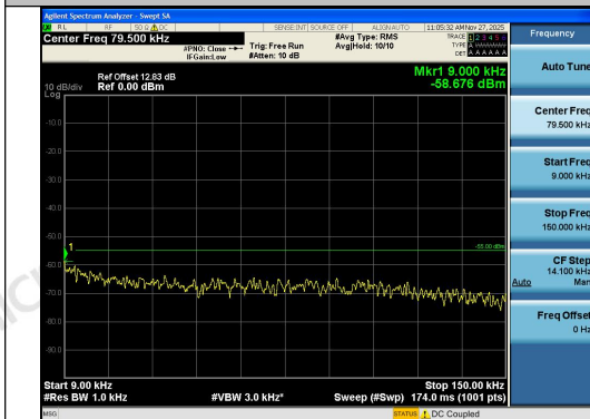
Band41-15MHz-QPSK-41515-1RB#74-0.009~0.1 5-PASS
