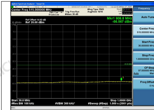
Band41-15MHz-QPSK-40620-75RB#0-30~1000- PASS
