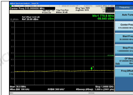
Band41-15MHz-16QAM-41515-1RB#0-30~1000- PASS
