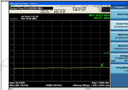
Band41-15MHz-16QAM-41515-1RB#74-30~1000 -PASS
