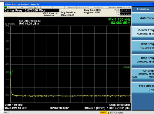
Band41-15MHz-QPSK-41515-1RB#74-0.15~30-PA SS
