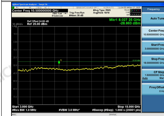
Band41-15MHz-16QAM-41515-1RB#0-3000~180 00-PASS
