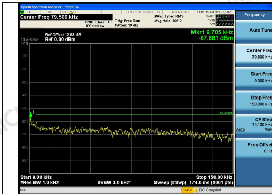
Band41-15MHz-QPSK-41515-1RB#0-0.009~0.15 -PASS
