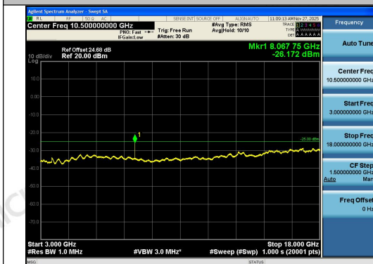
Band41-15MHz-16QAM-41515-1RB#74-3000~18 000-PASS
