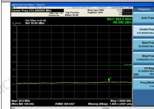
Band41-15MHz-QPSK-41515-1RB#74-30~1000- PASS
