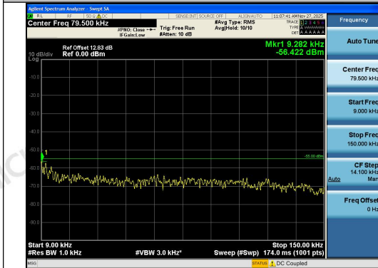
Band41-15MHz-16QAM-41515-1RB#74-0.009~0. 15-PASS
