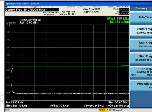
Band41-15MHz-16QAM-41515-1RB#74-0.15~30-P ASS
