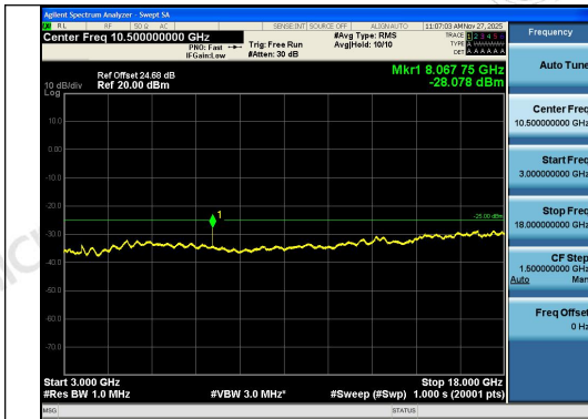
Band41-15MHz-QPSK-41515-1RB#74-3000~180 00-PASS
