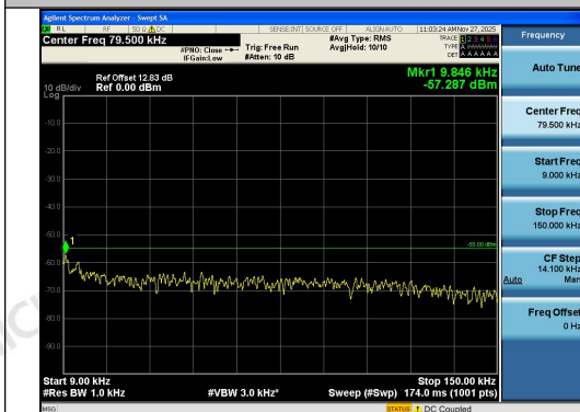
Band41-15MHz-16QAM-41515-1RB#0-0.009~0.1 5-PASS
