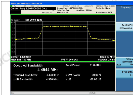
Band2-5MHz-QPSK-19175-25RB#0-PASS
