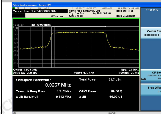
Band2-10MHz-QPSK-19150-50RB#0-PASS
