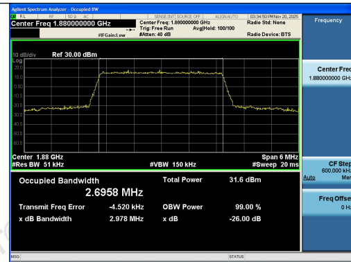
Band2-3MHz-16QAM-18900-15RB#0-PASS
