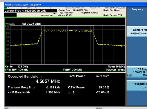
Band2-5MHz-16QAM-18625-25RB#0-PASS
