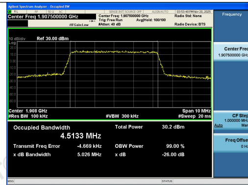
Band2-5MHz-16QAM-19175-25RB#0-PASS
