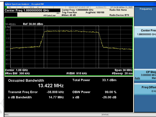
Band2-15MHz-QPSK-18900-75RB#0-PASS
