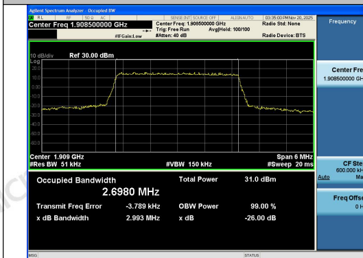
Band2-3MHz-QPSK-19185-15RB#0-PASS
