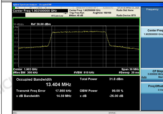
Band2-15MHz-QPSK-19125-75RB#0-PASS
