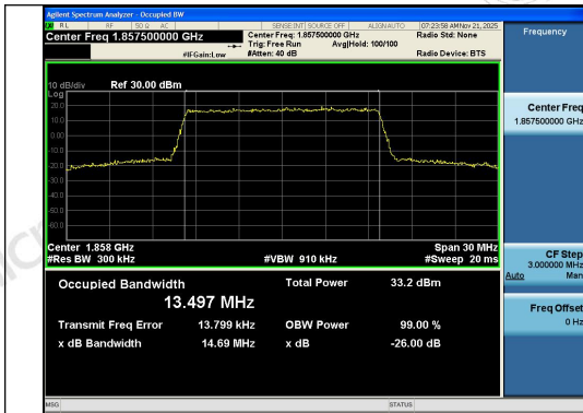
Band2-15MHz-QPSK-18675-75RB#0-PASS
