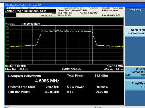
Band2-5MHz-16QAM-18900-25RB#0-PASS
