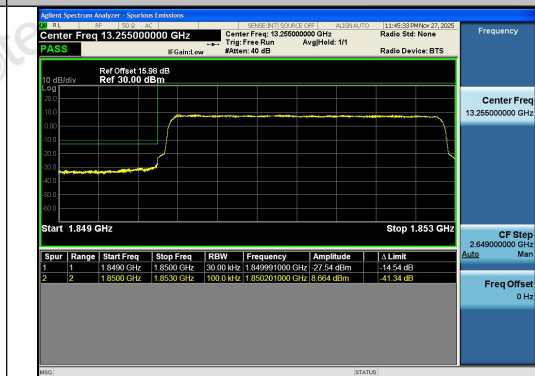
Band2-3MHz-16QAM-18615-15RB#0-PASS
