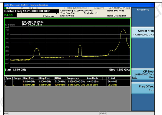
Band2-5MHz-16QAM-18625-1RB#24-PASS
