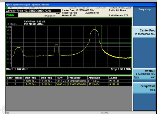
Band2-3MHz-16QAM-19185-1RB#14-PASS
