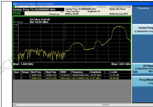
Band2-1.4MHz-QPSK-18607-1RB#5-PASS
