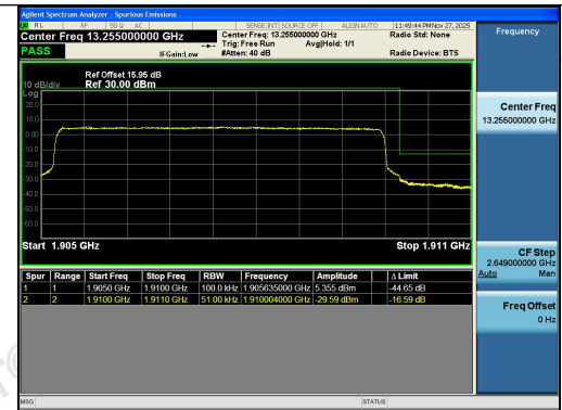
Band2-5MHz-16QAM-19175-25RB#0-PASS
