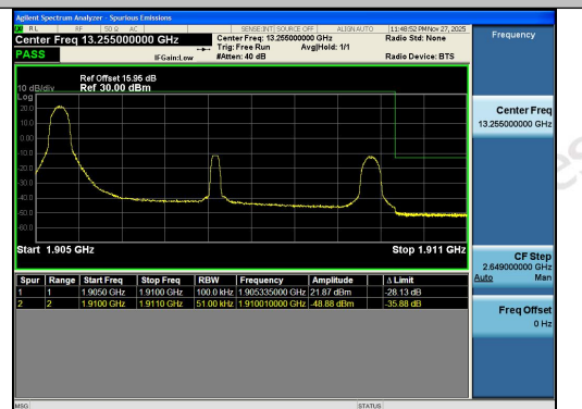
Band2-5MHz-16QAM-19175-1RB#0-PASS
