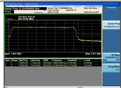
Band2-3MHz-16QAM-19185-15RB#0-PASS
