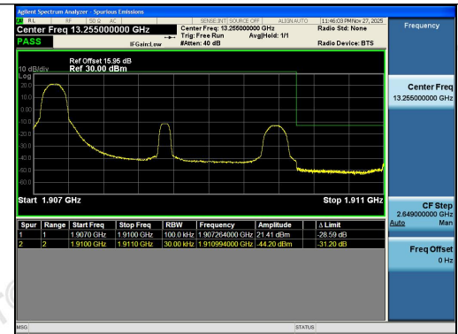
Band2-3MHz-16QAM-19185-1RB#0-PASS
