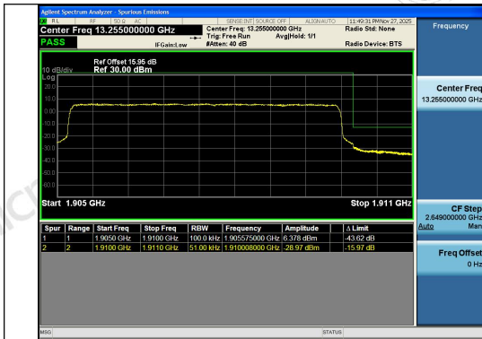
Band2-5MHz-QPSK-19175-25RB#0-PASS
