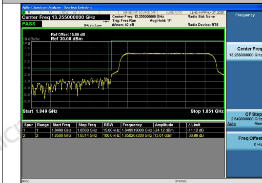
Band2-1.4MHz-QPSK-18607-6RB#0-PASS
