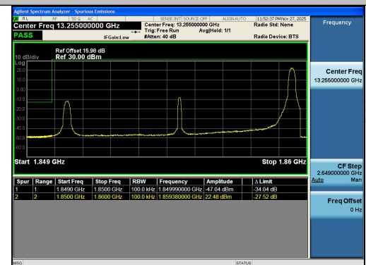
Band2-10MHz-16QAM-18650-1RB#49-PASS
