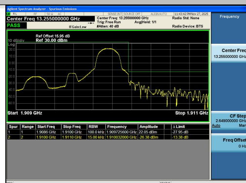
Band2-1.4MHz-16QAM-19193-1RB#5-PASS
