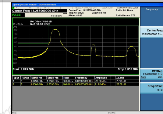
Band2-3MHz-16QAM-18615-1RB#0-PASS
