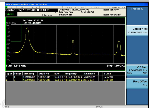
Band2-10MHz-16QAM-18650-1RB#0-PASS
