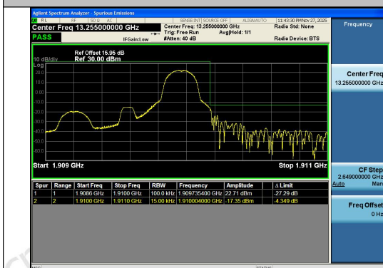
Band2-1.4MHz-QPSK-19193-1RB#5-PASS
