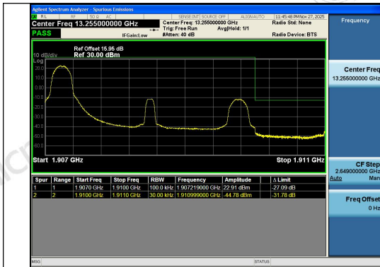
Band2-3MHz-QPSK-19185-1RB#0-PASS
