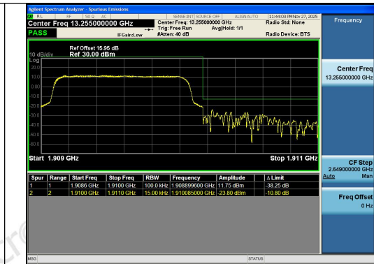
Band2-1.4MHz-16QAM-19193-6RB#0-PASS
