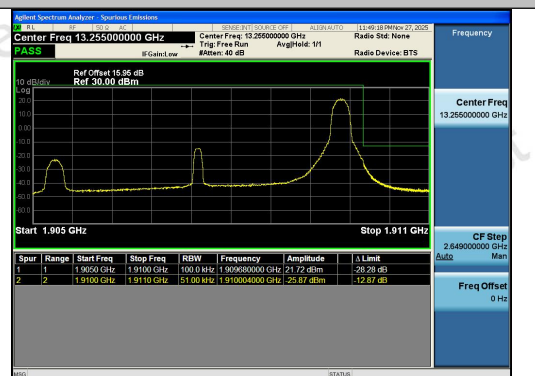
Band2-5MHz-16QAM-19175-1RB#24-PASS
