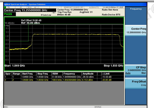
Band2-5MHz-16QAM-18625-25RB#0-PASS
