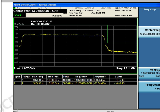
Band2-3MHz-QPSK-19185-15RB#0-PASS
