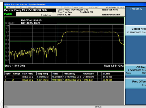
Band2-1.4MHz-16QAM-18607-6RB#0-PASS
