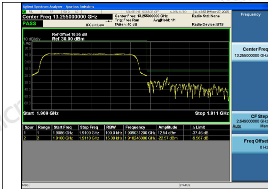
Band2-1.4MHz-QPSK-19193-6RB#0-PASS
