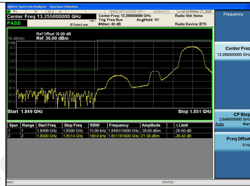
Band2-1.4MHz-16QAM-18607-1RB#5-PASS
