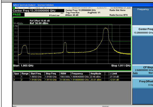
Band2-5MHz-QPSK-19175-1RB#24-PASS
