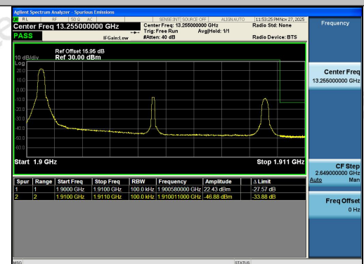
Band2-10MHz-16QAM-19150-1RB#0-PASS
