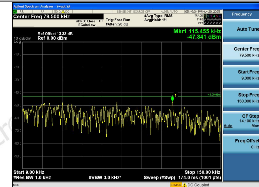
Band2-1.4MHz-16QAM-18607-1RB#5-0.009~0.15
