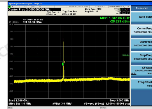
Band2-1.4MHz-16QAM-18607-1RB#5-1000~3000
