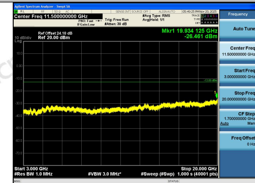
Band2-1.4MHz-QPSK-18607-1RB#5-3000~20000
