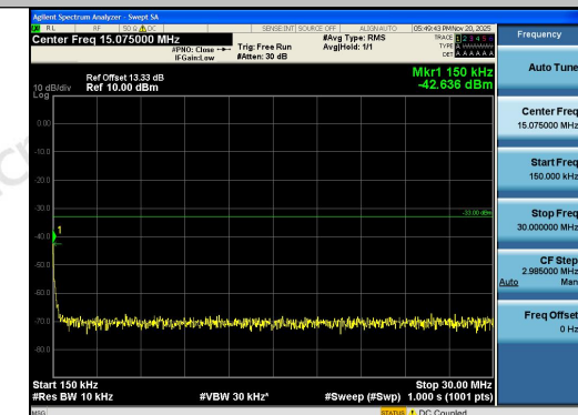
Band2-1.4MHz-16QAM-18607-1RB#5-0.15~30-PA
