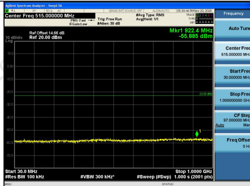
Band2-1.4MHz-QPSK-19193-1RB#0-30~1000-PA
