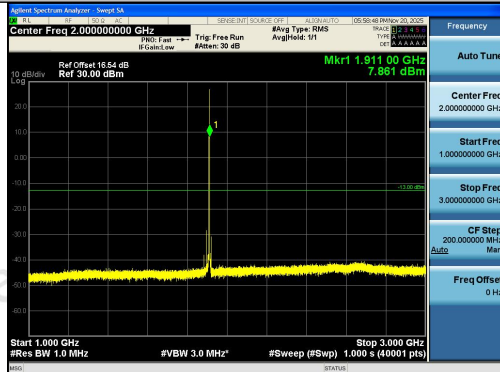
Band2-1.4MHz-QPSK-19193-1RB#5-1000~3000-
