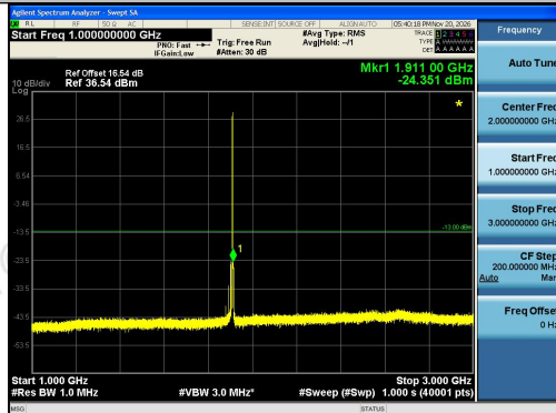
Band2-1.4MHz-QPSK-19193-1RB#0-1000~3000-
