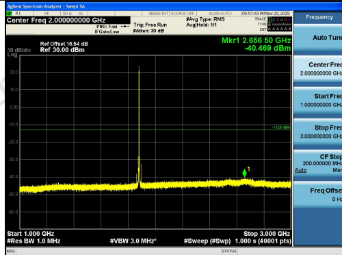
Band2-1.4MHz-16QAM-18900-6RB#0-1000~3000
