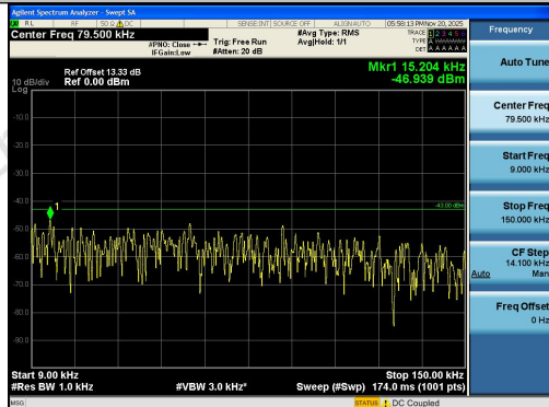
Band2-1.4MHz-QPSK-19193-1RB#5-0.009~0.15-
