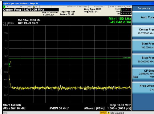
Band2-1.4MHz-QPSK-19193-1RB#5-0.15~30-PA
