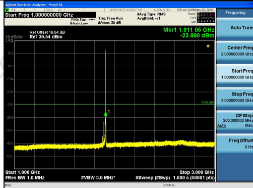
Band2-1.4MHz-16QAM-19193-1RB#0-1000~3000
