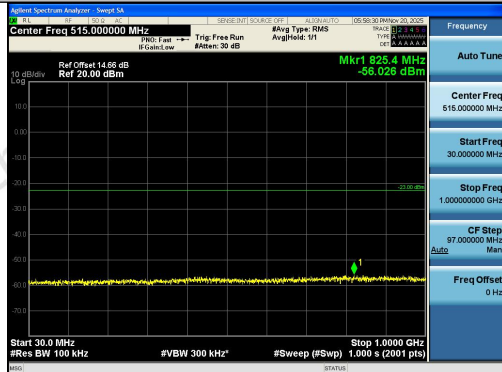
Band2-1.4MHz-QPSK-19193-1RB#5-30~1000-PA
