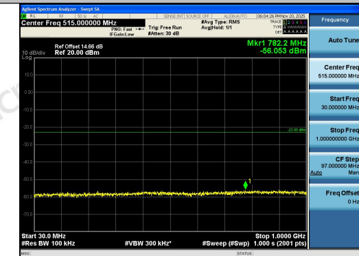
Band2-3MHz-16QAM-18615-1RB#0-30~1000-PA
