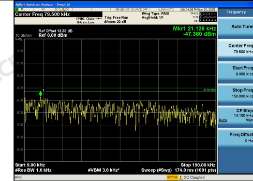
Band2-3MHz-16QAM-18615-1RB#0-0.009~0.15-P
