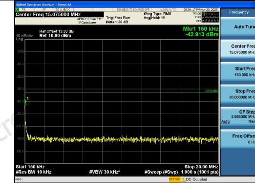
Band2-3MHz-16QAM-18615-1RB#0-0.15~30-PAS
