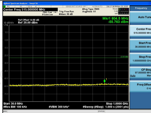
Band2-3MHz-16QAM-19185-1RB#0-30~1000-PA
