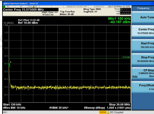
Band2-3MHz-16QAM-19185-1RB#0-0.15~30-PAS
