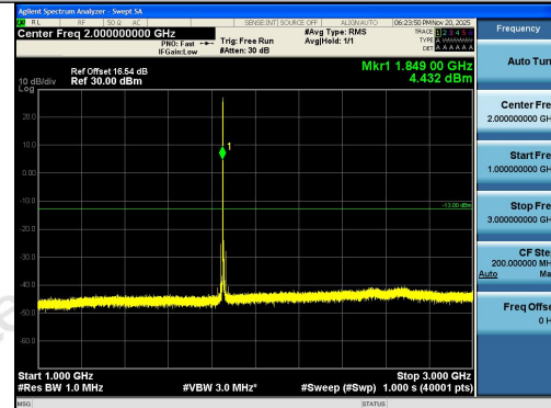
Band2-5MHz-QPSK-18625-1RB#0-1000~3000-PA
