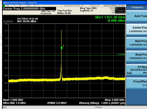
Band2-3MHz-16QAM-19185-15RB#0-1000~3000-PASS
