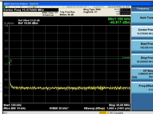
Band2-3MHz-QPSK-19185-1RB#14-0.15~30-PAS
