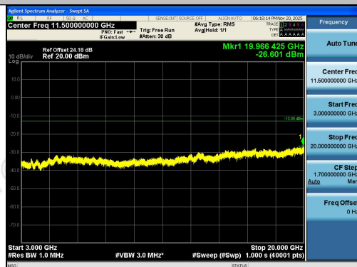
Band2-3MHz-16QAM-19185-1RB#0-3000~20000-PASS
