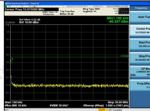
Band2-5MHz-QPSK-18625-1RB#0-0.15~30-PASS
