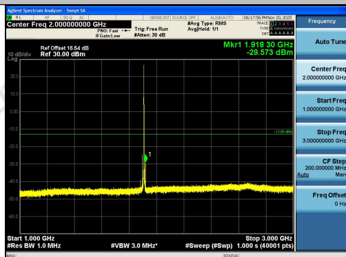
Band2-3MHz-16QAM-19185-1RB#0-1000~3000-P
