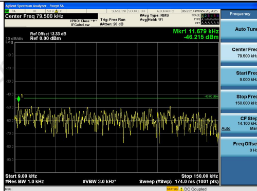
Band2-5MHz-QPSK-18625-1RB#0-0.009~0.15-PA
